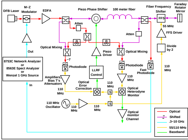
Figure 2: (color) Stabilized Transport with RF Test Signal
