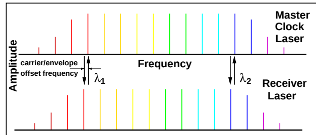
Figure 3: (color) Matching of comb spectra from two modelocked lasers.
