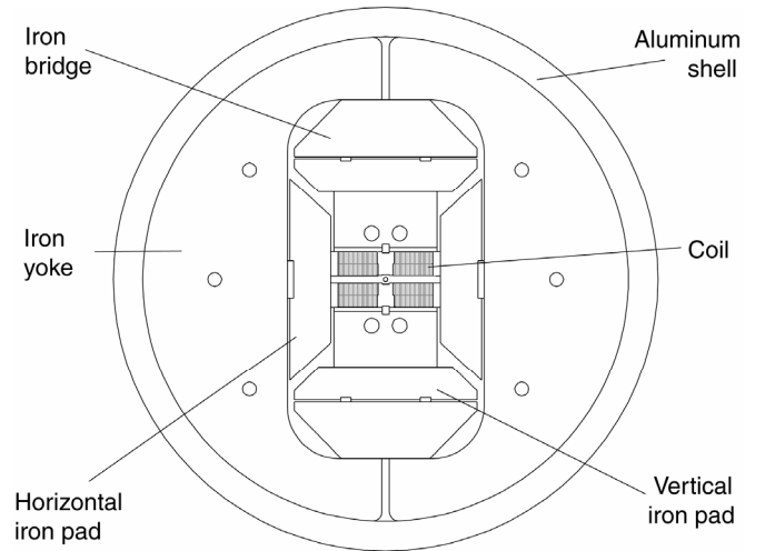
Figure 1: HD1 magnet cross-section. The outer diameter of the shell is 74 cm.
