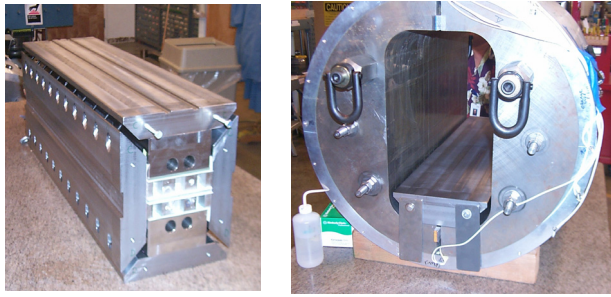
Figure 4: Assembled coil-pack (left) and shell and loading structure (right).
