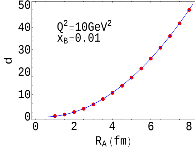
FIG. 4. The R_A dependence of heavy quark energy loss for a charm quark.
