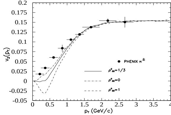
FIG. 2: Azimuthal anisotropy v_2 of final produced pions that include both directly produced and these from the decay of \rho vector mesons that have spin alignment according to Eq. (13) with \rho_{00}^0 = 1/3 (solid line), 0 (dot-dashed line) and 1 (dashed line). The multiplicity ratio \rho/\pi = 0.183 [24] is assumed. The data are for pions from PHENIX experiment [23].
