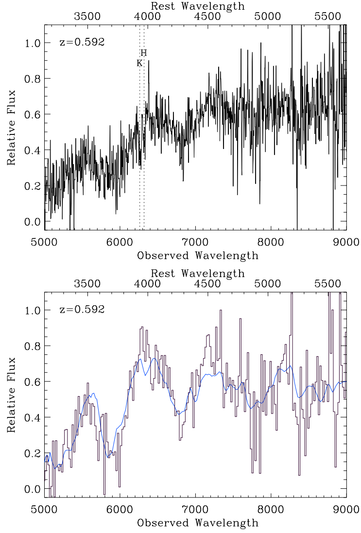
Fig. 12.— (Upper) Lightly smoothed spectrum of SN 1997ag showing narrow features used to determine the redshift. (Lower) rebinned spectrum SN 1997ag (histogram) after interpolating over narrow galaxy lines, compared with the Type Ia SN 1990N at +7 days before maximum (smooth curve).
