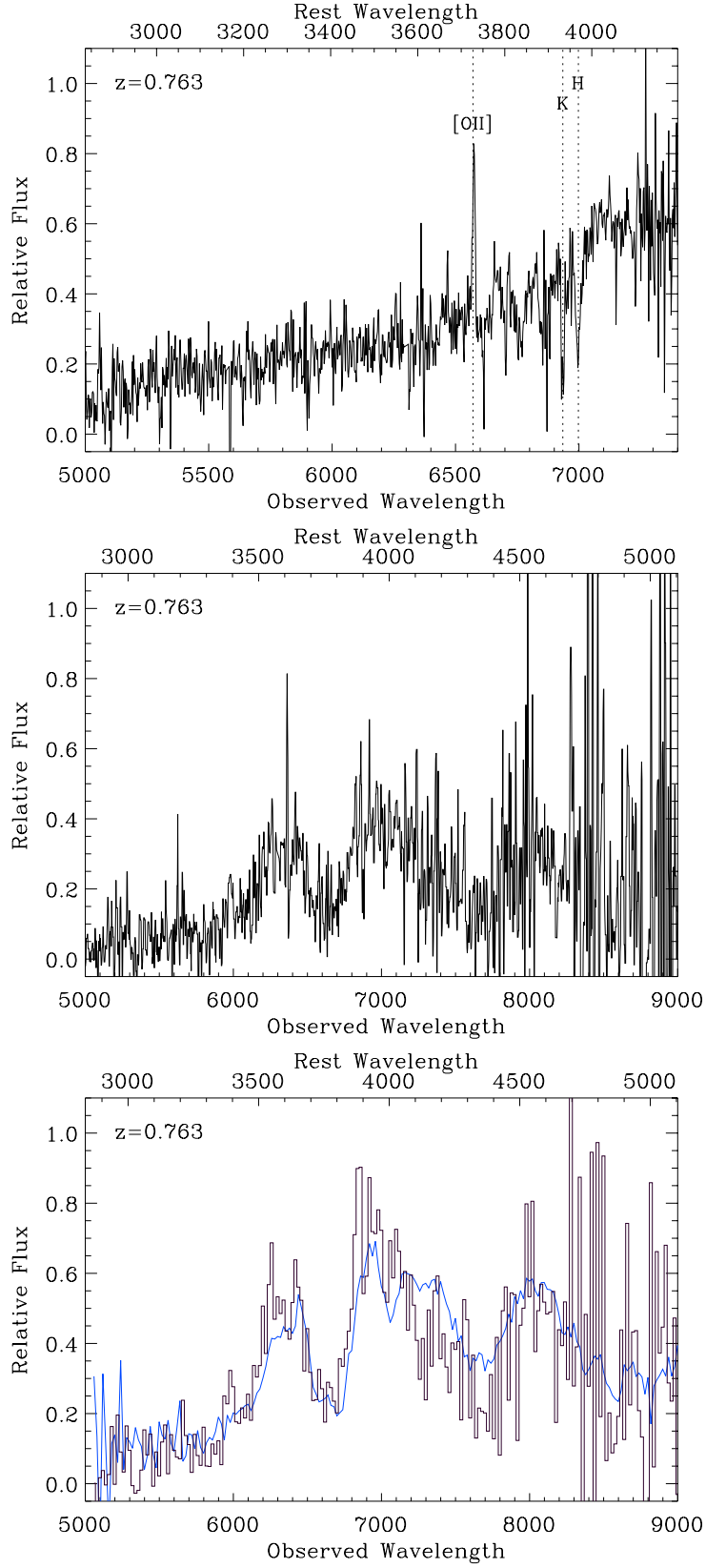
Fig. 4.— (Upper) Lightly smoothed spectrum of neighbouring (host) galaxy of SN 1997G (note that atmospheric absorption has not been corrected in this spectrum). (Lower) Lightly smoothed spectrum of the supernova SN 1997G (lower) rebinned spectrum of SN 1997G (histogram) after interpolating over poorly-subtracted sky lines and subtracting an Sa galaxy template, compared with SN 1999bk at +4 days (smooth curve).
