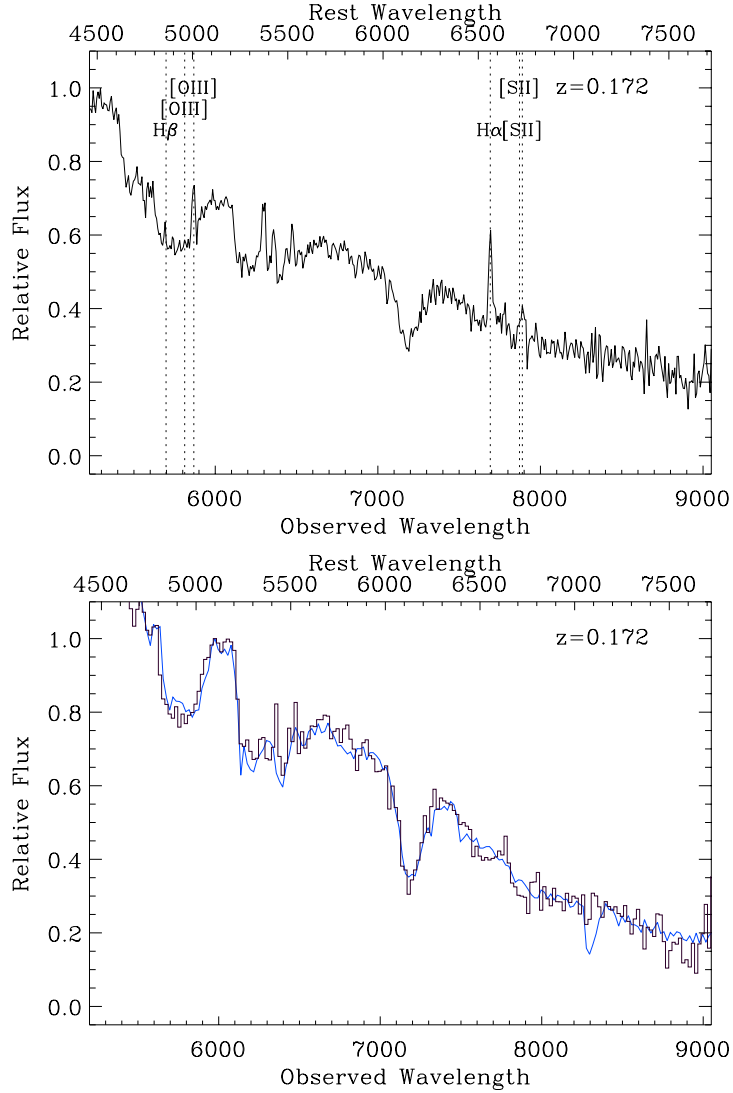
Fig. 5.— (Upper) Unsmoothed spectrum of SN 1997I obtained at the ESO 3.6m showing galaxy lines used to determine the redshift. (Lower) Rebinned spectrum of SN 1997I (histogram) after interpolating over narrow galaxy lines and subtraction of an Sb template galaxy spectrum, compared with SN 1999bp at +1 day (smooth curve).
