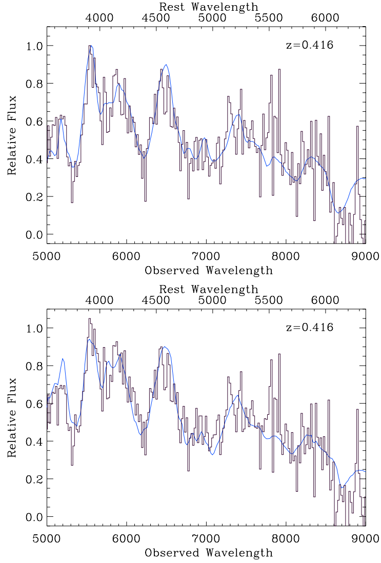
Fig. 15.— cont. (Upper) Rebinned spectrum of SN 1997am (histogram) after interpolating across cosmic rays and narrow lines from the host galaxy and subtraction of a SB1 galaxy template, compared with the Type Ia SN 1992A at +9 days (smooth curve). (Lower) previous plot but with the Type Ia SN 1991T at +10 days for comparison.
