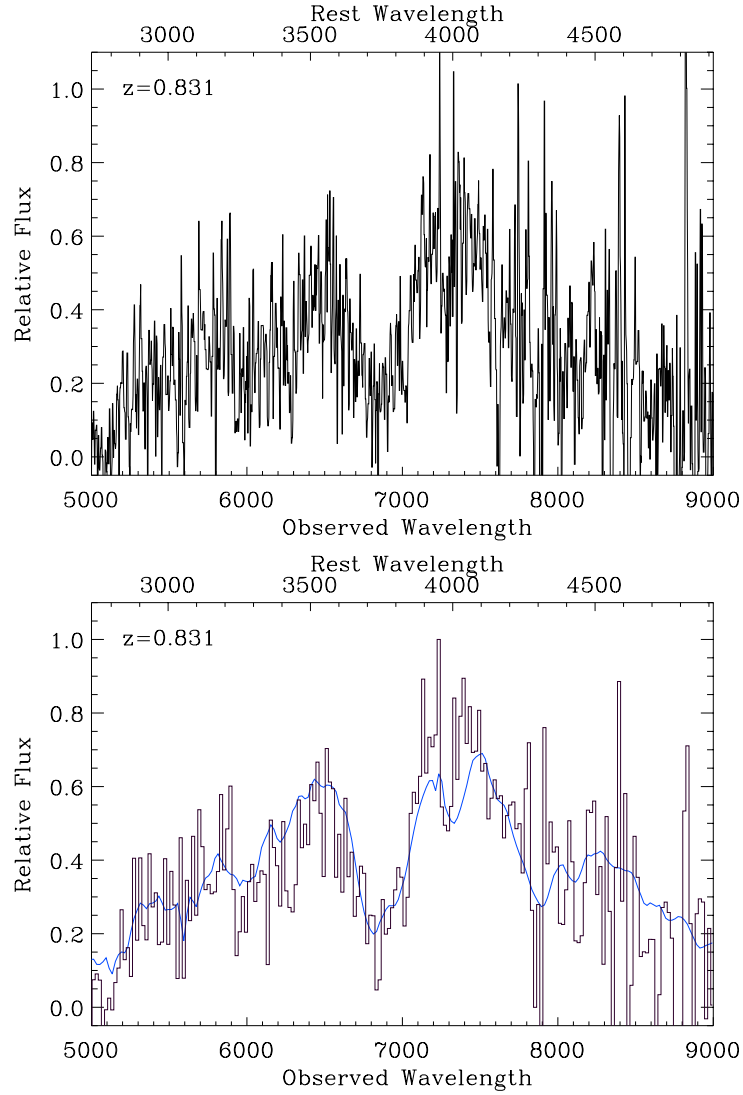
Fig. 16.— (Upper) Lightly smoothed spectrum of SN 1997ap. (Lower) Rebinned spectrum of SN 1997ap (histogram) after interpolating across the sky absorption region at 7600\text{\AA} compared with the Type Ia SN 1989B at -5 days (smooth curve).
