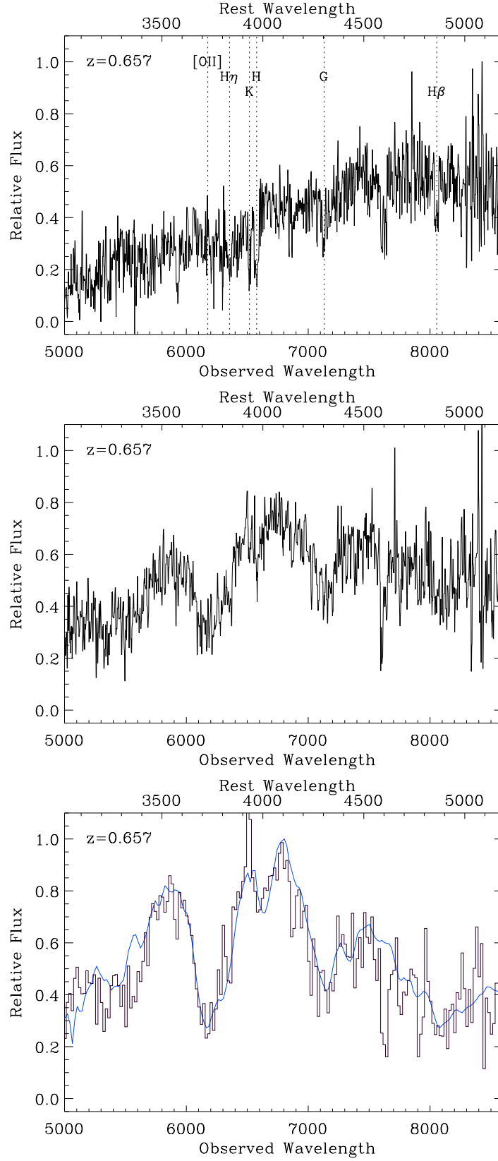
Fig. 8.— (Upper) Lightly smoothed spectrum of the host (or possible neighbour) galaxy of SN 1997R (atmospheric absorption has not been corrected in this spectrum). (Middle) Lightly smoothed spectrum of SN 1997R. (Lower) Rebinned spectrum of SN 1997R (histogram) after interpolating over narrow host galaxy lines, rebinning to 20Å and subtracting template Sa galaxy, compared with SN 1989B at -5 days (smooth curve).
