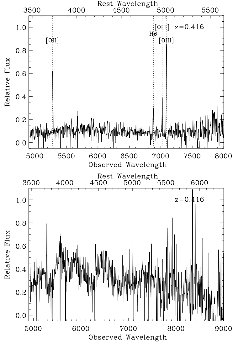
Fig. 15.— (Upper) Unsmoothed spectrum of the host of SN 1997am showing the narrow lines used to determine the redshift. (Lower) lightly smoothed spectrum of SN 1997am.
