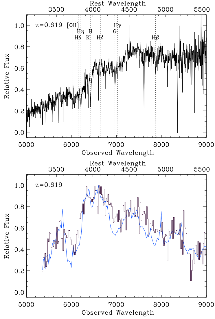
Fig. 6.— (Upper) Unsmoothed spectrum of SN 1997J showing the narrow lines used to determine the redshift. (Lower) rebinned spectrum of SN 1997J (histogram) after subtraction of template S0 host galaxy, compared with SN 1999bn at day +2 (smooth curve).
