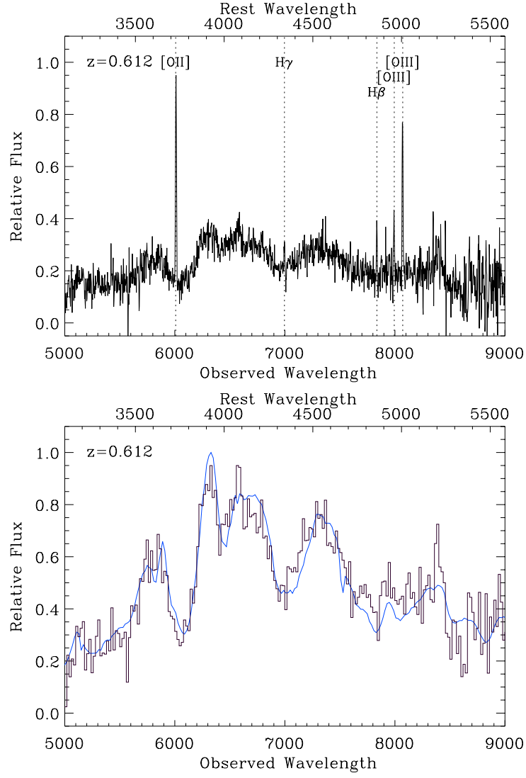
Fig. 9.— (Upper) Unsmoothed spectrum of SN 1997S showing the narrow lines used to determine the redshift. (Lower) rebinned spectrum of SN 1997S (histogram) after interpolating over strong emission lines of [OII] and [OIII], H\beta and H\gamma and subtraction of a SB1 host galaxy template, compared with SN 1992A at +5 days (smooth curve).
