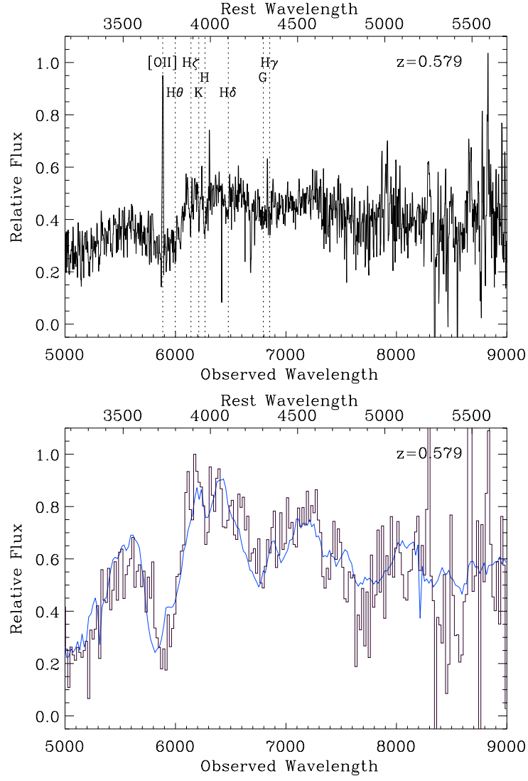
Fig. 11.— (Upper) Unsmoothed spectrum of the host of SN 1997af showing the narrow lines used to determine the redshift. (Lower) rebinned spectrum of SN 1997af (histogram) after interpolating across narrow lines from the host galaxy and subtracting an SB6 galaxy template, compared with the Type Ia SN 1999bp at -2 days (smooth curve).
