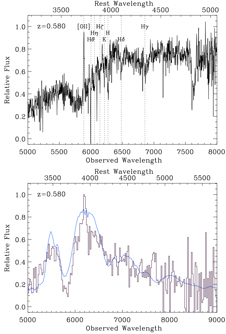
Fig. 3.— (Upper) Unsmoothed spectrum of SN 1997F showing narrow features used to determine the redshift (note that atmospheric absorption has not been corrected in this spectrum). (Lower) Rebinned spectrum of SN 1997F (histogram) after interpolating over narrow galaxy lines and sky absorption feature at 7600\text{\AA} , and subtracting template Sa galaxy, compared with SN 1999ee at -8 days (smooth curve).
