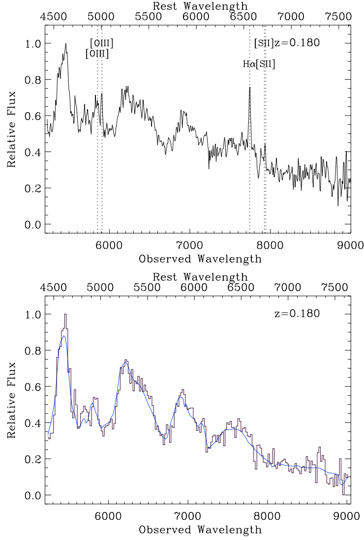
Fig. 7.— (Upper) Unsmoothed spectrum of SN 1997N showing the narrow lines used to determine the redshift. (Lower) Rebinned spectrum of SN 1997N (histogram) after interpolating over strong emission lines of [OIII] and H\alpha and subtracting template SB2 host galaxy light, compared with SN 1991T at +15 days (smooth curve).
