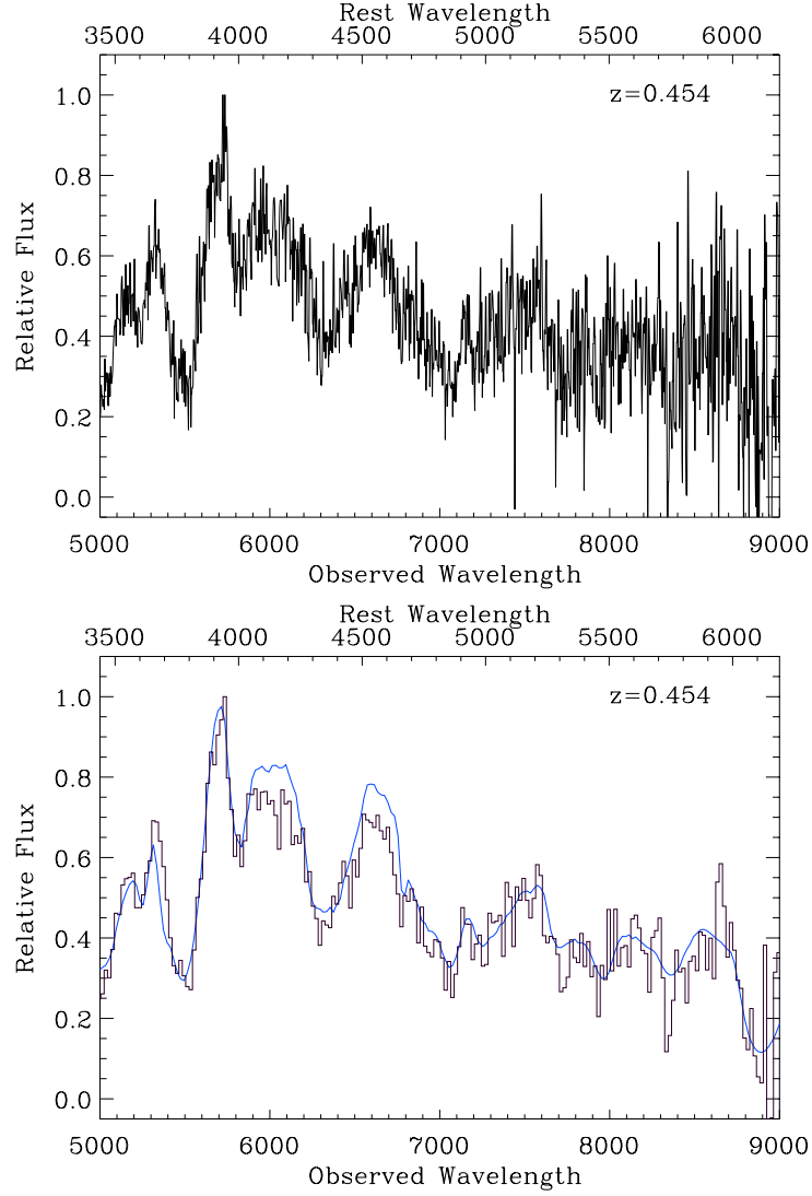
Fig. 13.— (Upper) Lightly smoothed spectrum of SN 1997ai. (Lower) rebinned spectrum of SN 1997ai (histogram) compared to the Type Ia SN 1992A at +5 days (smooth curve).
