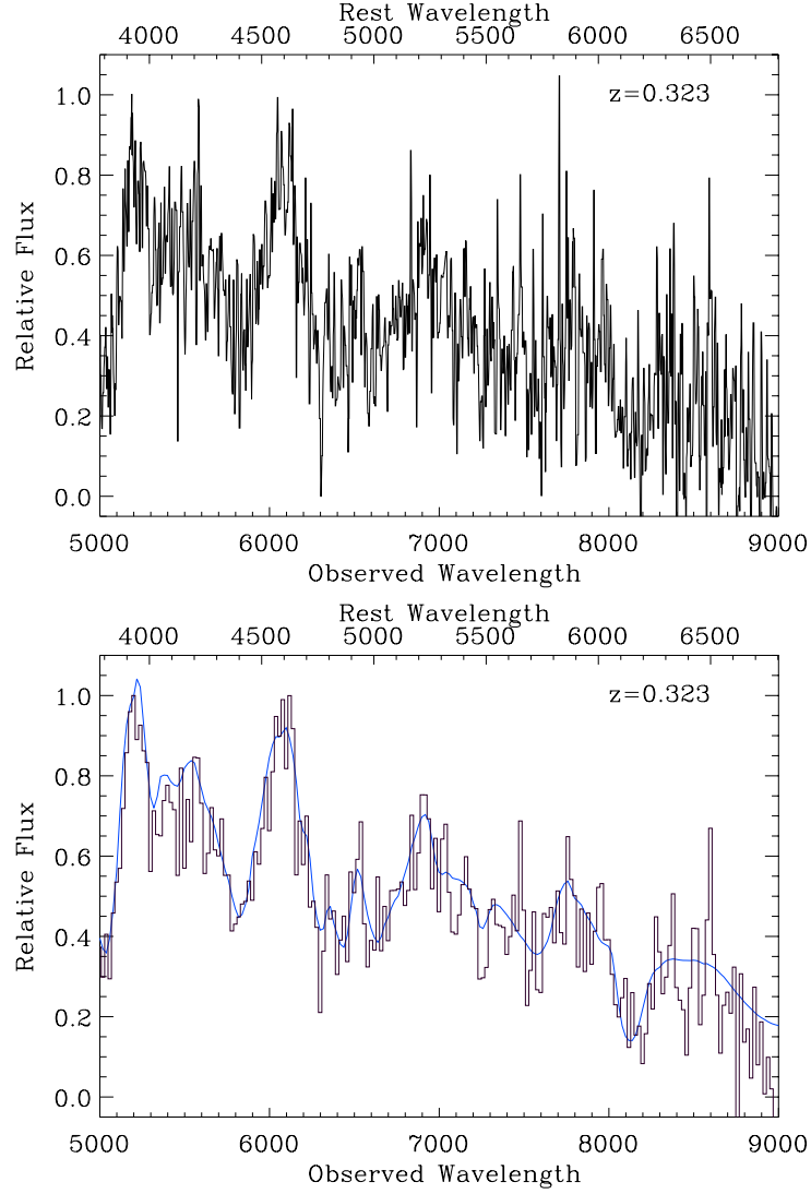
Fig. 10.— (Upper) lightly smoothed spectrum of SN 1997ac. (Lower) rebinned spectrum of SN 1997ac (histogram) compared with SN 1998bu at +11 days (smooth curve).
