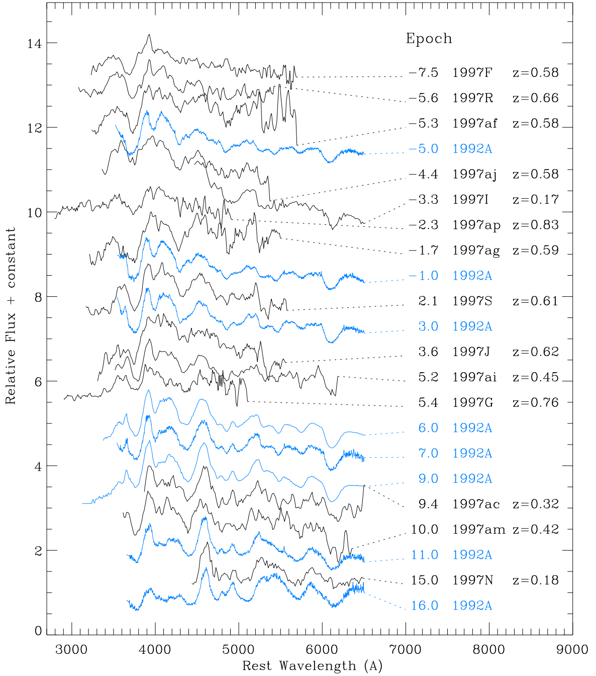
Fig. 17.— The time sequence of high redshift supernova spectra in order of rest-frame date relative to maximum light, as determined from the light curve ( \tau_c ). Spectra of the nearby Type Ia, SN 1992A are interspersed for comparison.
