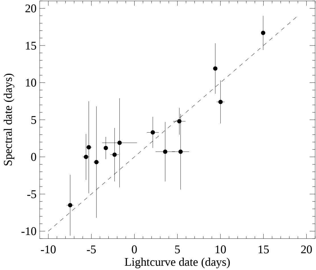
Fig. 2.— Comparison of the epoch of the spectrum as determined from the light curve ( \tau_{lc} ) with that determined from the weighted average of the 5 best template fits to the spectrum ( \tau_s ). In both cases the epochs are expressed as rest-frame days relative to maximum light. The dashed line shows the locus \tau_{lc} = \tau_s .
