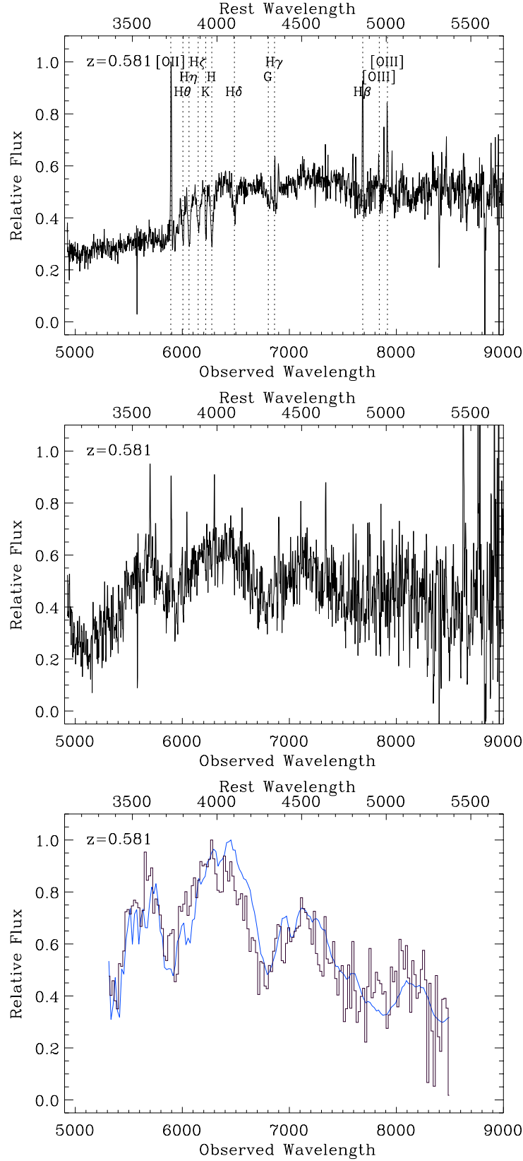
Fig. 14.— (Upper) Unsmoothed spectrum of the host of SN 1997aj (a separate extraction was possible although there are still narrow galaxy lines in the SN extraction) showing the narrow lines used to determine the redshift. (Middle) lightly smoothed spectrum of the supernova SN 1997aj. (Lower) Rebinned spectrum of SN 1997aj (histogram) after interpolating over narrow host galaxy lines of [OII] and Ca H&K and subtracting Sb galaxy light, compared with the Type Ia SN 1999aa at -3 days (smooth curve).
