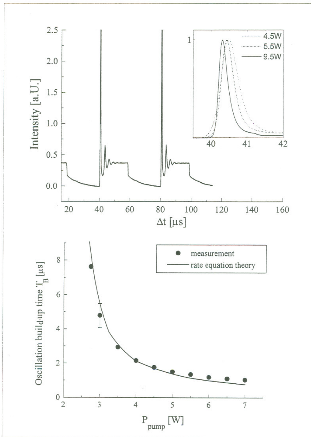
Figure III.7: Top: Q-switched pulse train as monitored through M5. The Q-switch is opened \approx 1 \mu s before the initial spike builds up. The inlay shows the different shapes of the Q-switched pulse for different pump powers on a normalized scale. Bottom: Delay in buildup of a Q-switched pulse vs. pump power.
