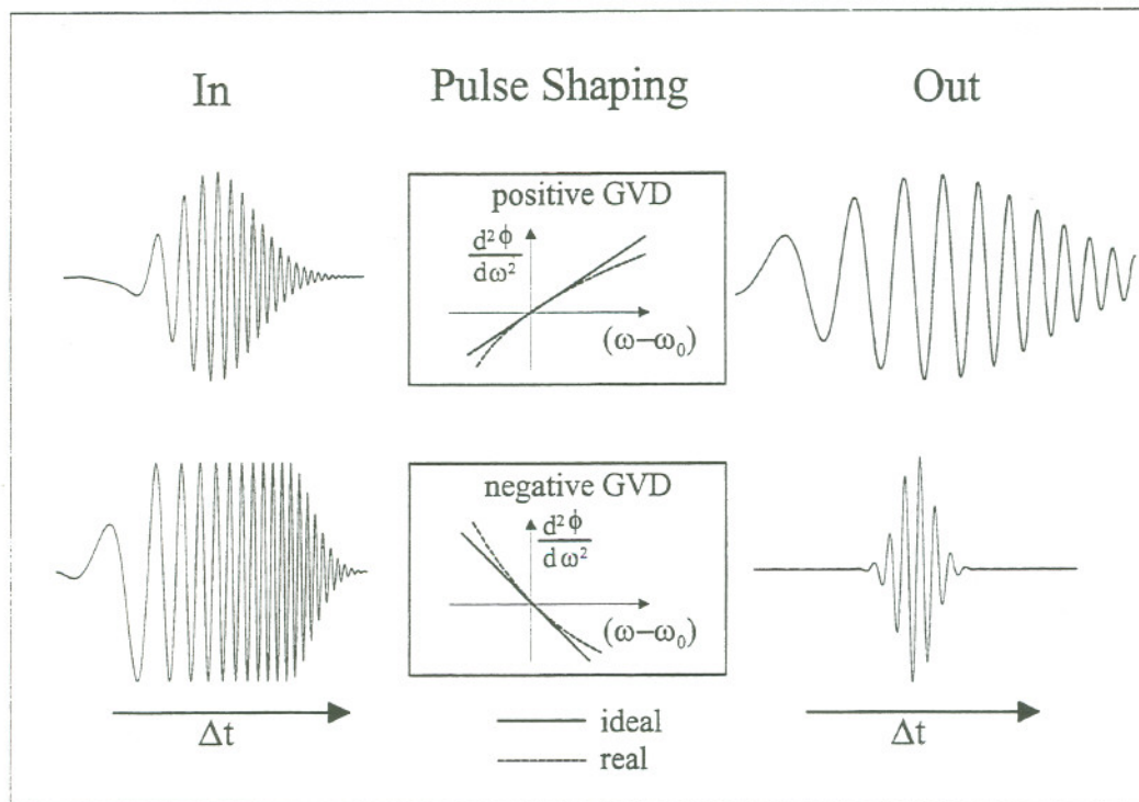
Figure IV.4: Different steps of pulse shaping. Top: A chirped pulses experiences GVD and broadens in time. Bottom: A chirped, broad pulse can be compressed to a short pulse by negative GVD (all frequency components "catch up" with each other).
