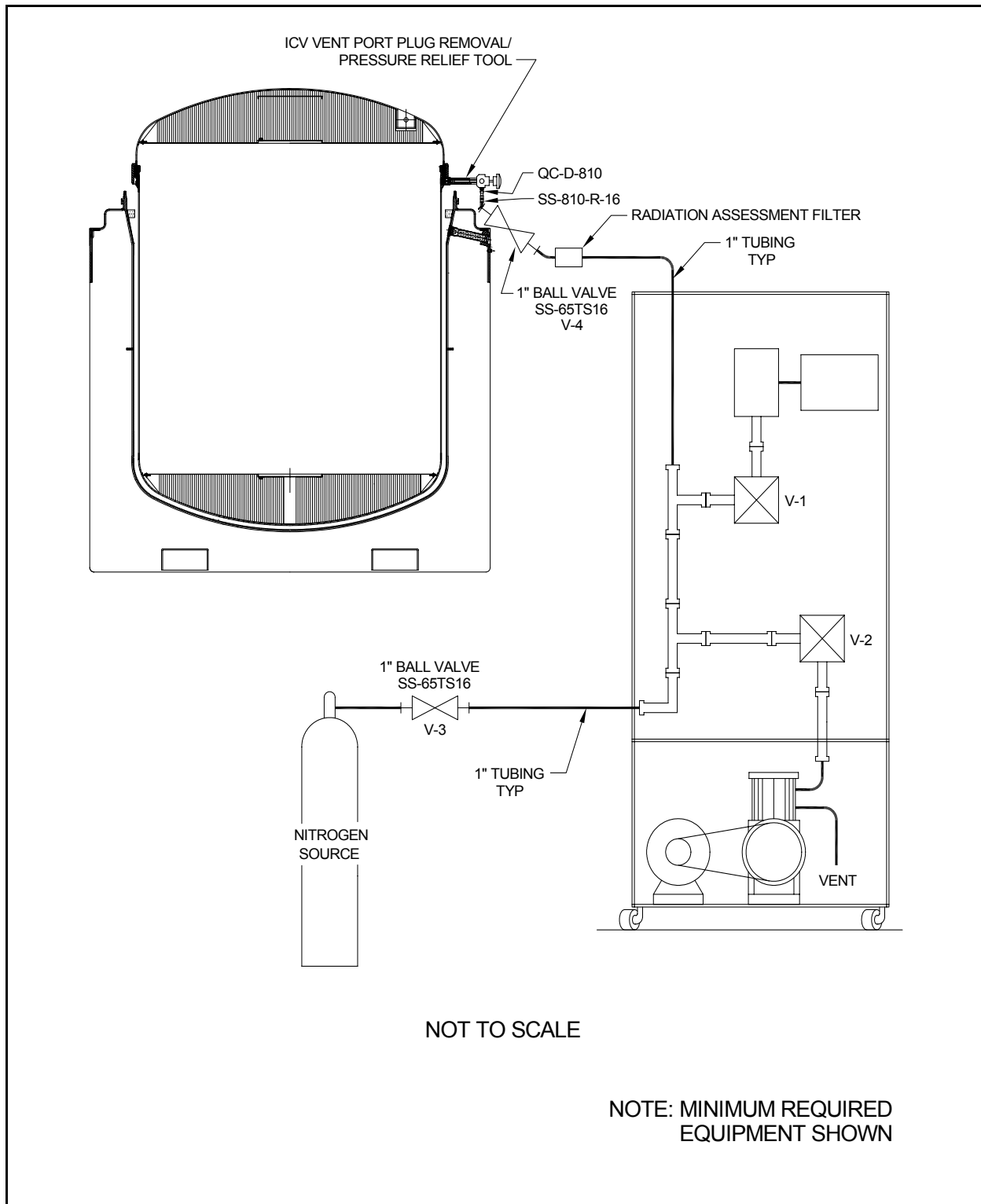
Figure 2.1 - Evacuation/Nitrogen Backfill
