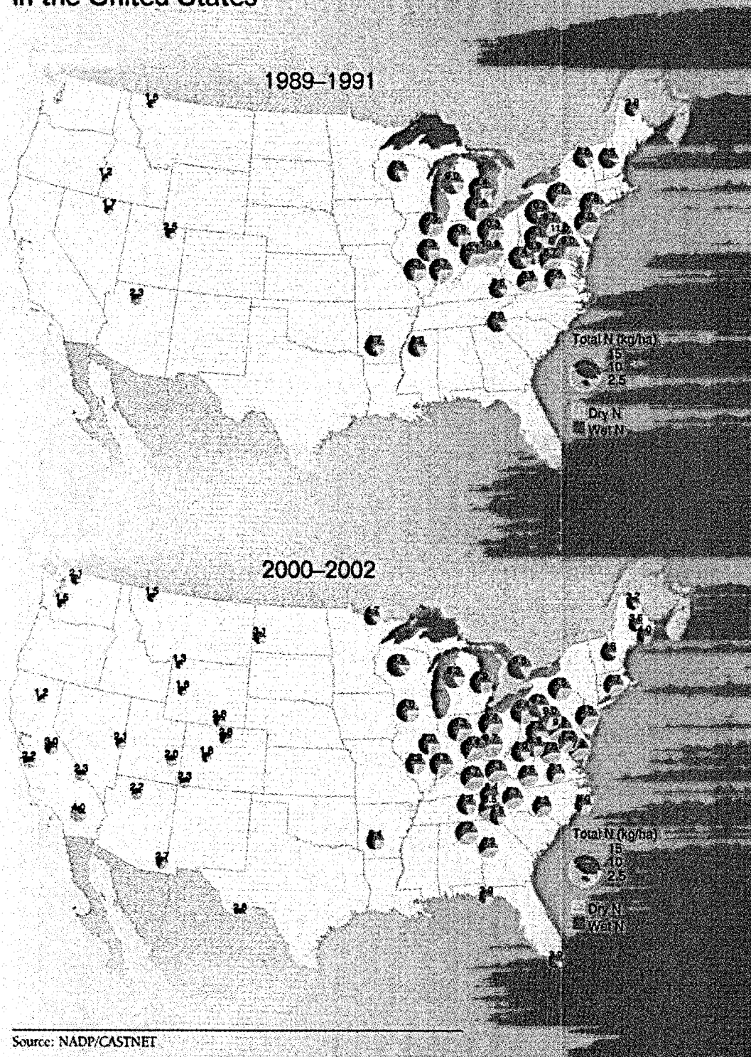
FIGURE 25. Comparison of annual total (wet plus dry) nitrogen deposition in the United States
