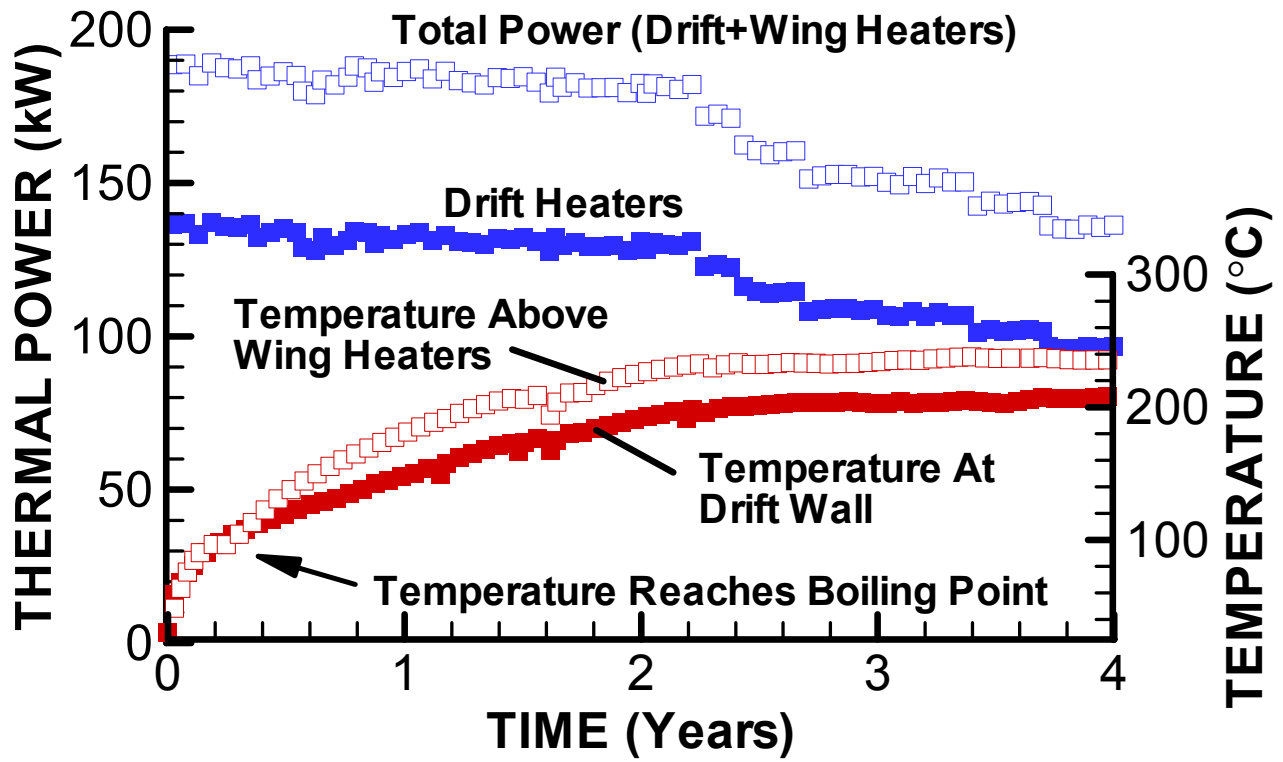
ig. 5. Thermal power and measured temperature at the drift wall and at a monitoring point located above the wing heater at a horizontal distance of 10 m from the center of the drift.
