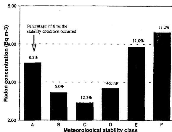
Fig. 2 Average Radon Concentrations vs. Meteorological Stability Classes at NF6 during April 1994
