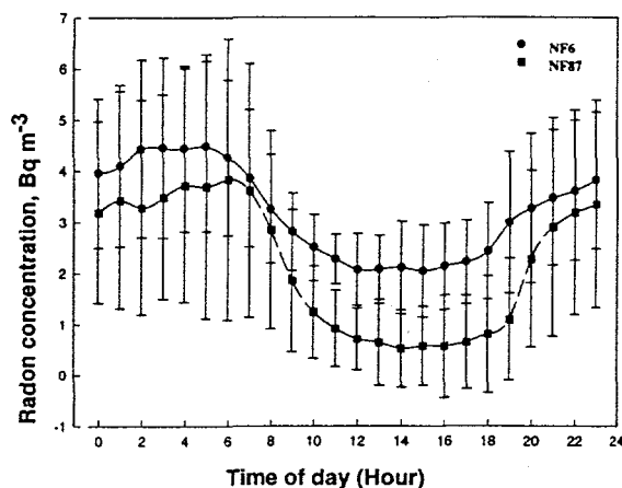
Fig. 1 Hourly Average Radon Concentrations at NF6 and NF87 during April 1994
