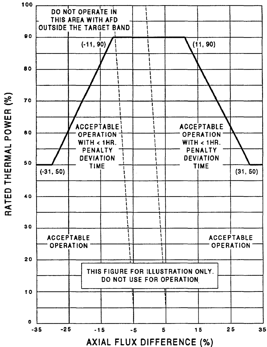
Figure B 3.2.3A-1 (Page 1 of 1) AXIAL FLUX DIFFERENCE Acceptable Operation Limits and Target Band Limits as a Function of RATED THERMAL POWER
