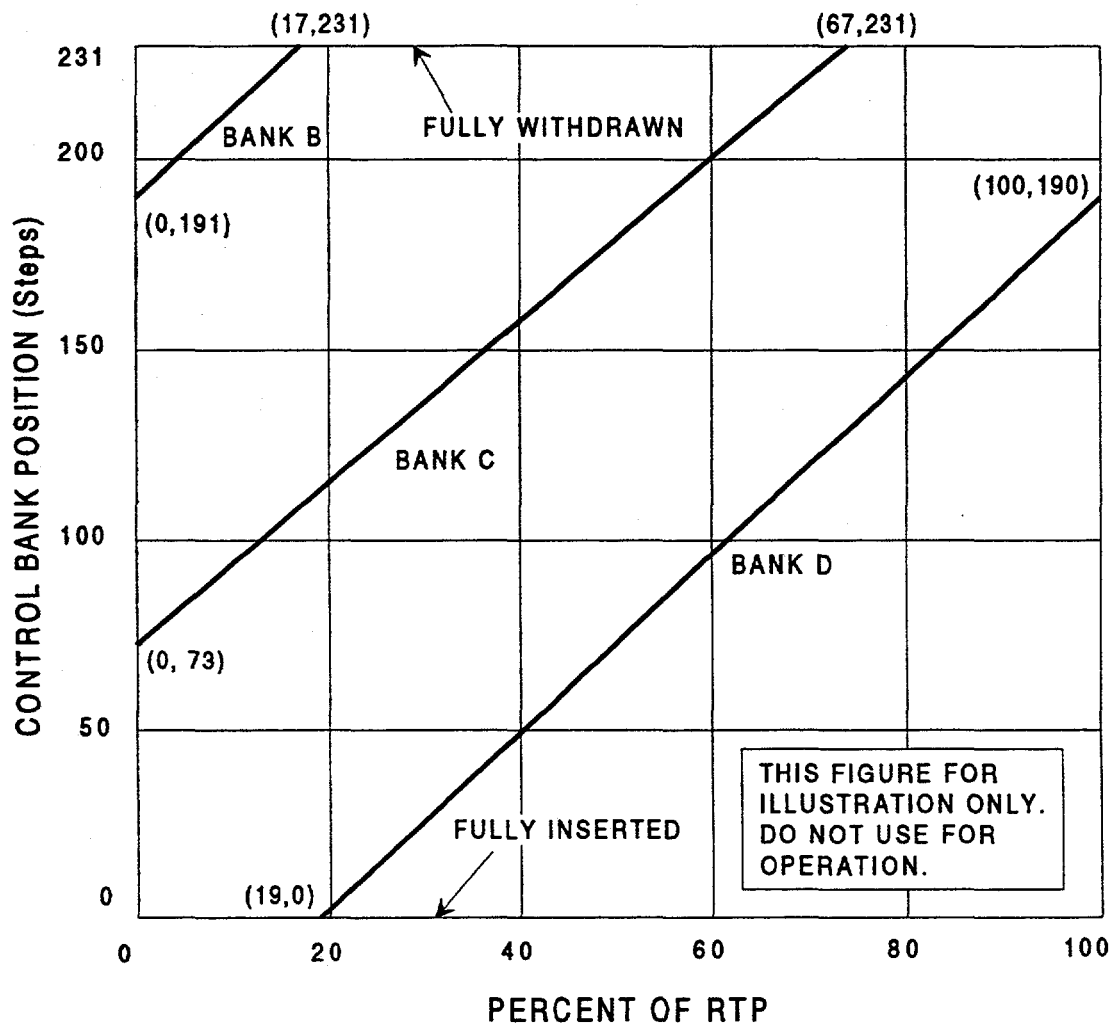
Figure B 3.1.7-1 (page 1 of 1) Control Bank Insertion vs. Percent RTP
