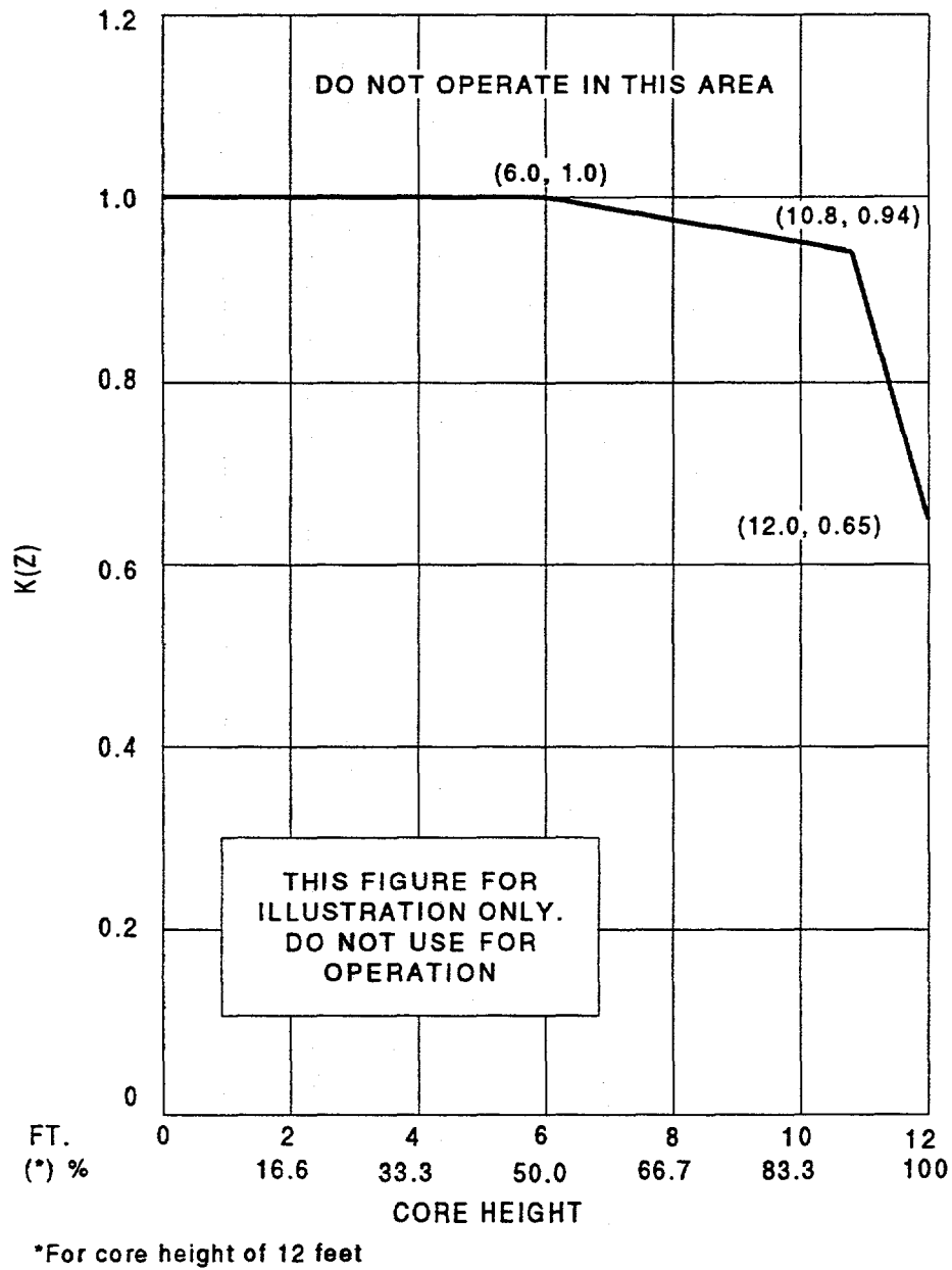
Figure B 3.2.1B-1 (page 1 of 1) K(Z) - Normalized F_q(Z) as a Function of Core Height
