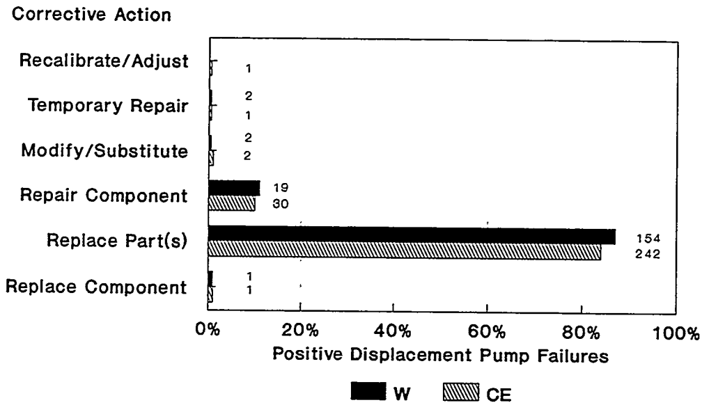
Figure 4.22 Pump failures vs. corrective action (NPRDS)
