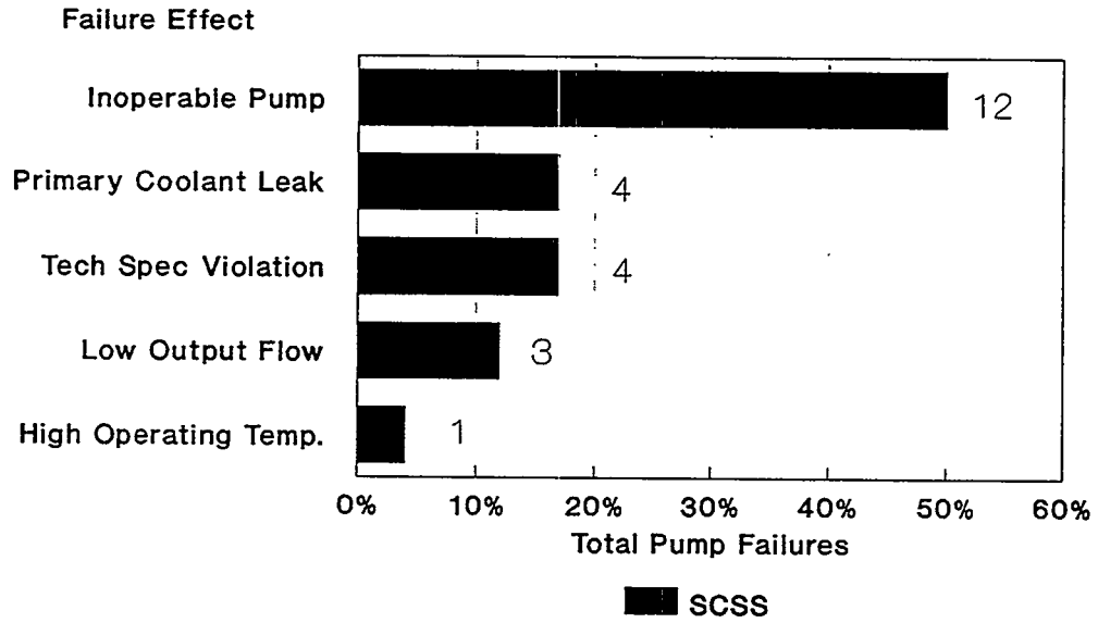
Figure 4.38 Pump failure vs. failure effect (SCSS)
