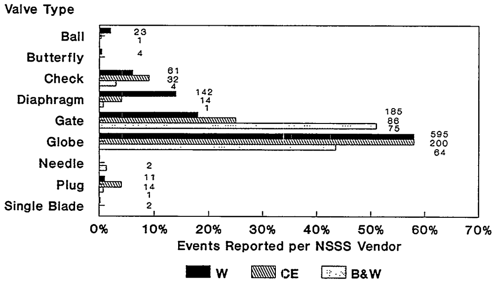
Figure 4.9 Valve failures vs. valve type (NPRDS)
