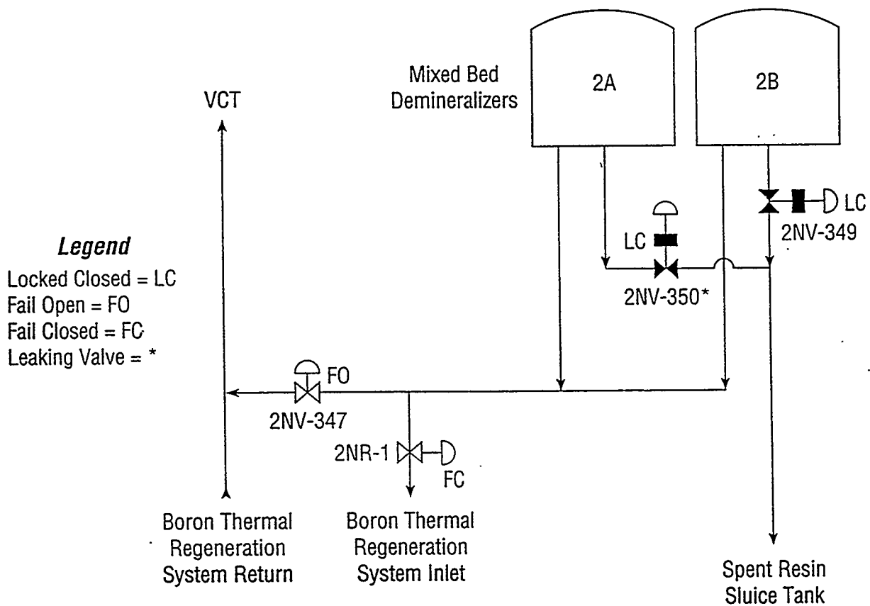
Figure 7.2 Flow diagram CVCS and boron thermal regeneration interface
