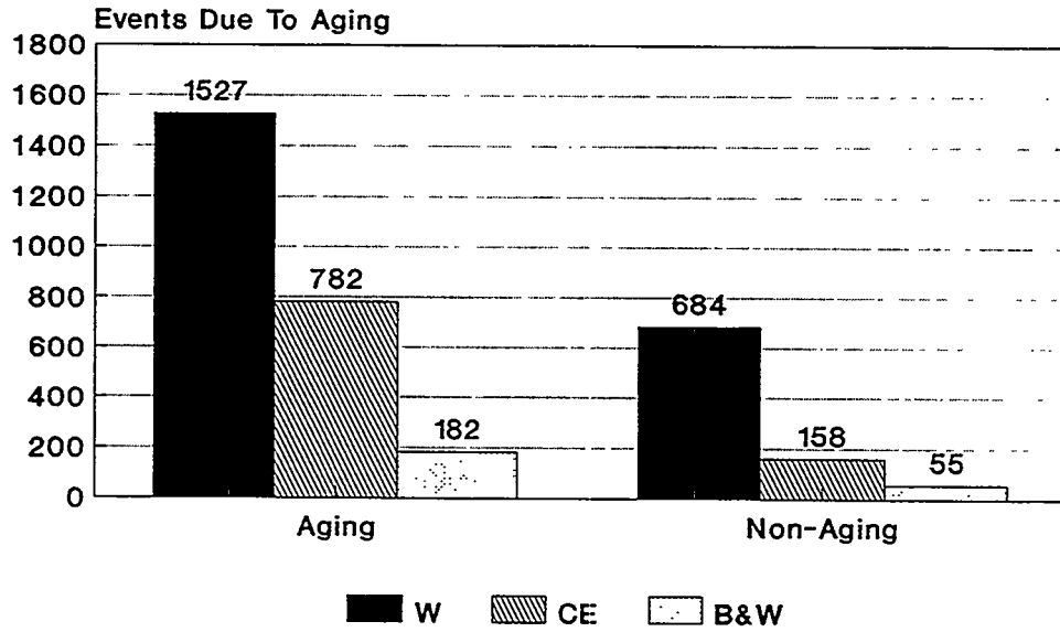
Figure 4.7 CVCS failures attributable to aging (NPRDS)
