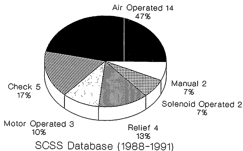
Figure 4.33 Valve failures vs. valve type (SCSS)
