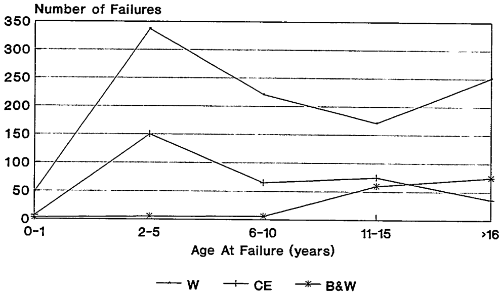
Figure 4.11 Valve age at failure (NPRDS)
