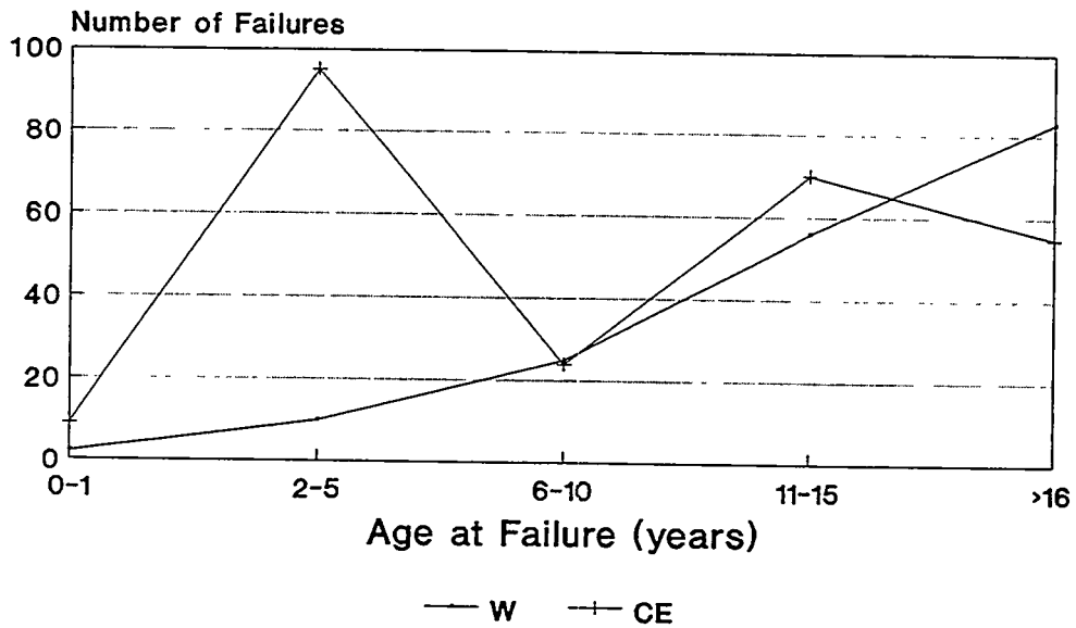
Figure 4.18 Pump age at failure (NPRDS)
