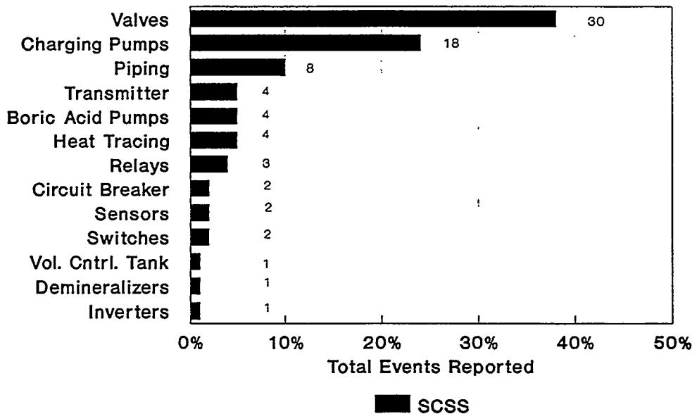
Figure 4.3 CVCS component failures reported to SCSS
