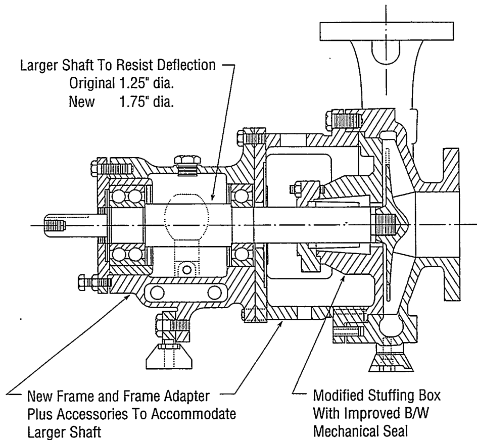
Figure 6.1 Boric acid transfer pump modifications
