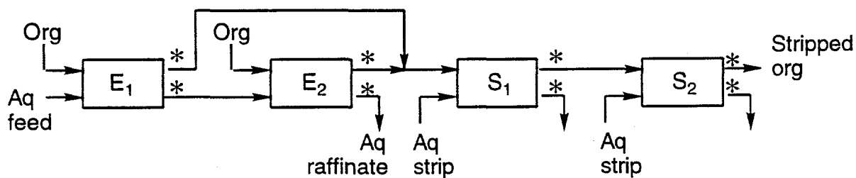
Scheme 1. Cross-current two-extraction two-strip contacting procedure (1:1 volume ratios) used for tests in this work. The asterisk (*) denotes when samples were taken for analysis. (Note: this is not meant to represent a process flowsheet).
