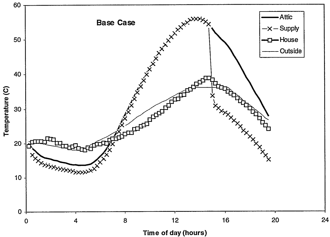
Figure 2. Simulation results for the base case system for a Sacramento Design day.
