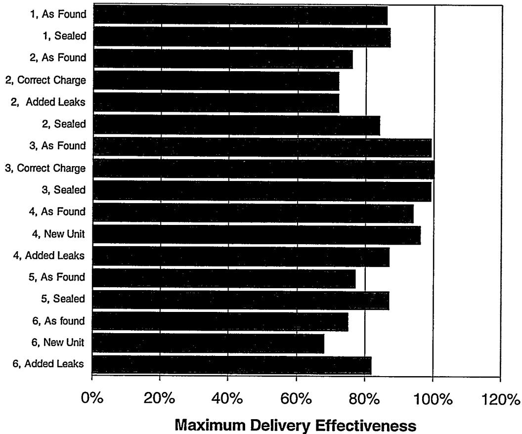
Figure 3. Comparison of maximum delivery effectiveness between systems and the increase in delivery efficiency for sealed systems
