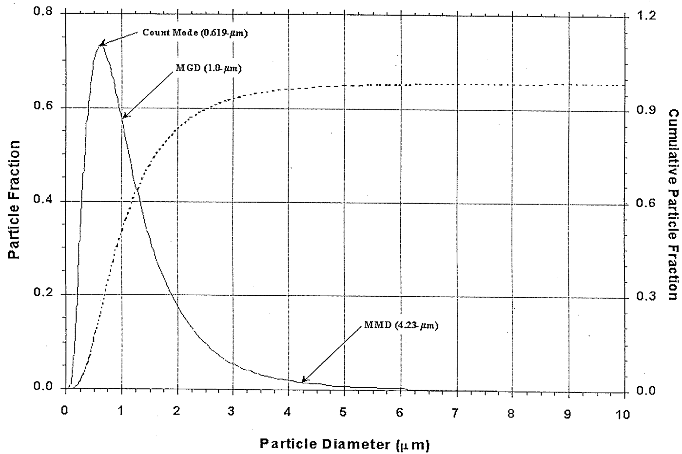
Figure 7-4. Typical Normalized and Integrated Log-Normal Particle Distribution Function (MGD = 1- \mu\text{m} and \sigma = 2 )
