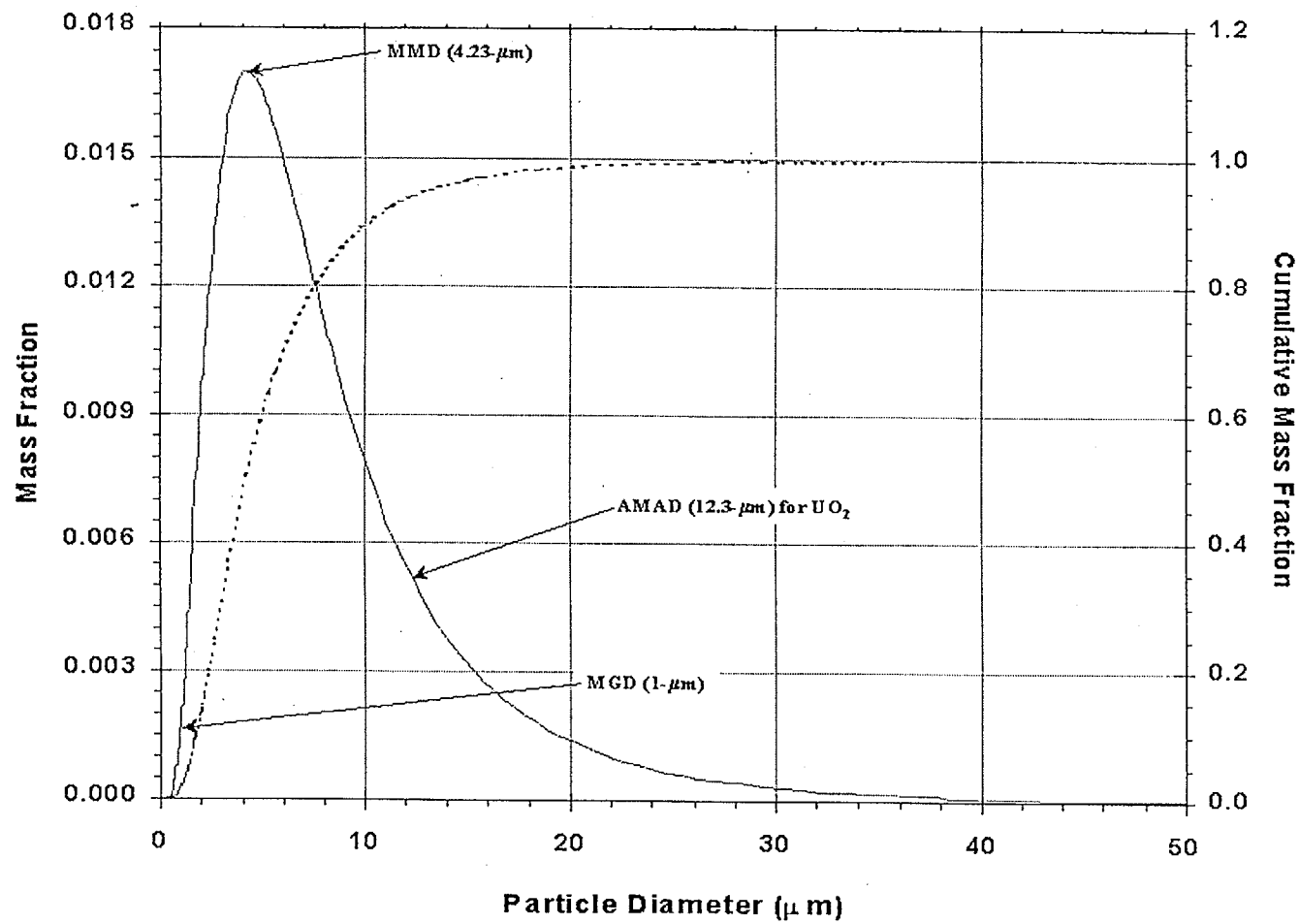
Figure 7-5. Typical Normalized and Integrated Log-Normal Mass Distribution Function (MGD = 1\text{-}\mu\text{m} and \sigma = 2 )
