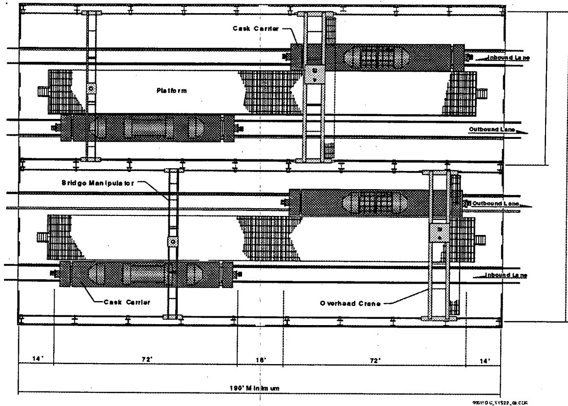
Figure 4. Carrier Preparation Building Floor Plan
