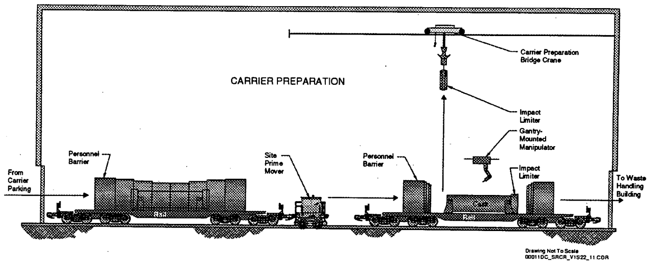
Figure 3. Carrier Preparation Building Materials Handling System
