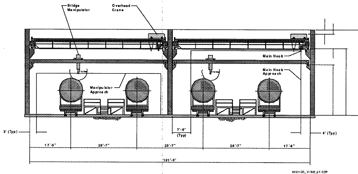
Figure 5. Carrier Preparation Building Section
