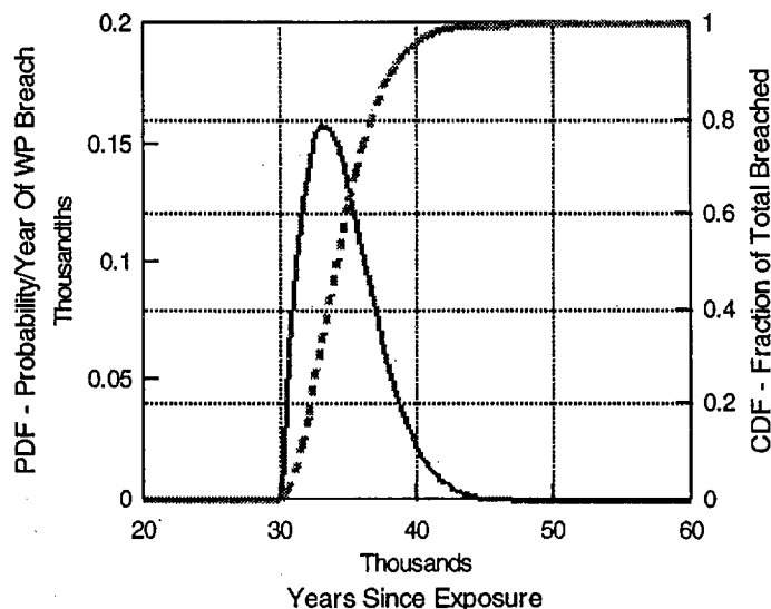
Figure 7.9. Distribution of disposal container breach failures developed using McCoy's model and parameters for intermittent wetting.
