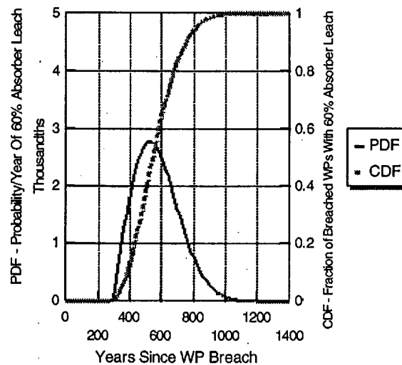
Figure 7.13. Distribution of time to leach 60% of neutron absorbing material from MPC-WP basket structure exposed to intermittent wetting conditions.
