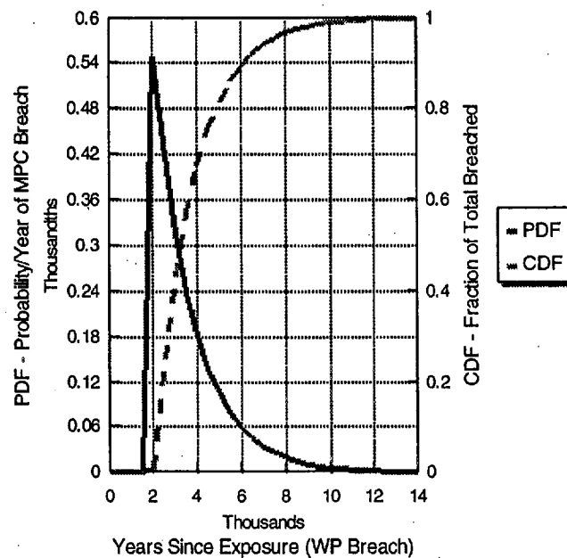
Figure 7.10. Distribution of MPC shell breach failures under continuously wetted conditions
