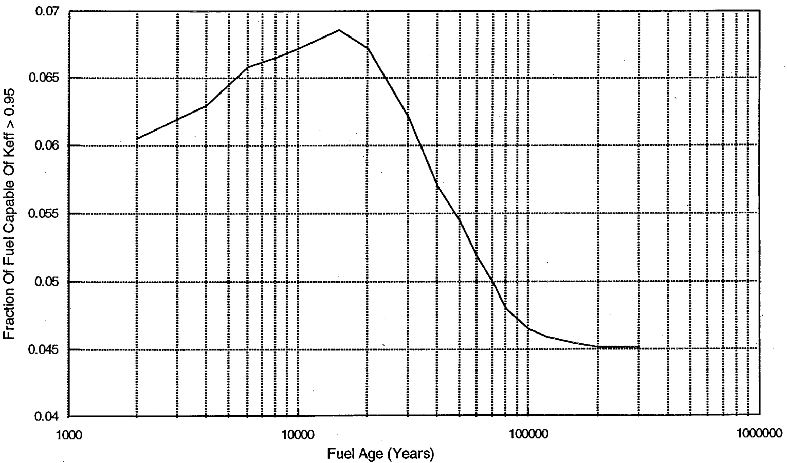
Figure 7.14. Fraction of design basis fuel (3% initial enrichment, 20 GWd/MTU Burnup) as a function of time capable of achieving k_{eff} > 0.95 in an MPC-WP geometry with no neutron absorber in the basket structure.
