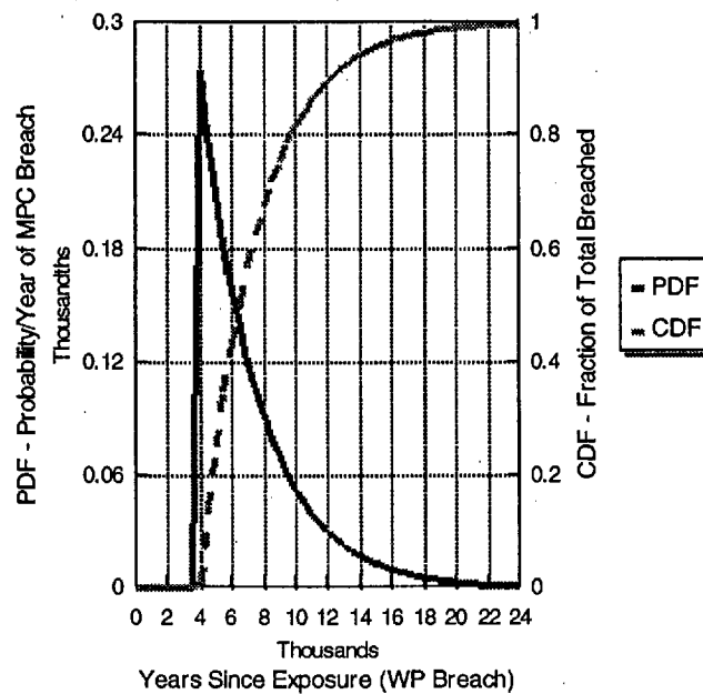
Figure 7.11. Distribution of MPC shell breach failures for intermittent wetting conditions.
