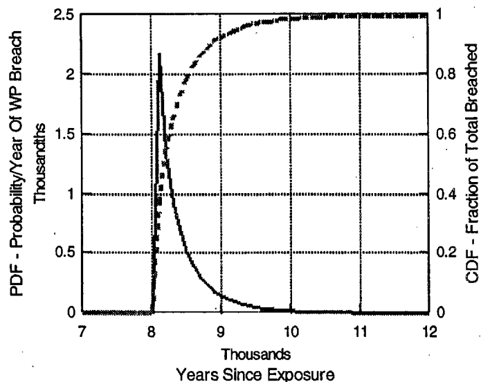
Figure 7.8. Distribution of disposal container breach failures developed using McCoy's model and parameters for continuous wetting.
