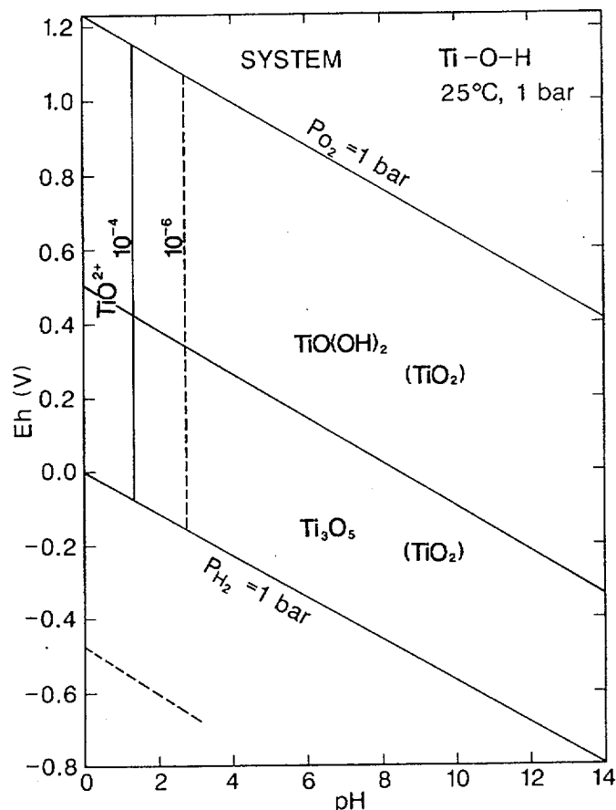
Figure 7. Eh-pH diagram for part of the system Ti-O-H. Assumed activity for Ti = 10^{-6} . Note TiO 2 occupies all Eh-pH space shown as TiO(OH) 2 and Ti 3 O 5 (Brookins 1988).
