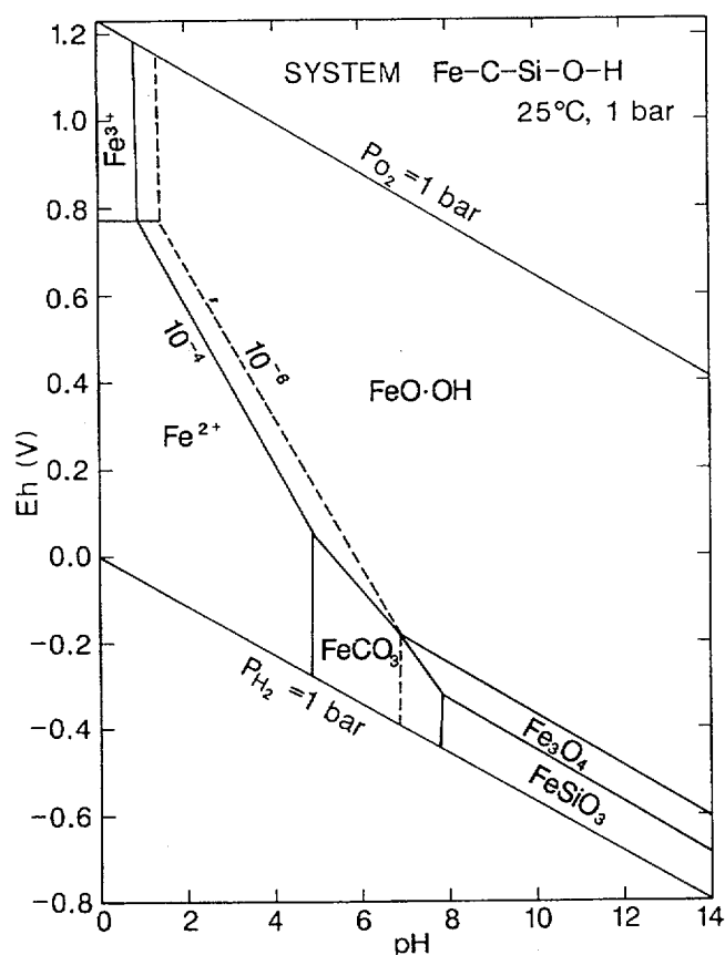
Figure 2. Eh-pH diagram for part of the system Fe-C-Si-O-H. Assumed activities for dissolved species are: Fe = 10^{-6} , Si = 10^{-3} , C = 10^{-3} . Goethite and magnetite assumed as Fe(III) solid phases (Brookins 1988).
