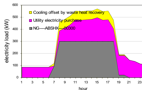
Figure 2. Office July Electricity Load Provision with CHP.
