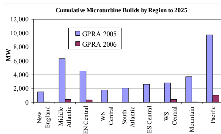
Figure 4. Microturbine Capacity
