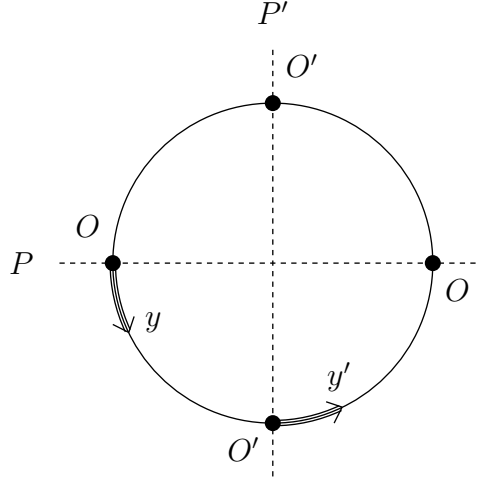
Figure 1: S^1/(Z_2 \times Z'_2) orbifold in the fifth dimension.
