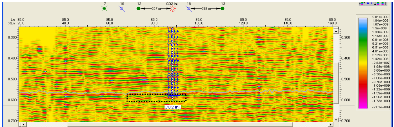
Figure 7. Seismic amplitude section, interpreted target top horizon (gray), and seismic synthetics at well CO2I#1. Gas shadow effect is evident below time horizon in the vicinity of the injection well.
