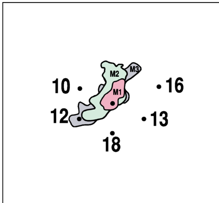
Figure 9. Interpreted boundary of the CO 2 plume based on the first three monitor surveys (January, March, June 2004). Note CO 2 movement toward well #13 only began to occur between the March and June surveys in response to increased water injection in well 7. Also note the northwest appendage evident on the March 2004 survey has receded in response to the increased water injection in well 10.
