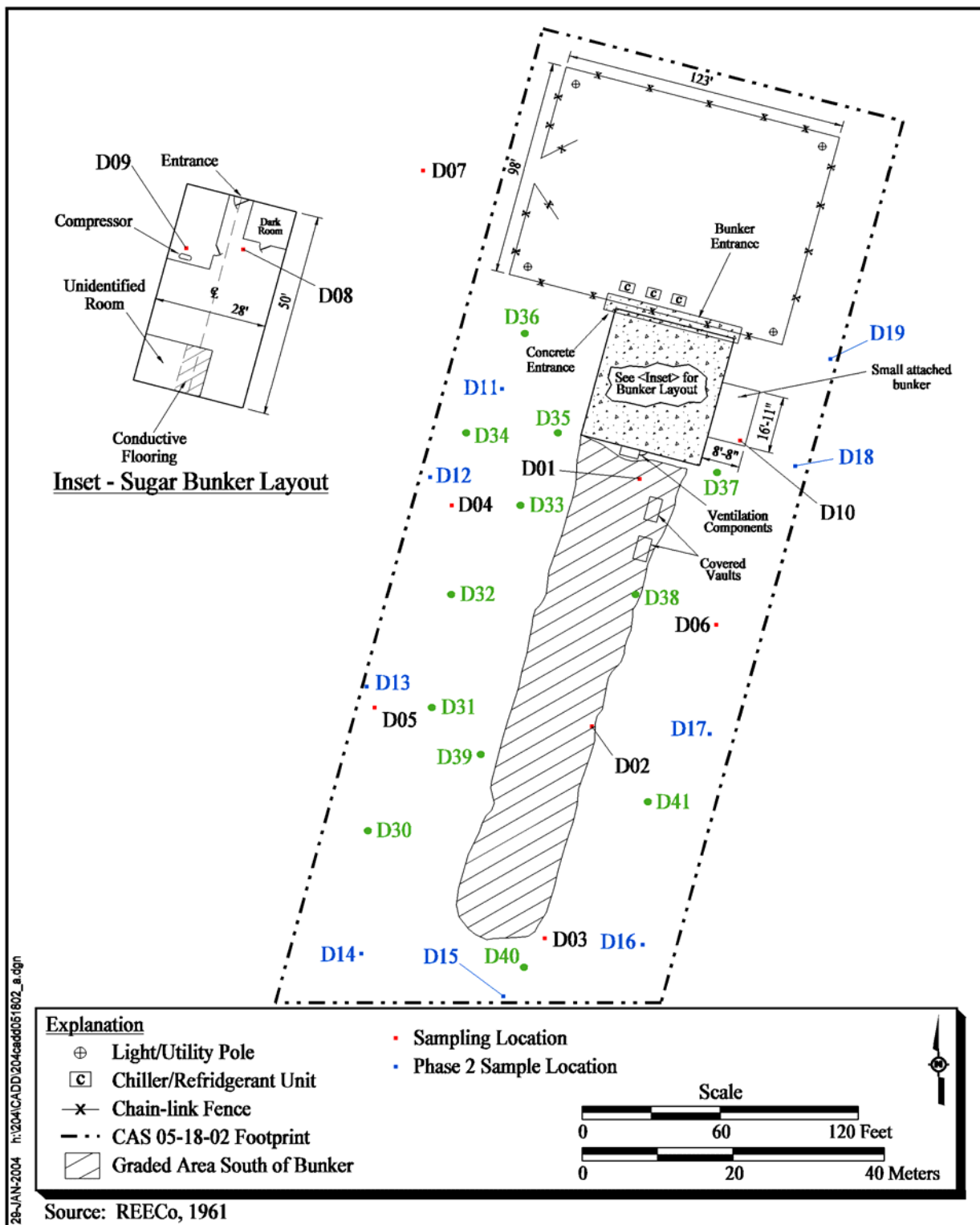
Figure A.6-1 CAS 05-18-02, Sampling Locations
