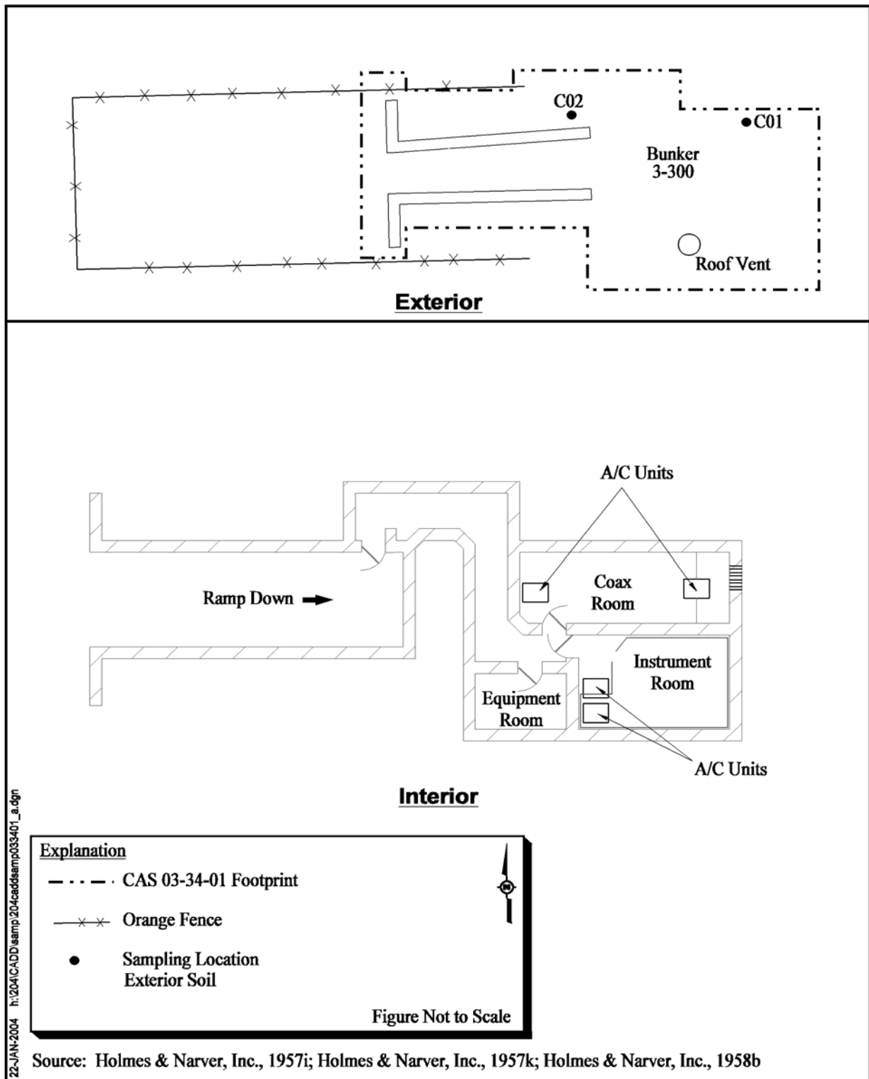
Figure A.5-1 CAS 03-34-01, Sampling Locations
