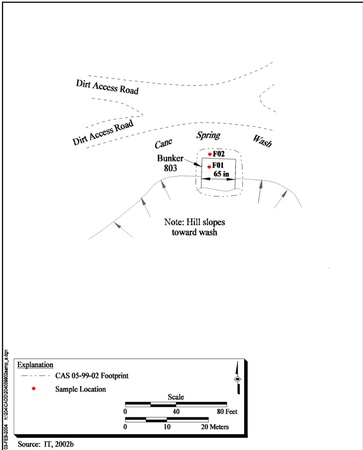
Figure A.8-1 CAS 05-99-02, Sampling Locations
