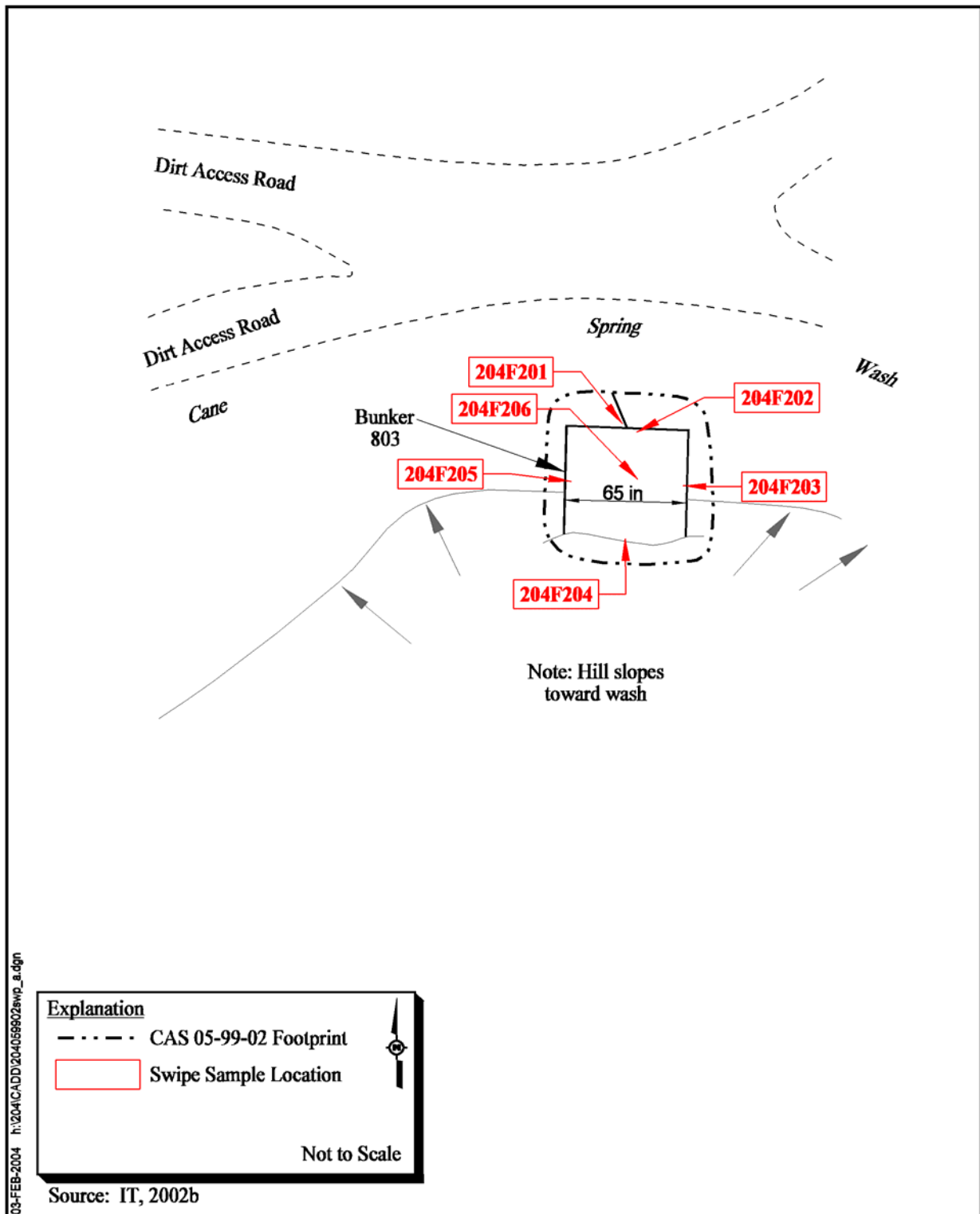
Figure A.8-2 CAS 05-99-02, Radiological Swipe Sample Locations, Bunker Interior
