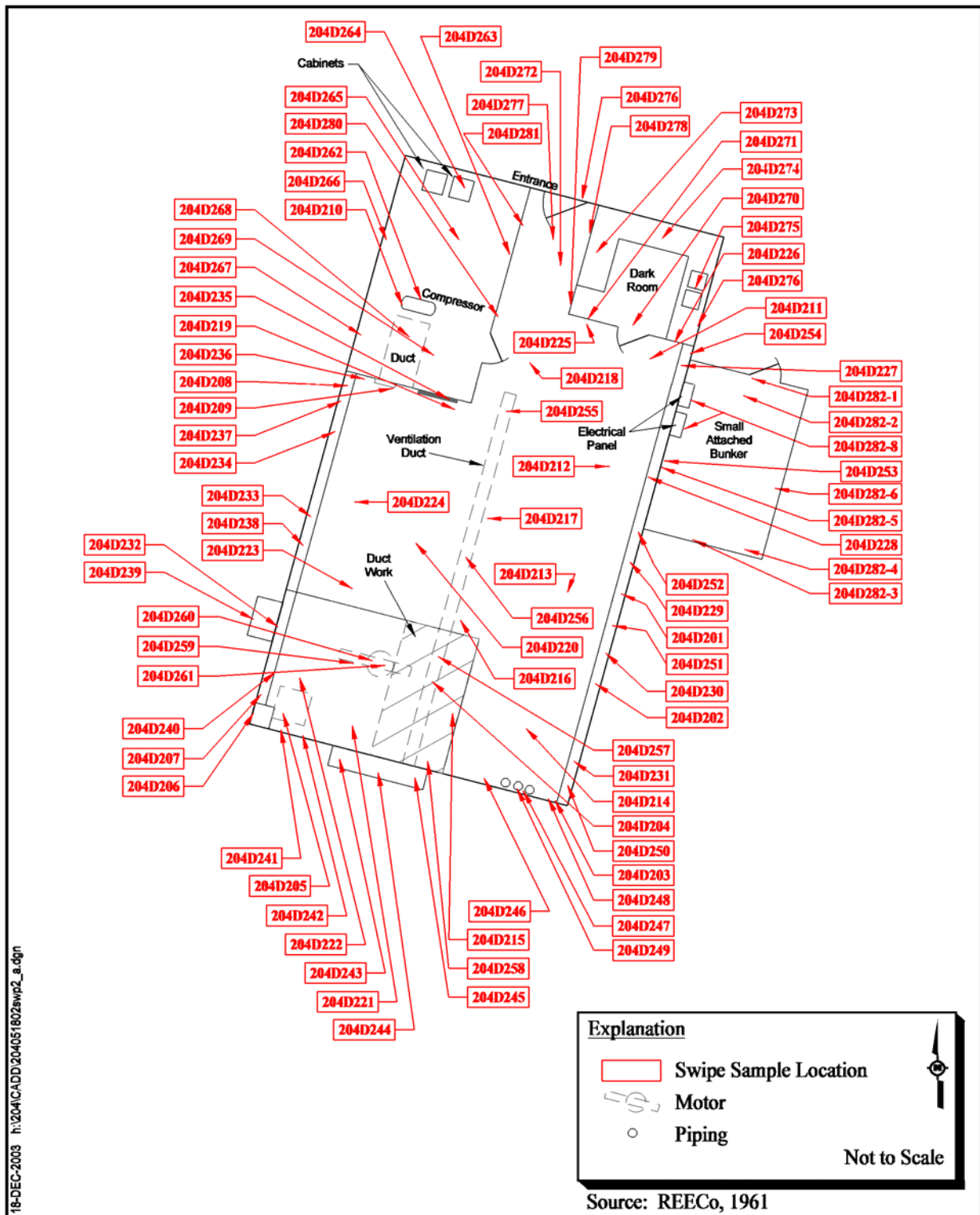
Figure A.6-2 CAS 05-18-02, Swipe Sample Locations, Bunker Interior
