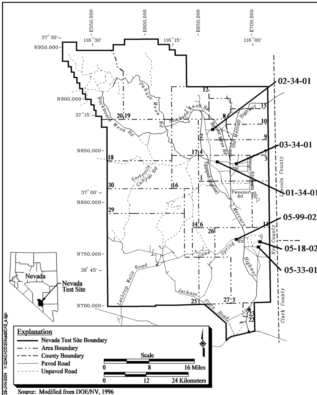
Figure 1-2 CAU 204, Storage Bunkers CAS Location Map
