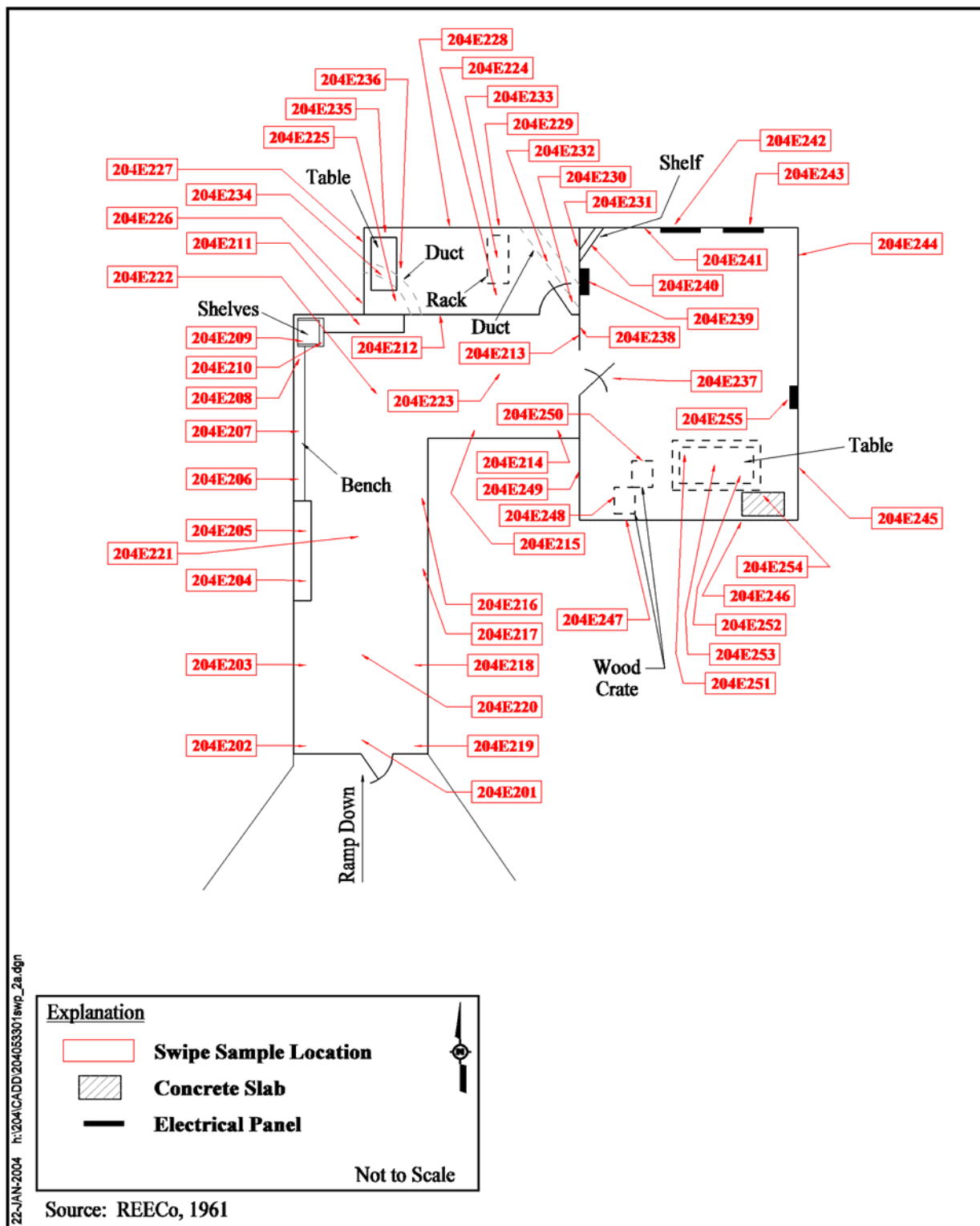
Figure A.7-3 CAS 05-33-01, Radiological Swipe Sample Locations
