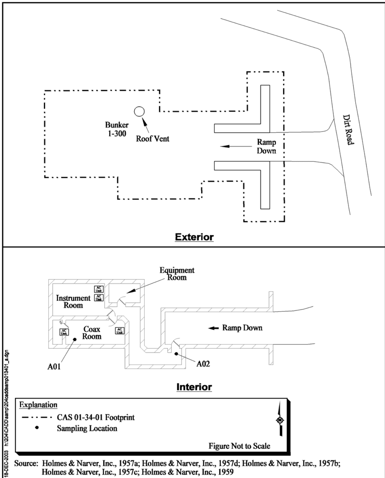
Figure A.3-1 CAS 01-34-01, Sampling Locations
