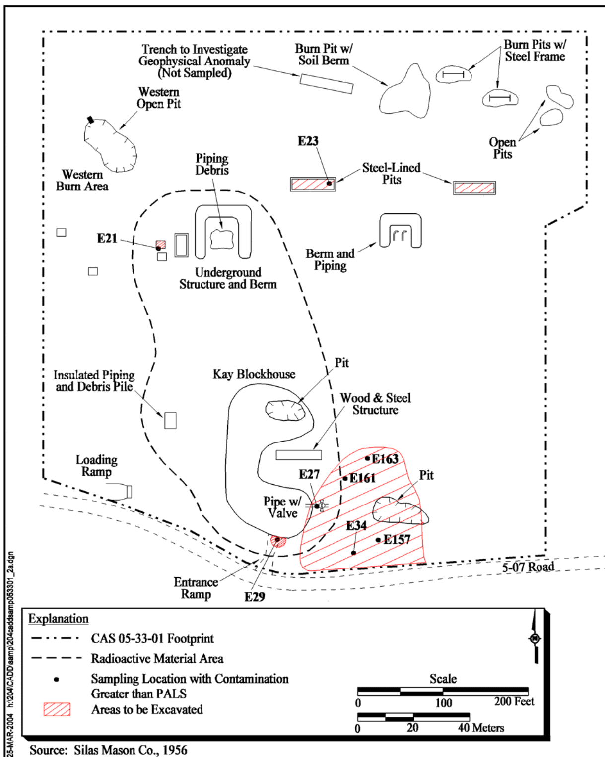
Figure 4-1 CAS 05-33-01, Kay Blockhouse Areas of Excavation
