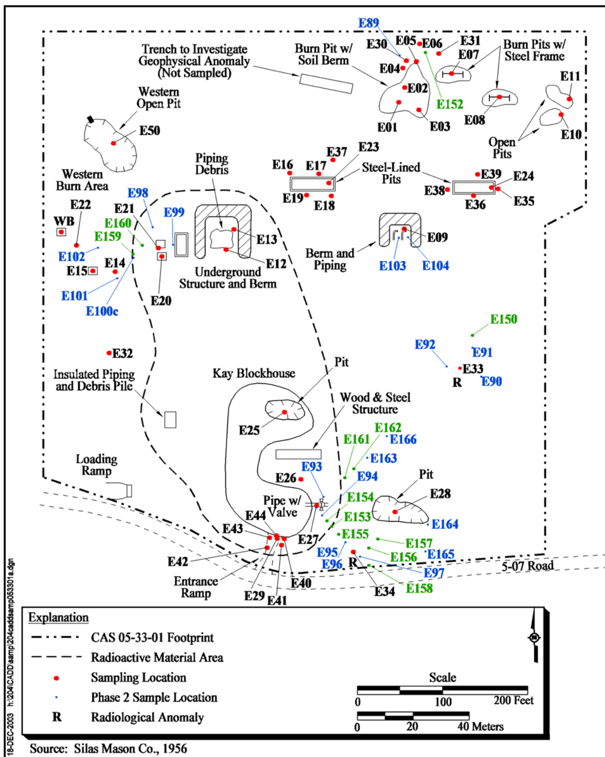
Figure A.7-1 CAS 05-33-01, Sampling Locations Exterior Soils
