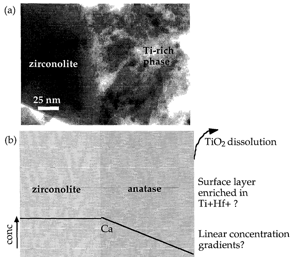
Figure 4. Reacted zirconolite: (a) TEM image of reaction surface showing ~100 nm thick Ti-rich alteration layer, which is identified as anatase ( \text{TiO}_2 ) by electron diffraction (E. Buck, pers. com.). (b) Schematic of reacted zirconolite and hypothetical Ca concentration through alteration layer assuming steady state transport-limited dissolution.
