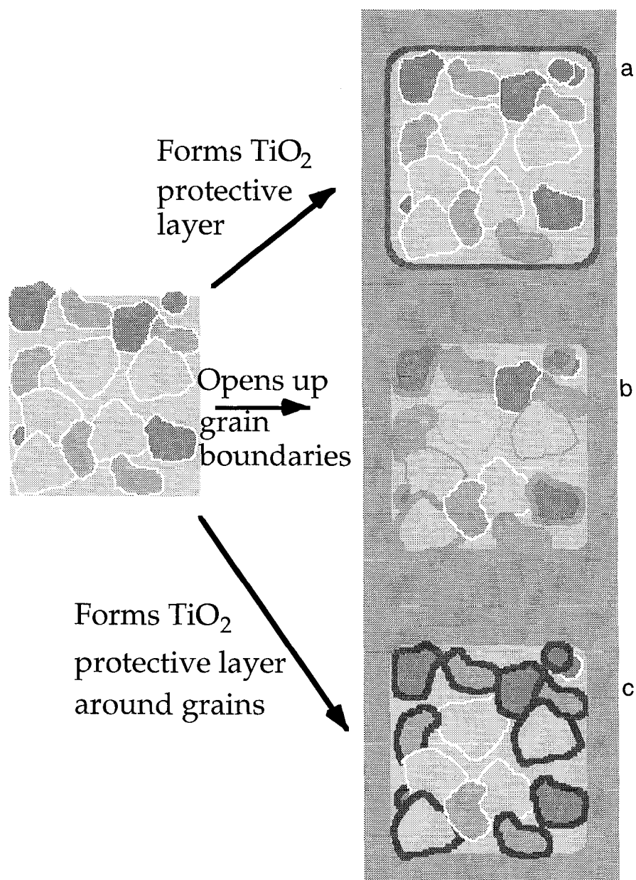
Figure 6. Possible effects of the ceramic dissolution process on surface area of ceramic-water contact.
