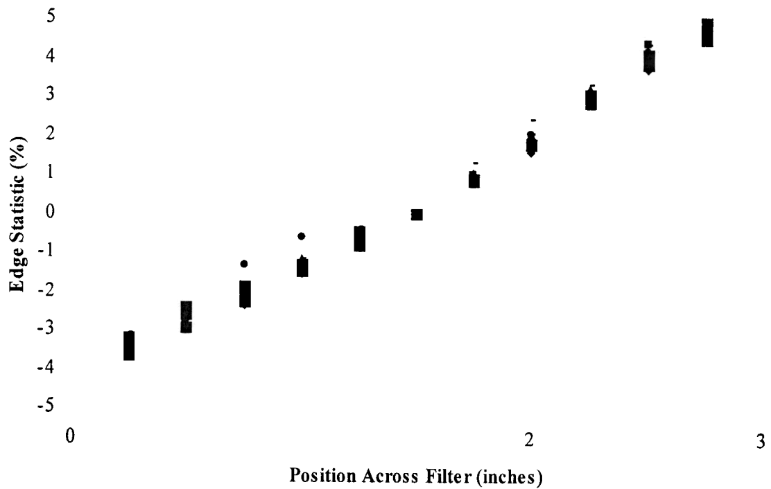
Figure 8 Edge performance statistic measured across an initial set of 10 tandem filters (3 inch diameter) showing 8 to10 % variability as the result of chamber geometry.
