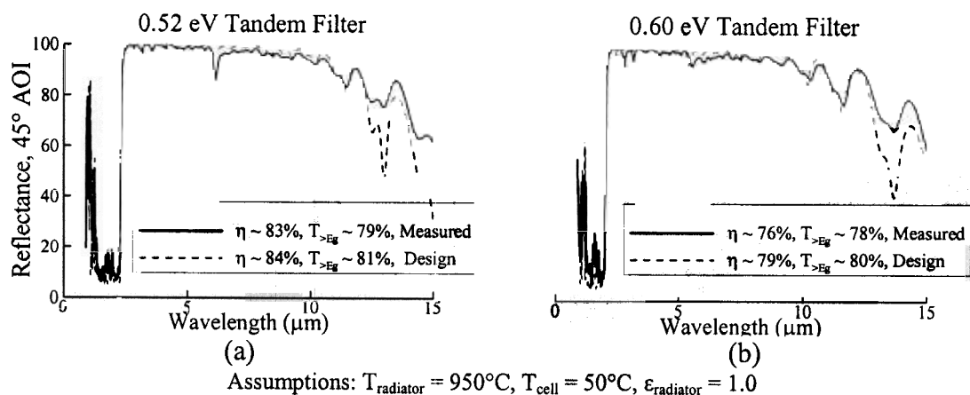
Figure 5 Current Spectral Performance of Front Surface, Tandem Filters for 0.52 eV (a) and 0.60 eV (b) Band Gap TPV Cells
