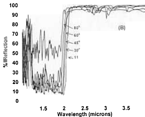
Figure 3: Measured reflection measurements of a 0.6 eV front surface filter highlight the shift in angle of the transition edge with angle of incidence (AOI). The pass band transmission degrades at near grazing angles.
