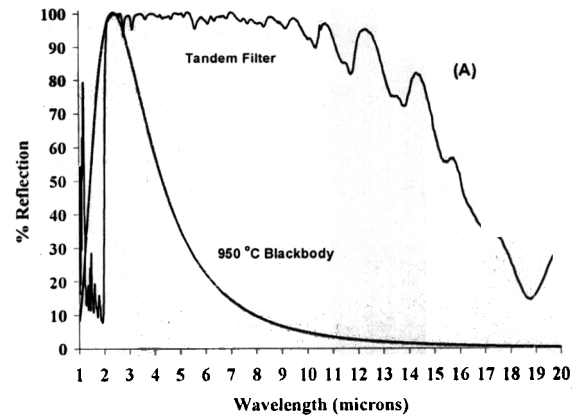
Figure 2: Measured reflection of a front surface tandem filter is plotted along with a black body spectrum for 950 °C. The filter's transition edge is placed at the cell's band gap. High reflection of below band gap photons is needed to achieve high spectral efficiency.
