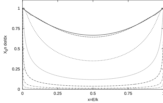
Figure 3. The differential cross section for pair production in water, as a function of x = E/k for photons with energies of 64 TeV (top curve), 640 TeV, 6.4 PeV, 64 PeV, 6400 PeV, 6.4 EeV and 64 EeV (bottom curve). These curves apply for other materials for photon energies of 0.23, 2.3, 23, 230, 2300, 23,000 and 230,000 E_{LPM} .
