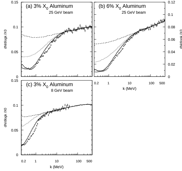
Figure 2. Data (points) from 8 and 25 GeV electrons passing through aluminum targets, from the SLAC E-146 collaboration, compared with calculations based on the Bethe-Heitler (dashed histogram), and Migdals LPM suppression (dot-dashed histogram), and on Migdals calculations with LPM and dielectric suppression (solid histogram). The data is binned logarithmically in photon energy, so the Bethe-Heitler 1/k spectrum is roughly flat.
