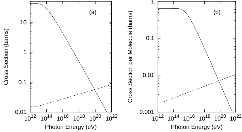
Figure 5. Comparison between the pair production and photonuclear interaction cross sections in (a) lead and (b) water. Above an energy of 10^{20} eV, the photonuclear cross section is larger than for pair production.
