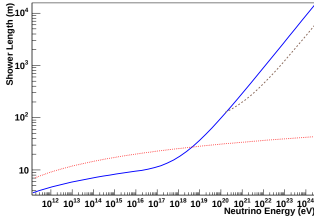
Figure 7. Shower length as a function of neutrino energy. The solid blue line is for a purely electromagnetic shower, while the dashed brown line is for a hybrid EM/hadronic shower. The dotted red line is for a purely hadronic shower. The difference between the hybrid and purely hadronic showers is that the hybrid includes the long electron path before bremsstrahlung, and the photon path before it interacts hadronically. For the hybrid and electromagnetic showers, the electron is assumed to take 80% of the \nu_e energy.
