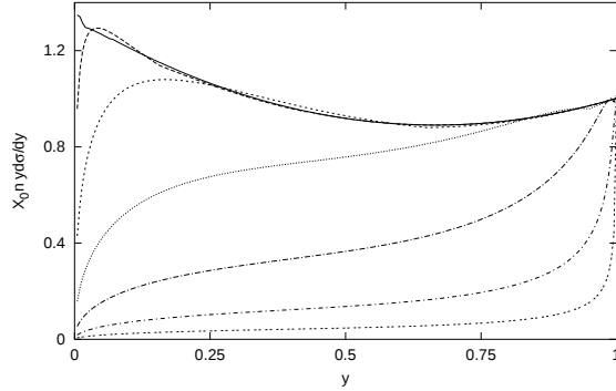
Figure 1. The energy weighted differential cross section per radiation length for bremsstrahlung in water as a function of y = k/E for electrons with energies of 640 GeV (top curve), 6.4 TeV, 64 TeV, 640 TeV, 6.4 PeV, 64 PeV and 640 PeV (bottom curve). These curves apply for other materials for electron energies of 0.0023, 0.023, 0.23, 2.3, 23, 230 and 2300 times E_{LPM} .
