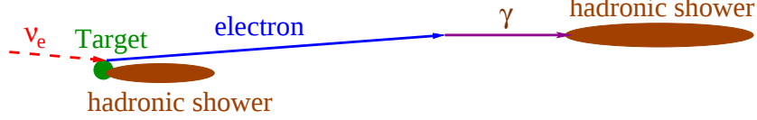
Figure 6. Diagram of UHE \nu_e shower development with photonuclear interactions (not to scale).
