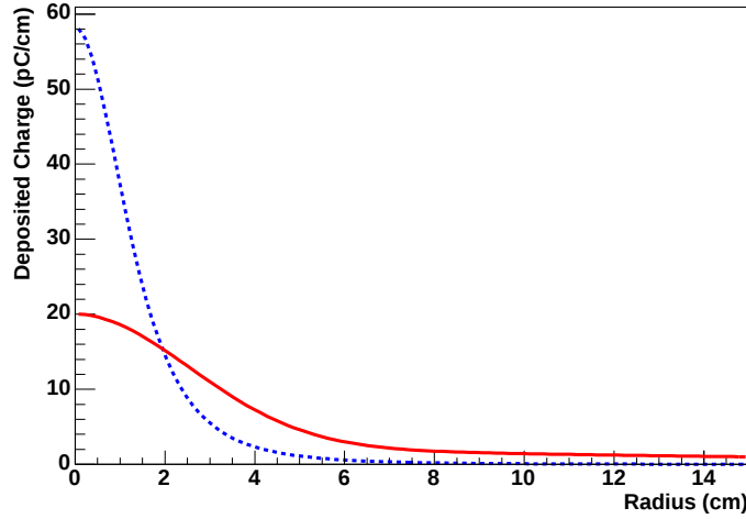
Figure 8. Lateral profiles of charge deposition dQ/dR for 150 GeV electromagnetic (dashed line) and hadronic (solid line) showers as observed by the LAA project.
