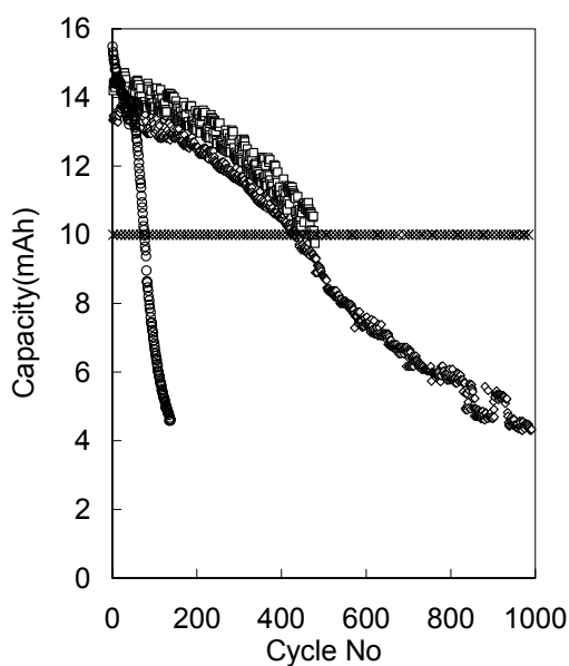
Figure 1. Discharge capacity of 12 cm 2 LiNi 0.8 Co 0.15 Al 0.05 O 2 /Mag-10 pouch cells: 100%DOD: ◇ PG03, PG04, 70%DOD: × PG06, and 100%DOD at 60°C: ○ PG13
