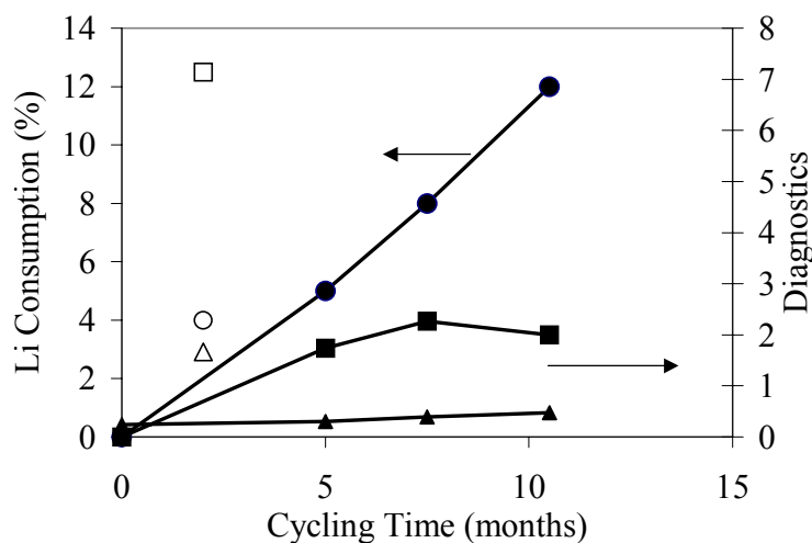
Figure 3. Diagnostic parameters shown as a function of time, room temperature cells (closed symbols) and 60°C cell (open symbols): Li consumption calculated as shown in Fig. 2 (●, ○); I/O ratio from FTIR data (■, □), D/G ratio from Raman data (▲, △).
