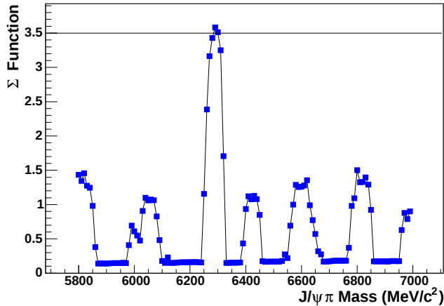
FIG. 2: The \Sigma function at different values of the invariant mass corresponding to the nominal mass peak position.
