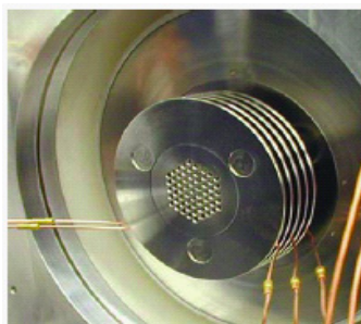
Multiple beamlet-Einzel lens array w/high gradient insulators
