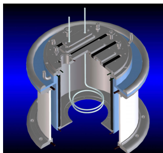
Figure 1: Source Test Stand (STS-100): Sixty-one beamlets have been extracted from an RF-argon plasma source, through a grid supported by three multi-layer high gradient insulator stacks (not visible), with brightness and uniformity meeting requirements for heavy ion fusion.
