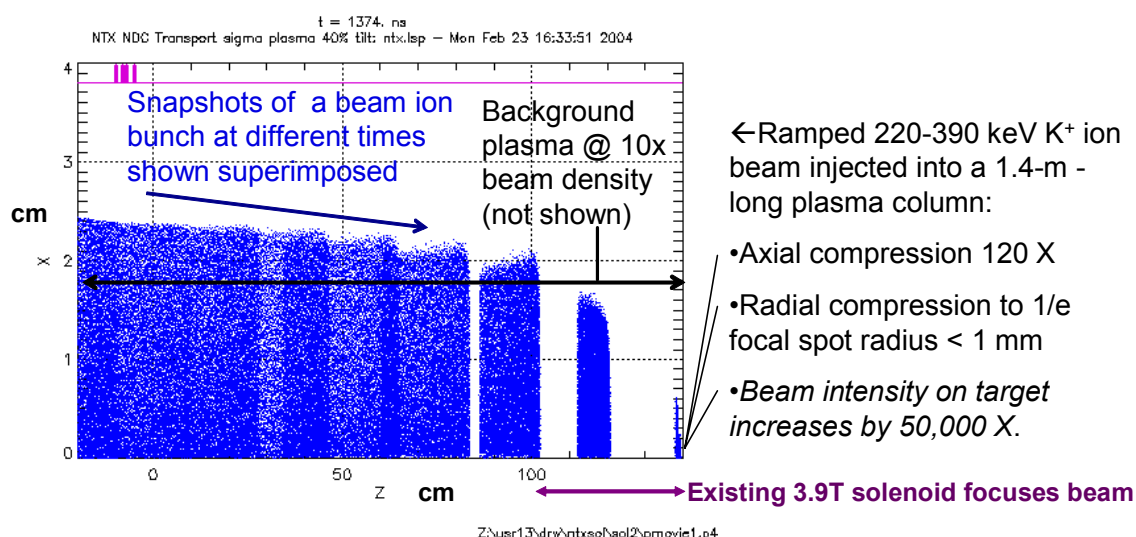
Figure 5: Particle-in-cell simulation of a possible experiment using NTX equipment to study longitudinal compression and radial focusing of an intense heavy ion beam within a neutralizing background plasma column. The peak beam current density exceeds 100 \text{ A/cm}^2 on axis.
