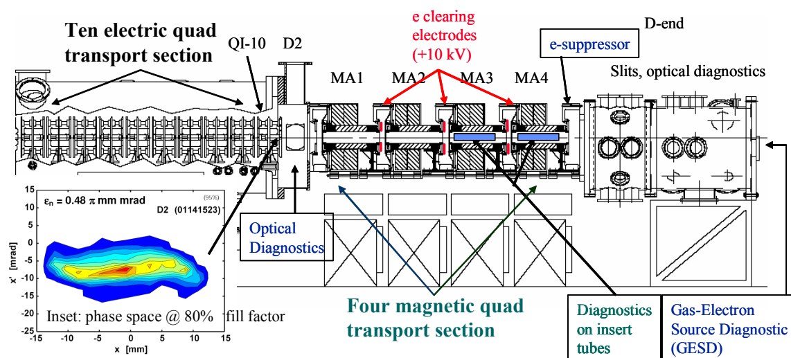
Figure 3: The High Current Experiment (HCX), showing the 5-lattice period electrostatic transport section and the new four magnetic quadrupole transport section and diagnostic locations where gas and electron cloud experiments are conducted. The inset shows a horizontal phase-space diagram following the HCX electrostatic transport section where the beam filled 80% of the aperture (maximum excursion of the beam envelope). The coherent envelope expansion of the beam has been removed so that any phase-space distortions are clearly visible. The mismatch amplitude in the upstream transport channel was 1 \pm 0.5 mm.
