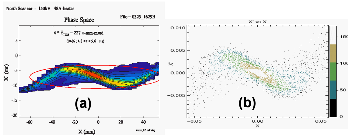
Figure 2 (a) Experimental phase space measured for an unapertured beam created with a 10-cm diameter alumino-silicate surface ionization source. (b) Warp-3-D particle-in-cell simulation of the experiment depicted in (a).
