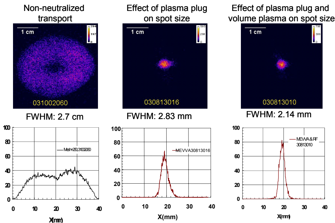
Figure 4. The Neutralized Transport Experiment (NTX) showing beam images at the focal plane for three cases of space-charge neutralization for a high perveance ( 6 \times 10^{-4} ), 25 mA, 300 keV K^+ ion beam: left: no preformed plasma; center: localized “plug” plasma just beyond the last focusing magnet, and right: with both “plug” and “volume” preformed plasma.
