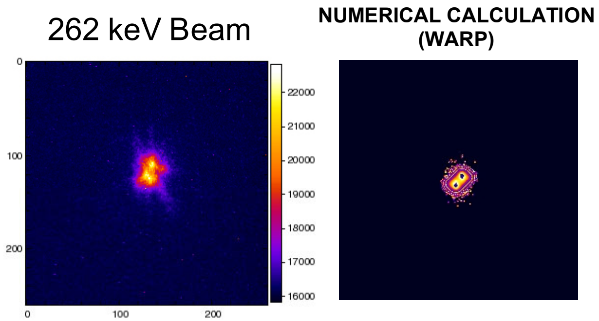
Figure 15: Analog (pinhole) simulation and WARP3D calculation of fully neutralized beam focused to a small spot. Image box size is 4cm b×4 cm squares.
