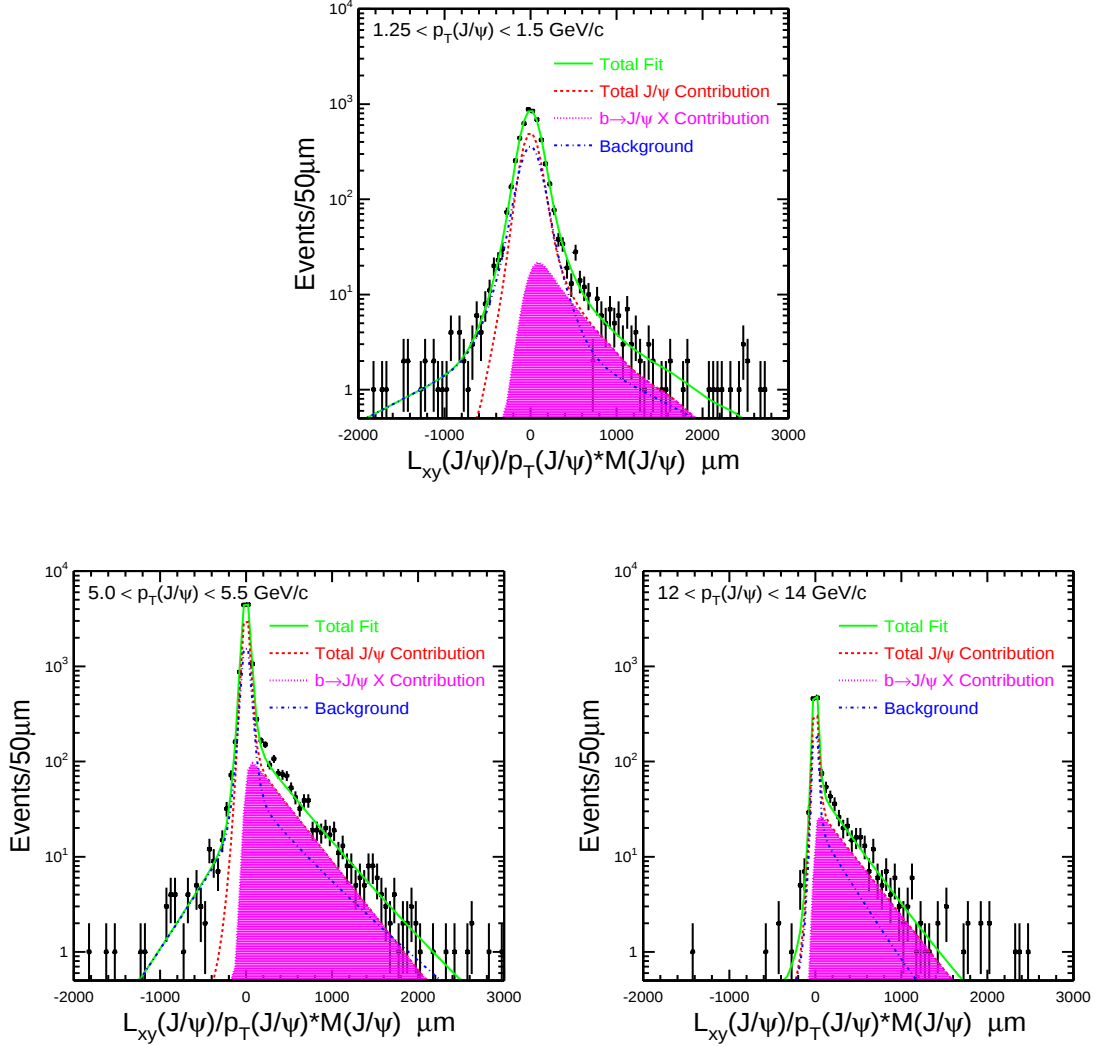
FIG. 7: Fits to the J/\psi pseudo-proper decay time in the ranges of 1.25 < p_T(\mu\mu) < 1.5 \text{ GeV}/c (top), 5.0 < p_T(\mu\mu) < 5.5 \text{ GeV}/c (bottom left) and 12.0 < p_T(\mu\mu) < 14.0 \text{ GeV}/c (bottom right). The solid line is the fit to all the events in the mass window of 2.85 to 3.35 \text{ GeV}/c^2 , the dashed line is the fit to all signal events, the solid histogram is the fit to the portion of the signal events that are from b -hadron decays and the dot-dashed line is the fit to background events including events in the invariant mass sidebands.
