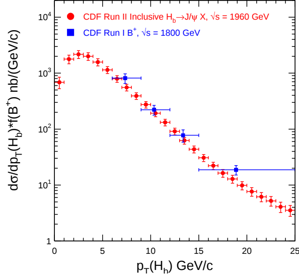
FIG. 13: The differential cross-section distributions of b -hadrons as a function of b -hadron momentum from the measurement of the B^+ meson cross section in CDF Run I [9] and b -hadron inclusive cross section extracted in this analysis (Run II). The differential cross sections showed are integrated over the rapidity range |y(H_b)| < 1.0 .
