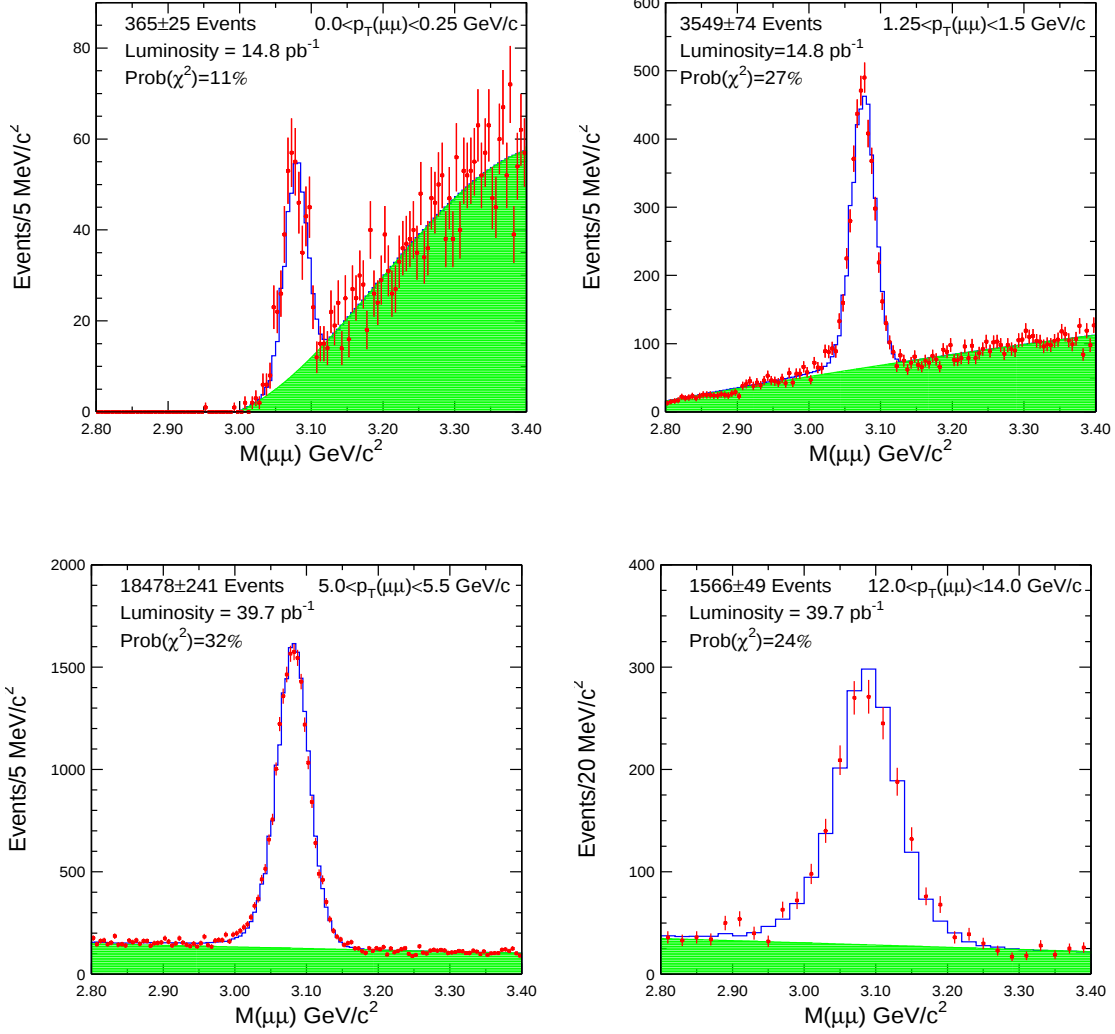
FIG. 2: Invariant mass distributions of reconstructed J/\psi \rightarrow \mu\mu events in the ranges of p_T(\mu\mu) < 0.25 \text{ GeV}/c (top left), 1.25 < p_T(\mu\mu) < 1.5 \text{ GeV}/c (top right), 5.0 < p_T(\mu\mu) < 5.5 \text{ GeV}/c (bottom left) and 12.0 < p_T(\mu\mu) < 14.0 \text{ GeV}/c (bottom right). The points with error bars are data. The solid line is the fit to the signal shape from the simulation and a polynomial shape for the background. The shaded histogram is the fitted background shape. The number of signal events and the fit probability of the binned \chi^2 fitting are also provided.
