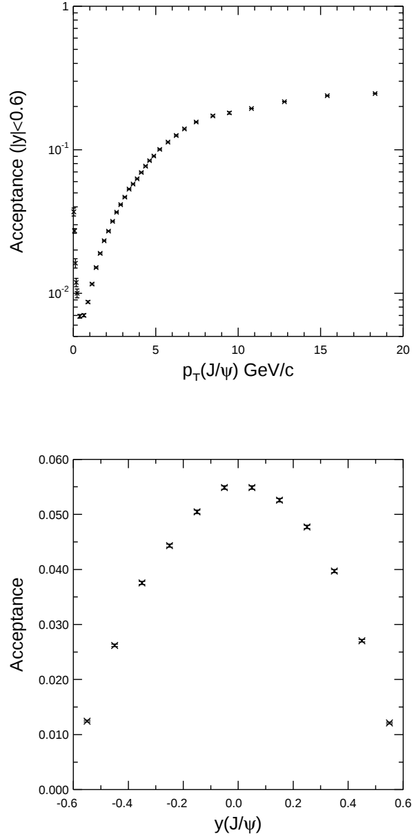
FIG. 3: Acceptance of J/\psi \rightarrow \mu\mu events determined from a GEANT simulation of the CDF detector. The acceptance is shown as a function of p_T(J/\psi) and y(J/\psi) . The acceptance as a function of p_T(J/\psi) is measured integrated over |y| < 0.6 and the acceptance as a function of y is shown integrated over all p_T .
