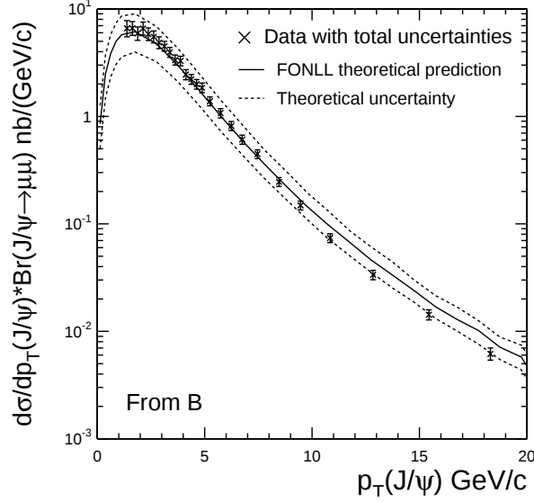
FIG. 9: Differential cross-section distribution of J/\psi events from the decays of b -hadrons as a function of J/\psi transverse momentum integrated over the rapidity range |y| < 0.6 . The crosses with error bars are the data with systematic and statistical uncertainties added including correlated uncertainties. The solid line is the central theoretical values using the FONLL calculations outlined in [42], the dashed line is the theoretical uncertainty.
