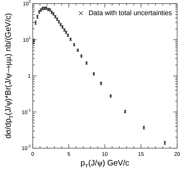
FIG. 5: Inclusive J/\psi cross section, d\sigma/dp_T \cdot Br(J/\psi \rightarrow \mu\mu) , as a function of J/\psi p_T integrated over the rapidity range |y| < 0.6 . The differential cross section with systematic and statistical uncertainties added is plotted. This includes correlated uncertainties.
