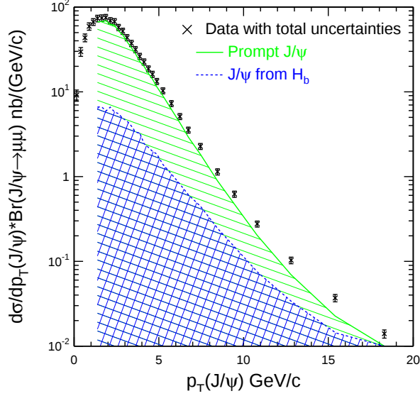
FIG. 10: The inclusive J/\psi cross section as a function of J/\psi p_T integrated over the rapidity range |y| < 0.6 is plotted as points with error bars where all uncertainties have been added. The hatched histogram indicates the contribution to the cross section from prompt charmonium production. The cross-hatched histogram is the contribution from decays of b -hadrons.
