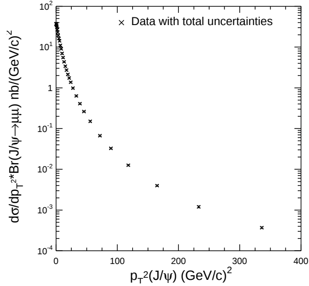
FIG. 6: The invariant J/\psi cross section, d\sigma/dp_T^2 \cdot Br(J/\psi \rightarrow \mu\mu) , as a function of p_T^2(J/\psi) . The differential cross section is plotted. This includes correlated uncertainties.
