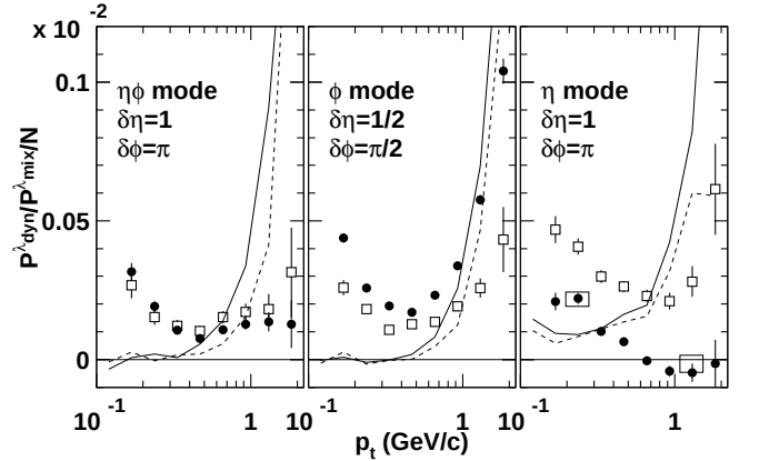
FIG. 2: Central events: normalized dynamic texture for fineness scales m = 0, 1, 0 from left to right panels, respectively, as a function of p_t . \bullet – STAR data; solid line – HIJING without jet quenching; dashed line – HIJING with quenching; \square – peripheral STAR data from Fig. 1 renormalized as described in the text. The rectangles around two chosen points show the estimated systematic errors.
