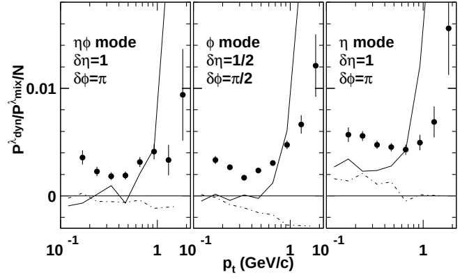
FIG. 1: Peripheral events: normalized dynamic texture for fineness scales m = 0, 1, 0 from left to right panels, respectively, as a function of p_t . \bullet – STAR data; solid line – HIJING without jet quenching; dash-dotted line – HIJING without jets.
