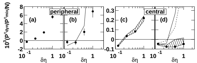
FIG. 3: Scale dependence of the dynamic texture in peripheral and central events. (a,c): 0.2 < p_t < 0.28 , (b,d): 1.1 < p_t < 1.5 GeV/c. • – STAR data; solid line – HIJING without jet quenching; dashed line – HIJING with quenching. A systematic error estimate is shown as a hatched area. Errors on different scales are estimated independently.
