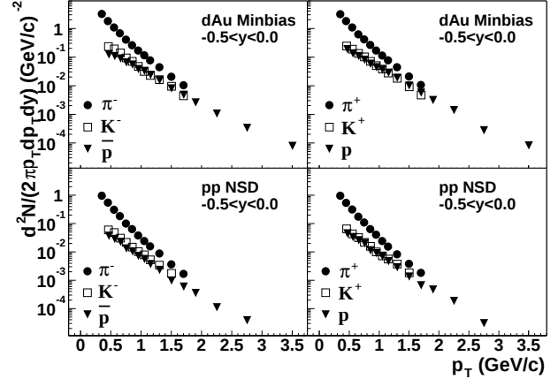
FIG. 2: The invariant yields of pions (filled circles), kaons (open squares), protons (filled triangles) and their anti-particles as a function of p_T from d+Au and NSD p+p events at 200 GeV. The rapidity range was -0.5 < y < 0.0 with the direction of the outgoing Au ions as negative rapidity. Errors are statistical.
