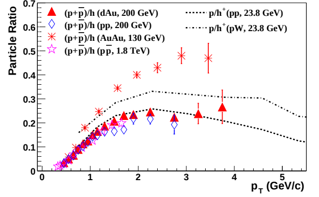
FIG. 4: Minimum-bias ratios of (p + \bar{p}) over charged hadrons at -0.5 < \eta < 0.0 from \sqrt{s_{NN}} = 200 GeV p+p (open diamonds), d+Au (filled triangles) and \sqrt{s_{NN}} = 130 GeV Au+Au [5] (asterisks) collisions. Results of p + \bar{p} collisions at \sqrt{s_{NN}} = 1.8 TeV [27] are shown as open stars. Dashed lines are results of p/h^+ ratios from \sqrt{s_{NN}} = 23.8 GeV p+p (short-dashed lines) and p+W (dot-dashed) collisions [12]. Errors are statistical.
