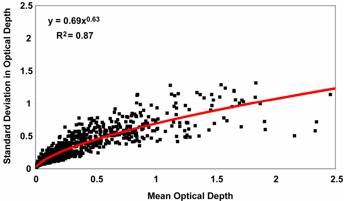
Figure 1. Lamont, OK raman lidar observations of cirrus optical depth variability. A power law relates the observed mean optical depth and standard deviation in optical depth.
