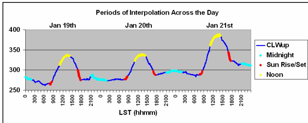
Figure 2. Example of calculated clear-sky LWup (blue) for three days from the Atmospheric Radiation Measurement (ARM) SGP site in January 2004 showing the interpolation periods of local midnight (light blue), sunrise/sunset (red), and local noon (yellow).
