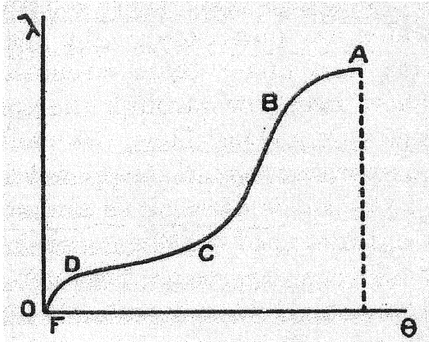
Figure 2: Schematic variation of capillary conductivity \lambda with water content \theta (Buckingham, 1907, Figure 14).
