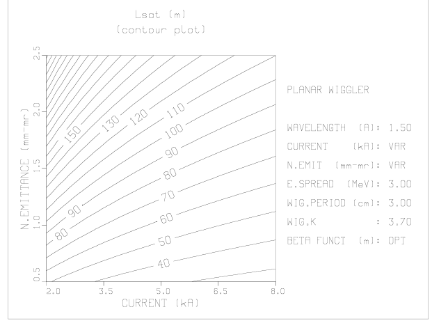
Figure 2. L_{sat} vs. I and \varepsilon_n for the hybrid wiggler with g = 0.6 cm.
