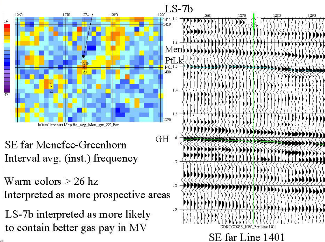
Figure 11 Detail of frequency analysis in Figure 9 for data at potential well site LS-7b.
