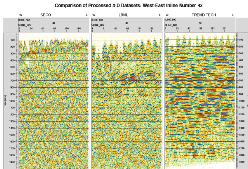
Comparison of processed seismic data along Inline 43 (see Figure 1).
