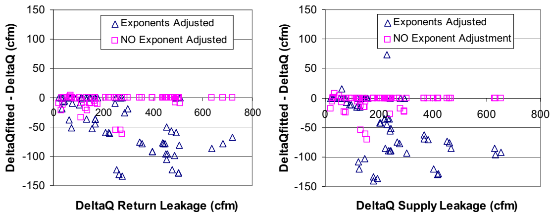
Figure 6. Comparison of DeltaQ Supply and Return Leakage to DeltaQfit with Adjusted Flow Exponents ( l/s = cfm \times 0.47 )
