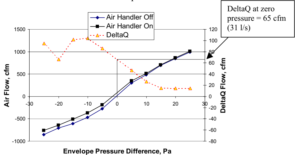
Figure 1. Example DeltaQ Test Results (l/s = cfm \times 0.47)
