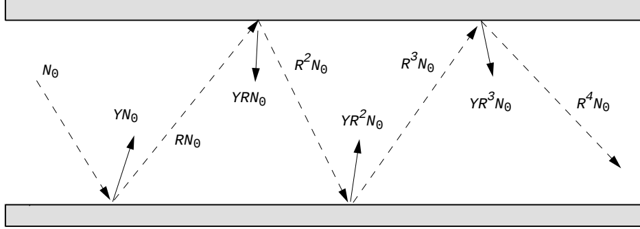
Figure 5: A initial pulse of N_0 photons strikes the wall of a closed vacuum chamber. Upon each bounce, some photoelectrons are generated and some photons are reflected.
