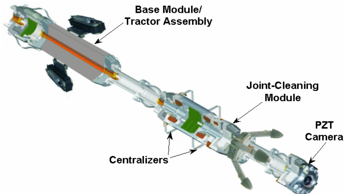
Figure 1. Pipe Wall Preparation Robot Train
