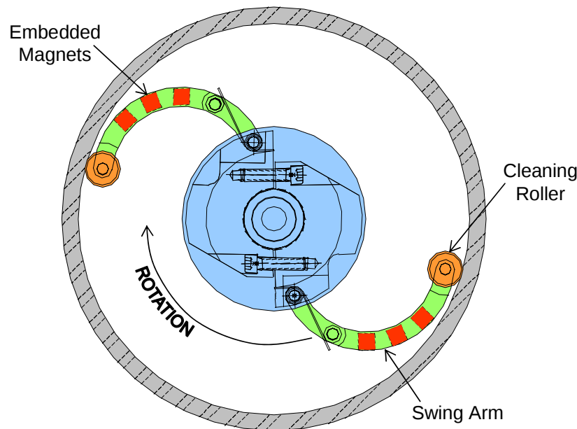
Figure 29. Embedded Magnets to Collect Debris
