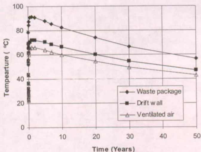
Fig. 1. Temperature histories of the waste package, the drift wall, and the ventilated air at the end of the 600-m emplacement drift [1].
