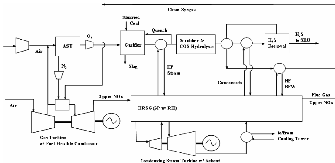
Figure 7. IGCC plant with fuel flexible combustor
