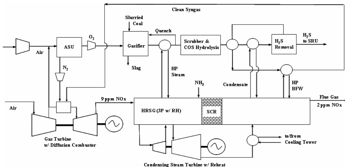
Figure 5. Baseline IGCC plant with diffusion combustor and SCR
