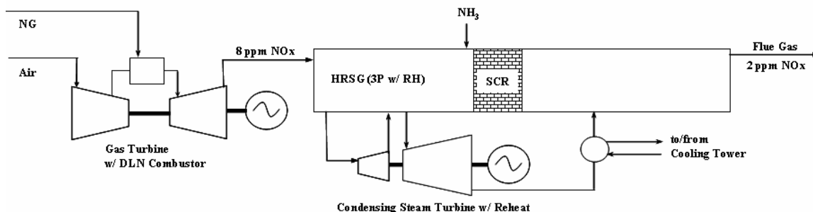
Figure 6. Baseline NGCC plant with DLN combustor and SCR
