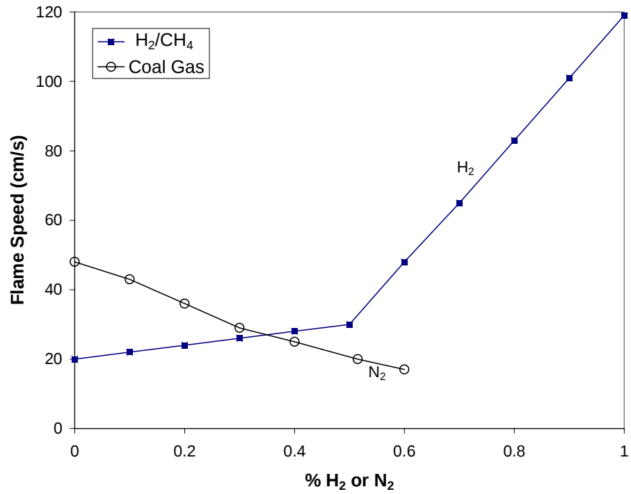
Figure 2. Calculated laminar flame speed versus the volume percent of H 2 in methane or the volume percent N 2 addition to the model coal gas (equivalence ratio = 0.7).
