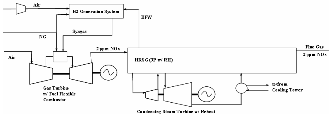
Figure 8. NGCC plant with fuel flexible combustor and CPOX
