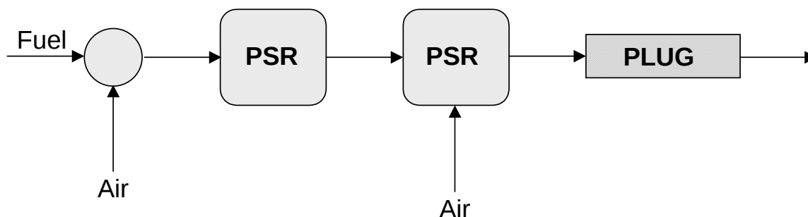
Figure 4. Example of a reactor network model utilized to study gas turbine combustor emissions.
