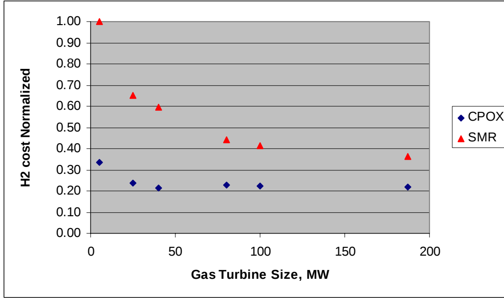
Figure 1. Contained hydrogen unit cost comparison (includes capital and operating cost)
