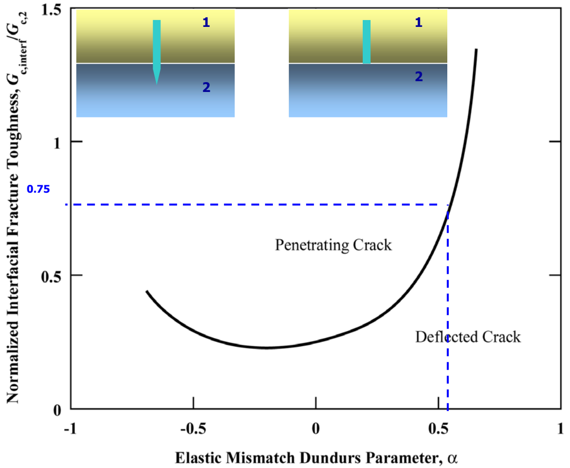
Figure 3. The linear-elastic solutions of He and Hutchinson 22 used to determine the conditions for a normally incident crack to penetrate or deflect along an interface between two materials 1 and 2 . Whether the crack penetrates or not is a function of the (i) impingement angle, (ii) the elastic mismatch across the interface, defined by the first Dundurs' parameter \alpha = (E_1 - E_2) / (E_1 + E_2) , where E_1 and E_2 are the respective elastic moduli for materials 1 and 2 , and E is Young's modulus 29 , and (iii) relative magnitude of the interface toughness and the toughness of material 2 on the far side of the interface, ( G_{c,interf}/G_{c2} ). The figure shows a plot of G_{c,interf}/G_{c2} as a function of the modulus mismatch \alpha . For the enamel/dentin junction where \alpha \sim 0.53 , the absence of interface delamination leads to a criticality between penetration and arrest at the DEJ, which can be used to estimate a lower-bound for the toughness of the DEJ, G_{c,interf} , given by 0.75 of G_{c,interf}/G_{c2} , where G_{c2} is the toughness of the dentin.
