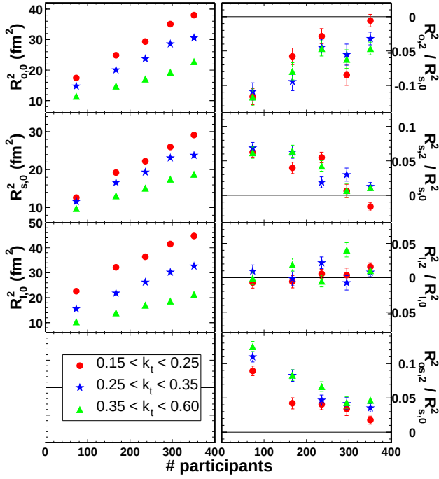
FIG. 3: (color online) Fourier coefficients of azimuthal oscillations of HBT radii vs. number of participating nucleons, for three k_T (GeV/c) bins. Left panels: means ( 0^{\text{th}} -order FC) of oscillations; right panels: relative amplitudes (see text for details). Larger participant numbers correspond to more central collisions.
