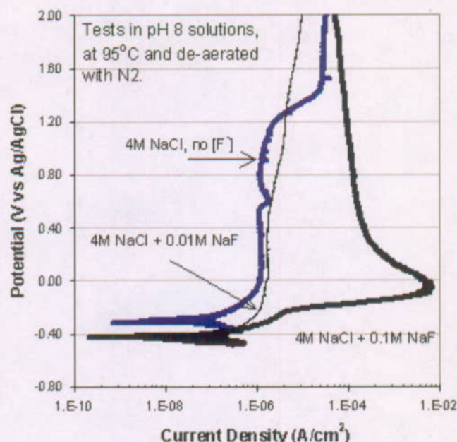
Figure 1. Fluoride Effects at pH 8 on Anodic Polarization Behavior of Titanium Grade 7 in 4 mol/L NaCl Solutions, at 95°C and de-aerated with \text{N}_2
