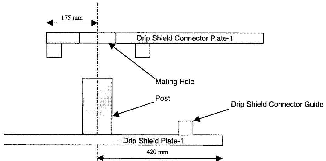
Figure I.1. Geometry for Calculation of Overlap Between Drip Shields
