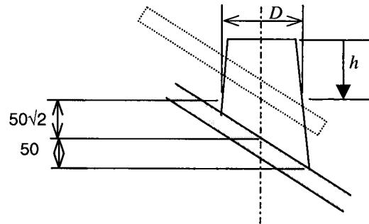
Figure I.3. Definitions of D and h for calculating clearance.
