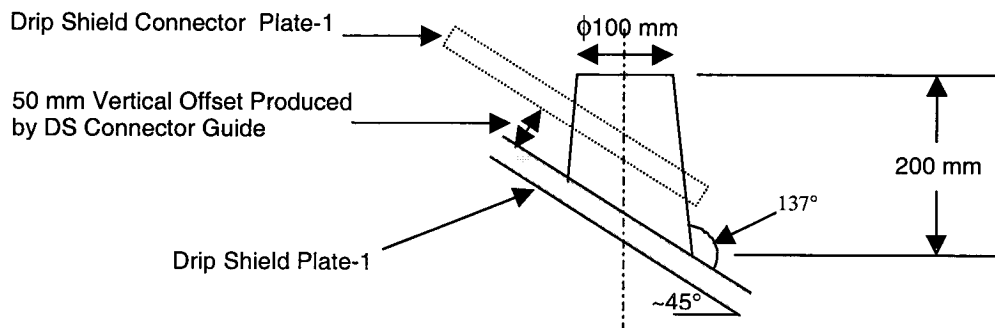
Figure I.2. Schematic (Not to Scale) for Calculation of Clearance Between Post and DS Connector Plate-1
