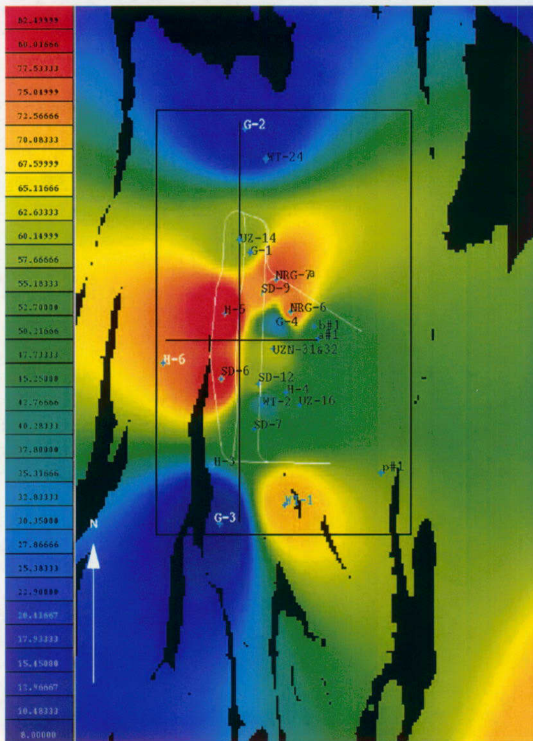
Figure 8. Map View of Volcanic Glass Distribution in "PTn" Unit, Tpcpv1-Tptrv2 (Sequence 20) for Entire MM3.0
