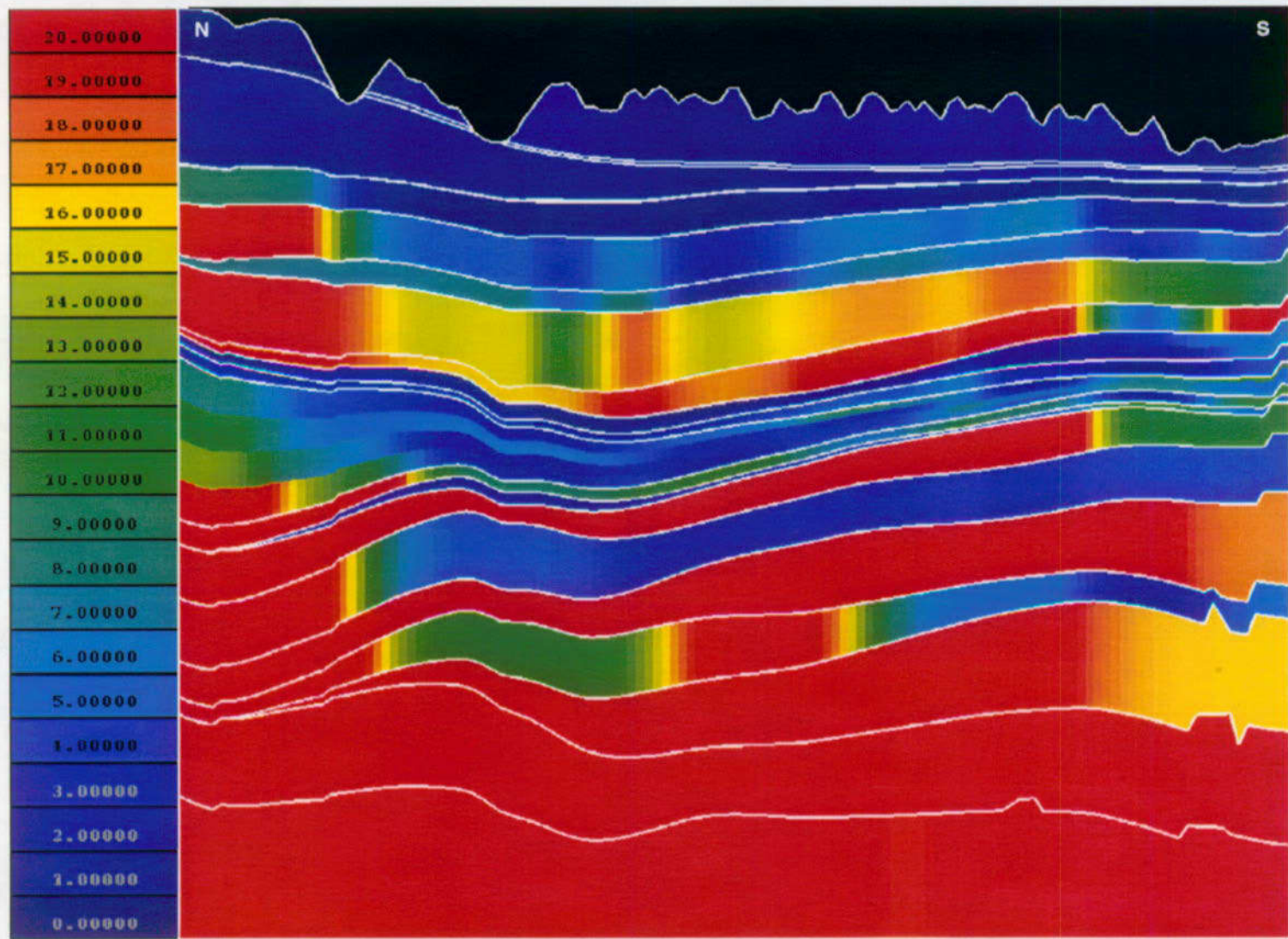
Figure 28. Quartz Distribution in North-South Cross Section Through Potential Repository
