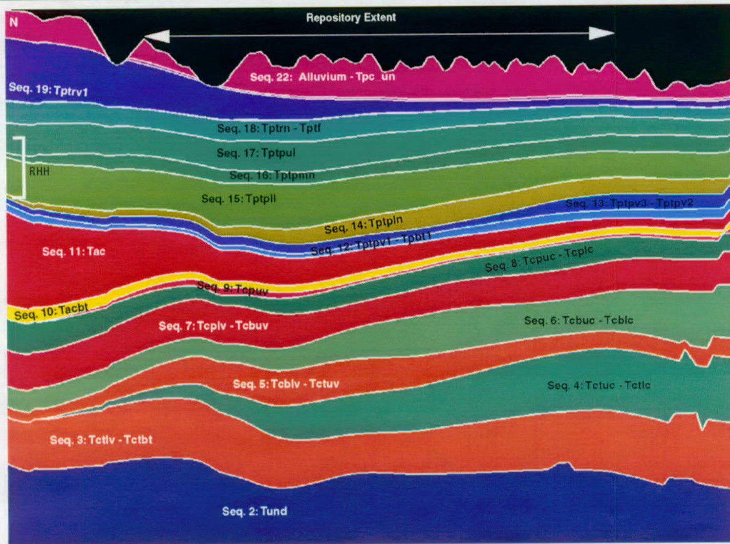
Figure 5. North-South Cross Section Through Potential Repository, Illustrating Sequences Used in MM3.0, Excluding Paleozoic
