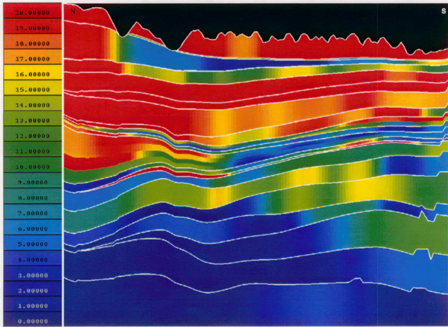
Figure 26. Cristobalite + Opal-CT Distribution in North-South Cross Section Through Potential Repository
