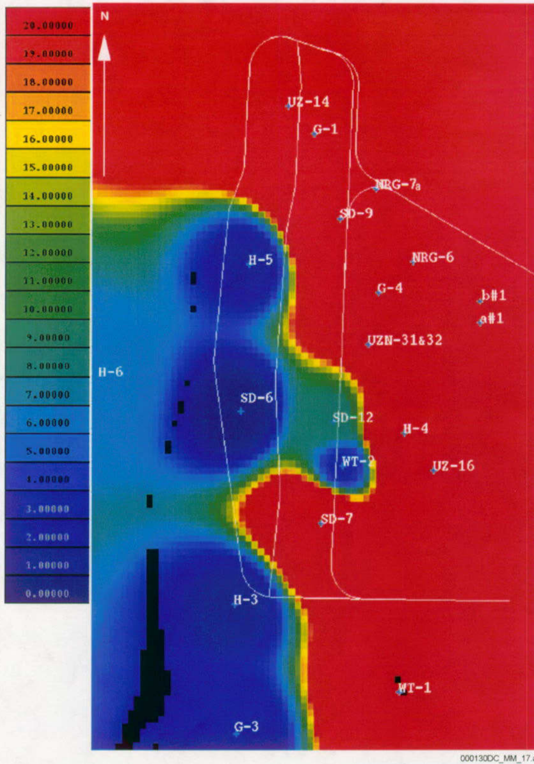
Figure 17. Zeolite Distribution in Map View of Lower Layer (Layer 11) of Calico Hills Formation (Tac, Sequence 11)
