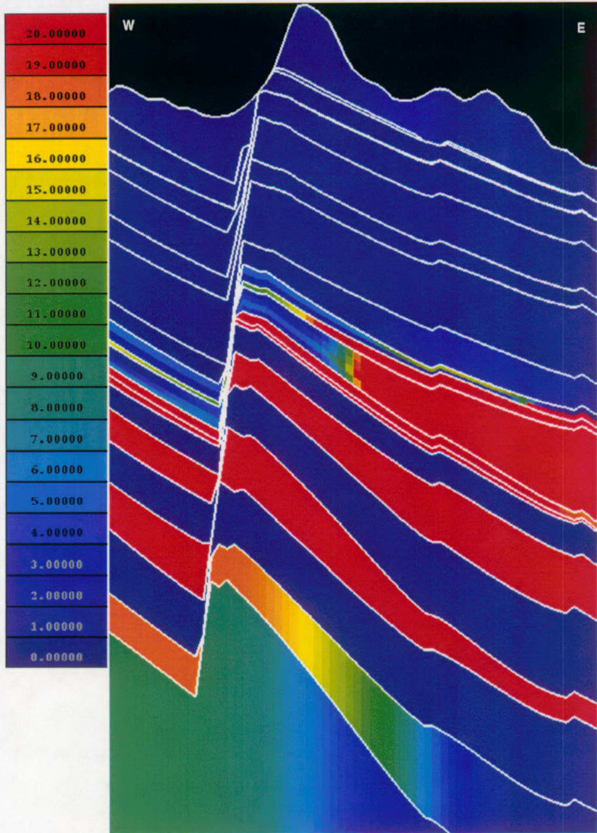
Figure 11. Zeolite Distribution in East-West Cross Section Through Potential Repository Block
