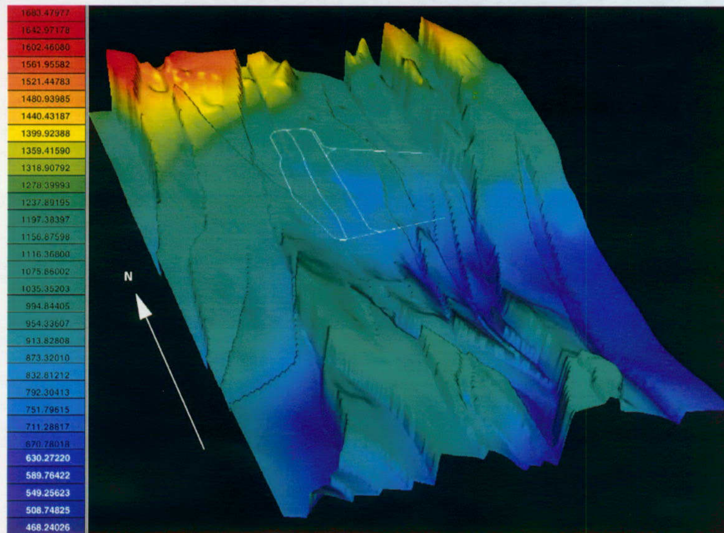
Figure 4. Shaded Relief View of Tpcpv1, Nonwelded Subzone of Vitric Zone of Tiva Canyon Tuff
