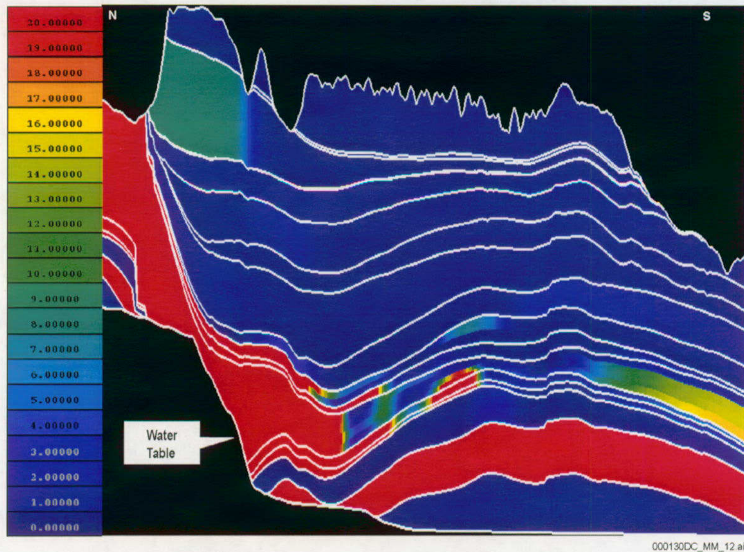
Figure 12. Zeolite Distribution in North-South Cross Section Through Potential Repository Block and Above the Water Table
