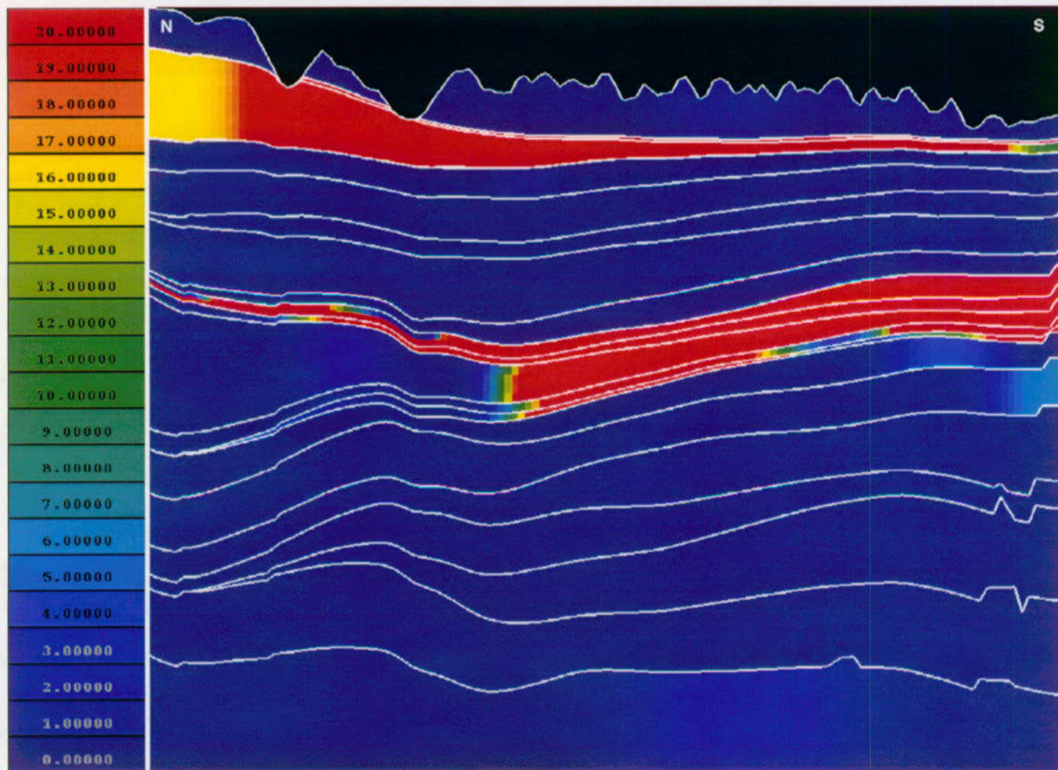
Figure 22. Volcanic Glass Distribution in North-South Cross Section Through Potential Repository
