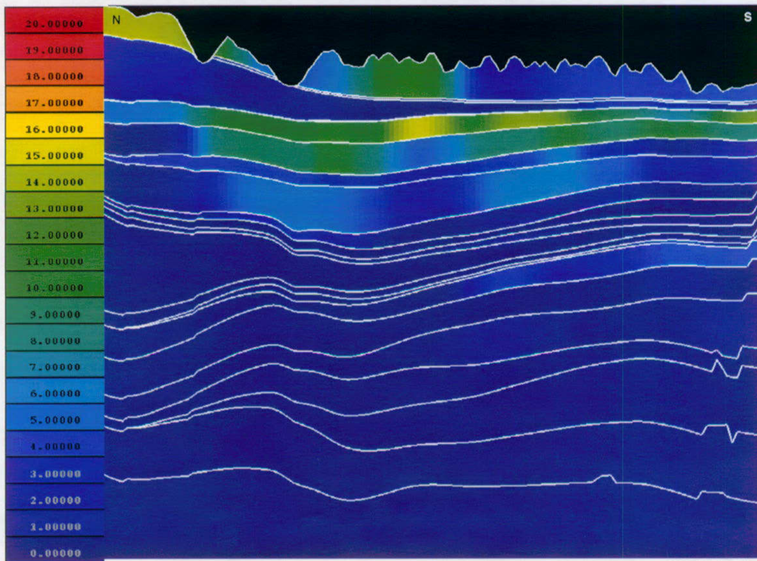
Figure 24. Tridymite Distribution in North-South Cross Section Through Potential Repository
