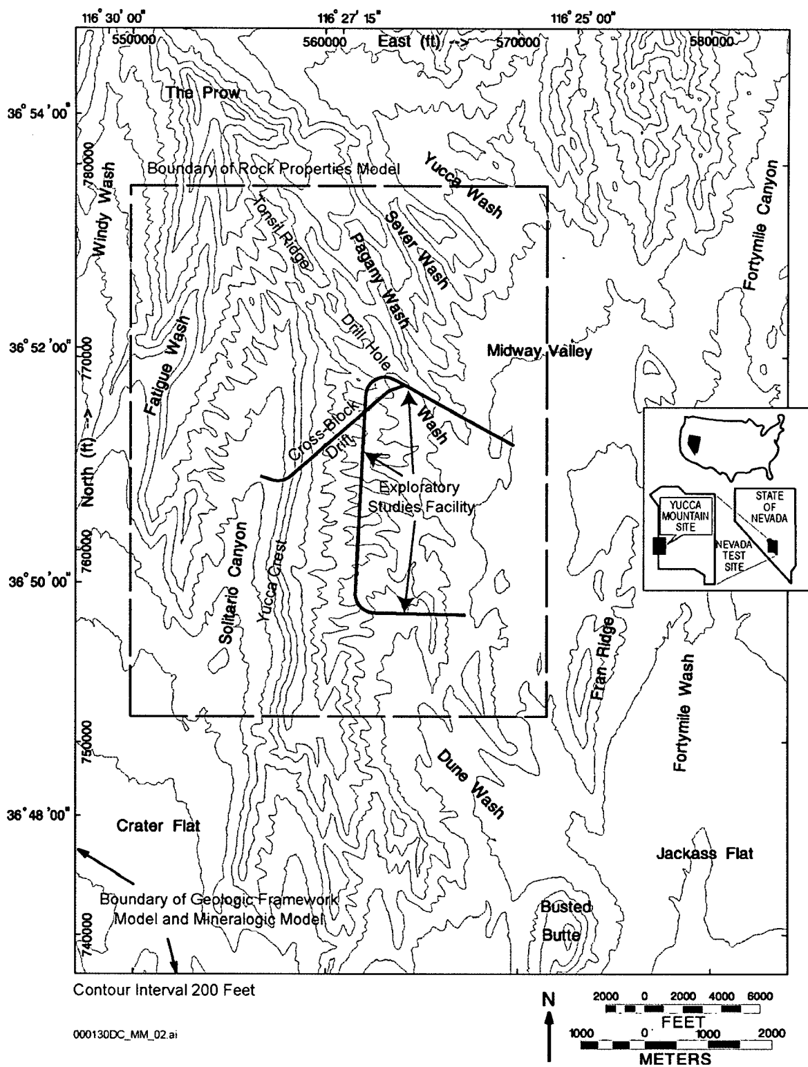
Figure 2. Location Map of Yucca Mountain, Nevada, Showing Location of Exploratory Studies Facility, Cross-Block Drift, and Area of Integrated Site Model with Boundaries of Component Models
