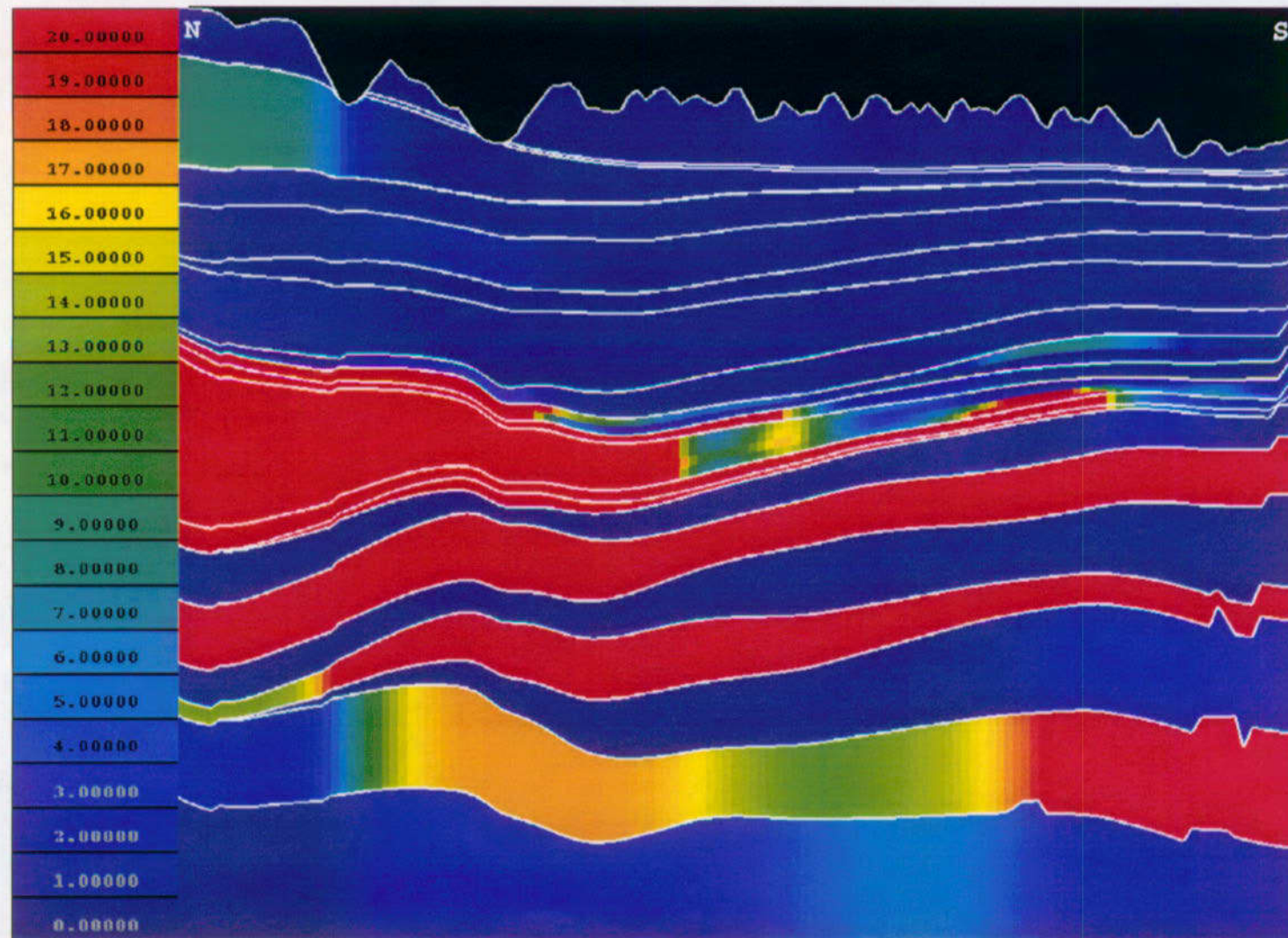
Figure 10. Zeolite Distribution in North-South Cross Section Through Potential Repository Block
