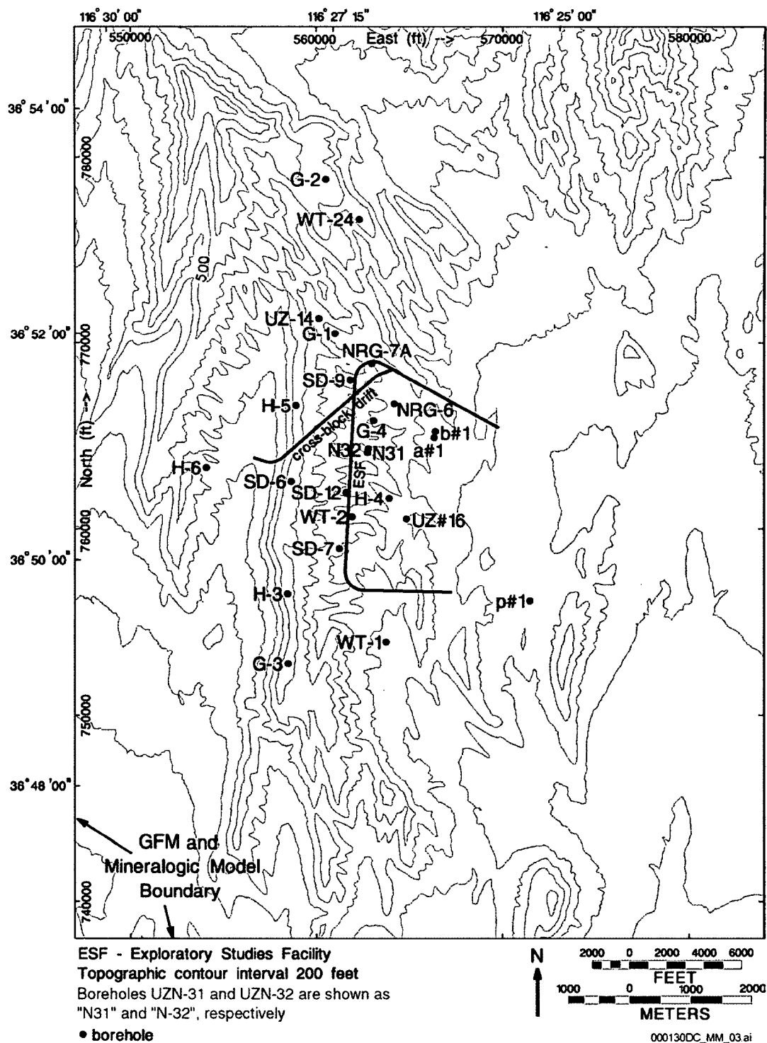
Figure 3. Locations of Boreholes Used in MM3.0
