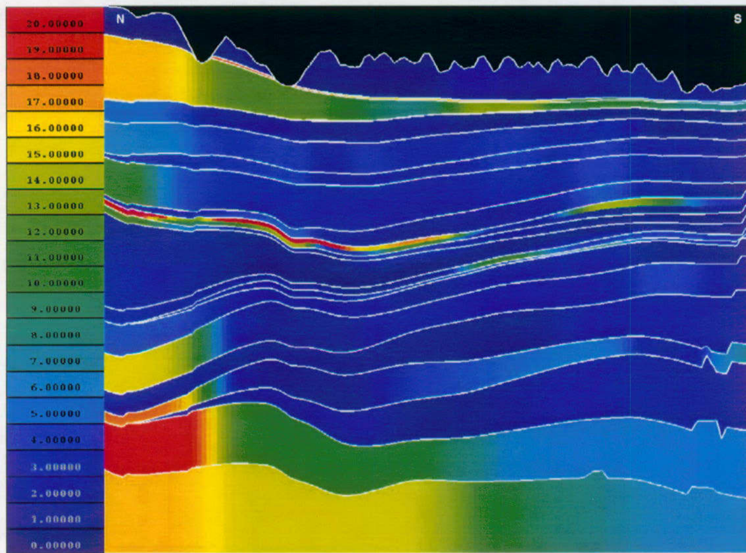
Figure 20. Smectite + Illite Distribution in North-South Cross Section Through Potential Repository
