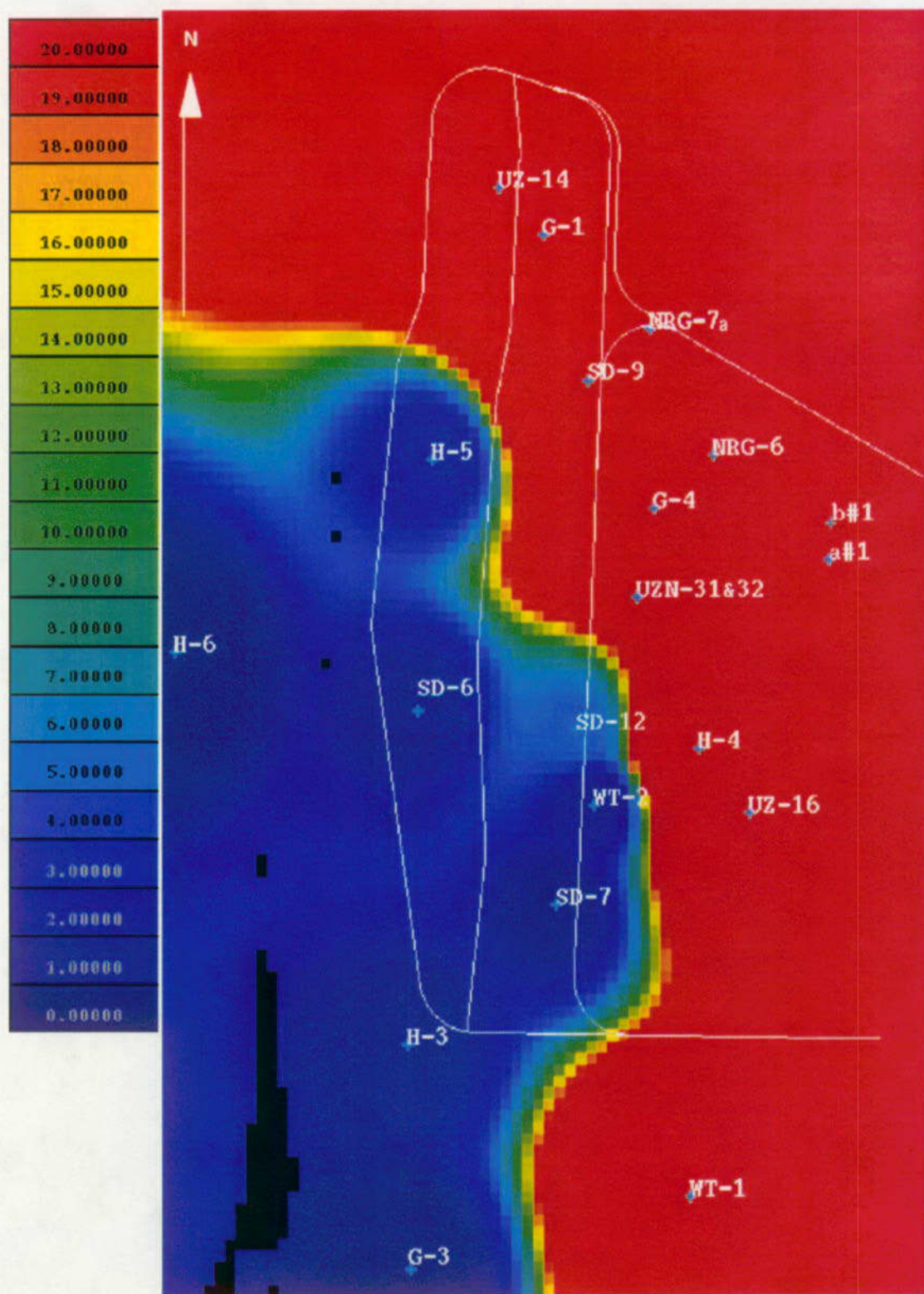
Figure 15. Zeolite Distribution in Map View of Middle-Upper Layer (Layer 13) of Calico Hills Formation | Tac, Sequence 11)
