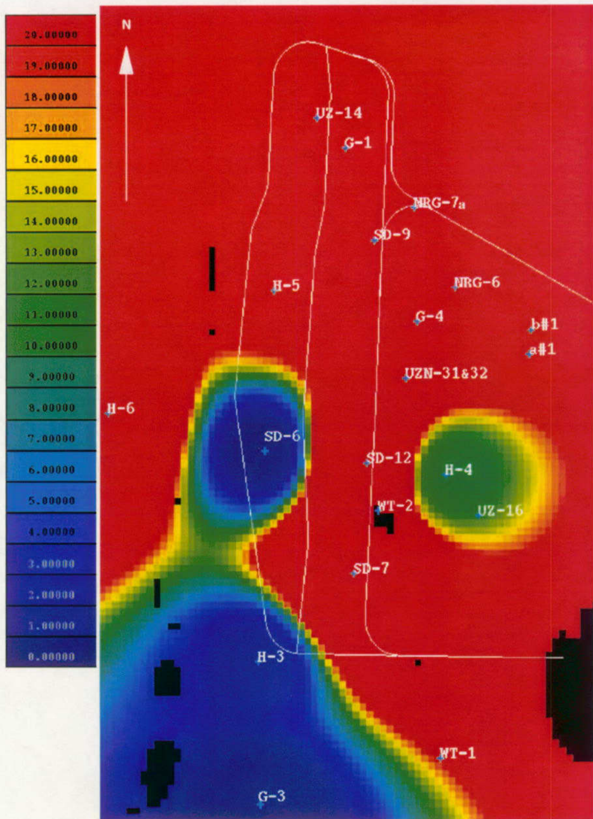
Figure 19. Zeolite Distribution in Map View of Upper Vitric Zone of Prow Pass Tuff (Tcuv, Sequence 9)
