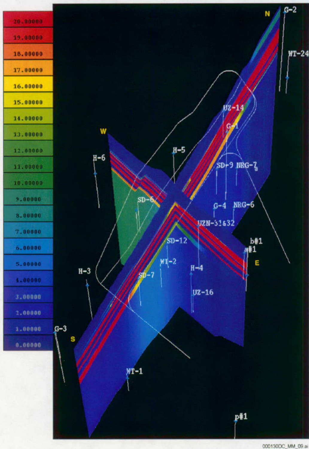
Figure 9. Zeolite Distribution in North-South and East-West Cross Sections Through Center of Potential
