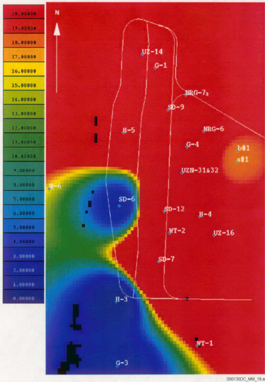
Figure 18. Zeolite Distribution in Map View of Bedded Tuff of Calico Hills Formation (Tacbt, Sequence 10)
