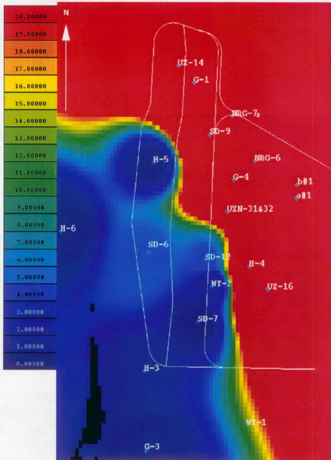
Figure 14. Zeolite Distribution in Map View of Upper Layer (Layer 14) of Calico Hills Formation (Tac, Sequence 11)
