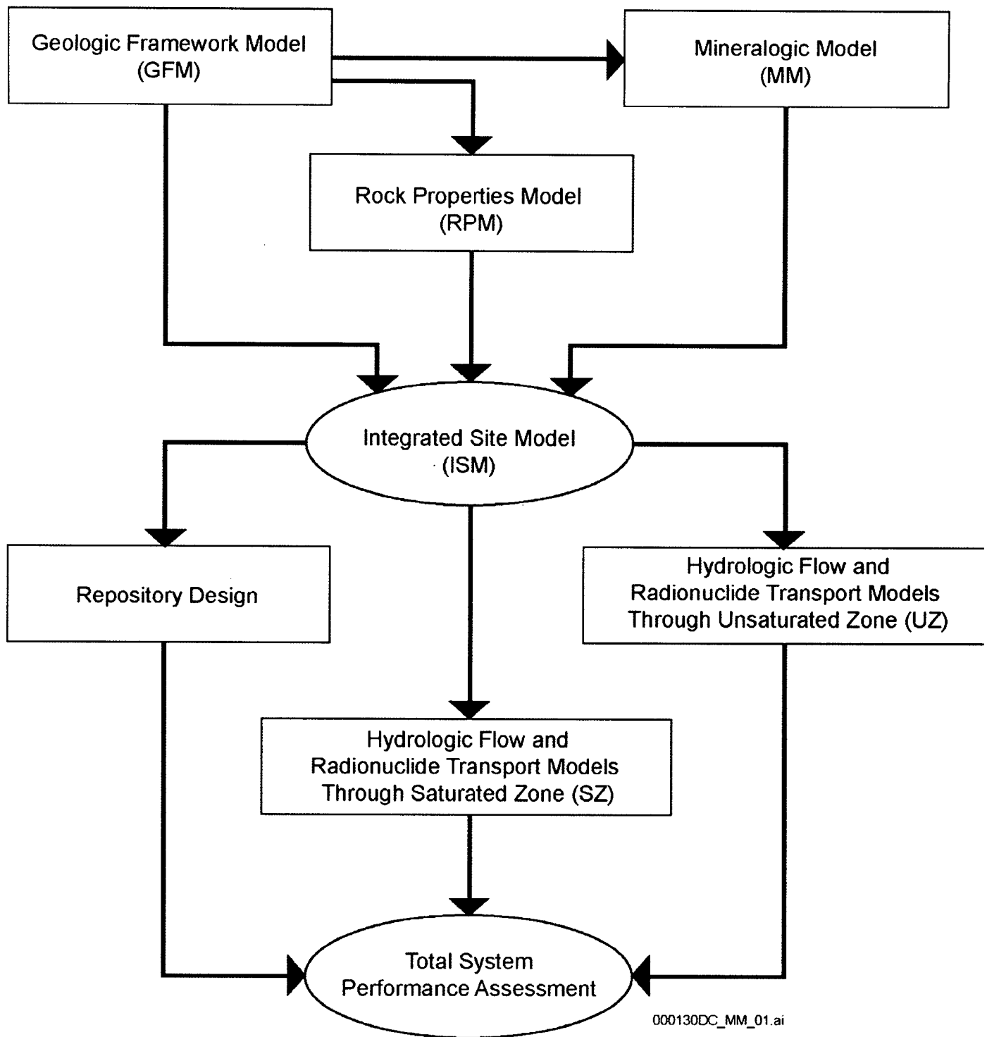
Figure 1. Interrelationships Between Component Models, Integrated Site Model, and Downstream Uses
