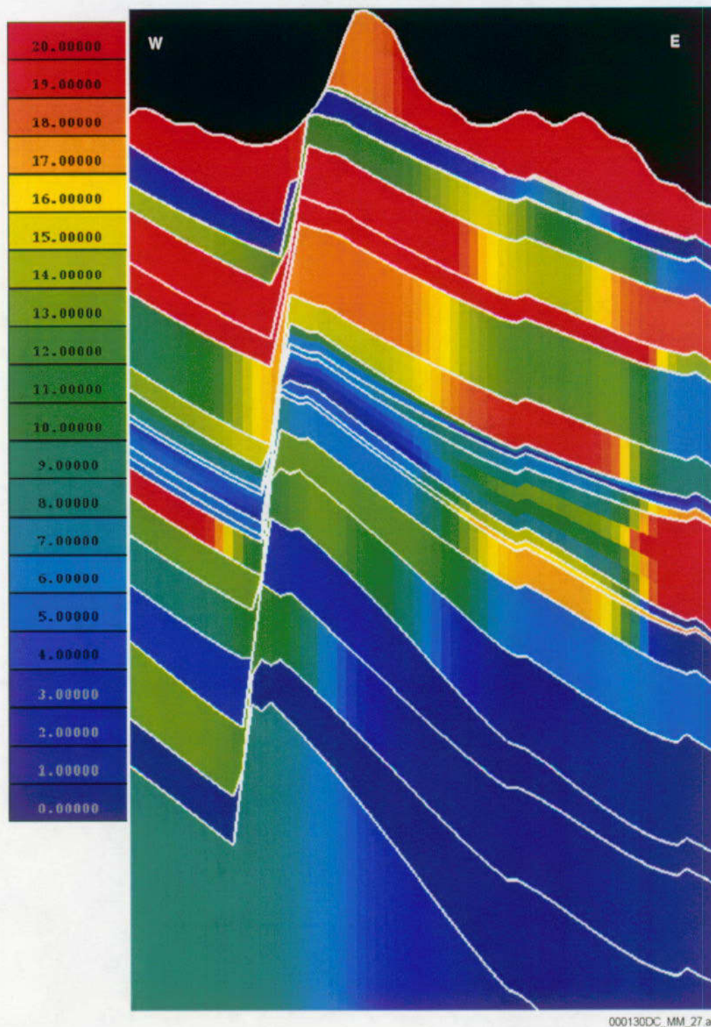
Figure 27. Cristobalite + Opal-CT Distribution in East-West Cross Section Through Potential Repository
