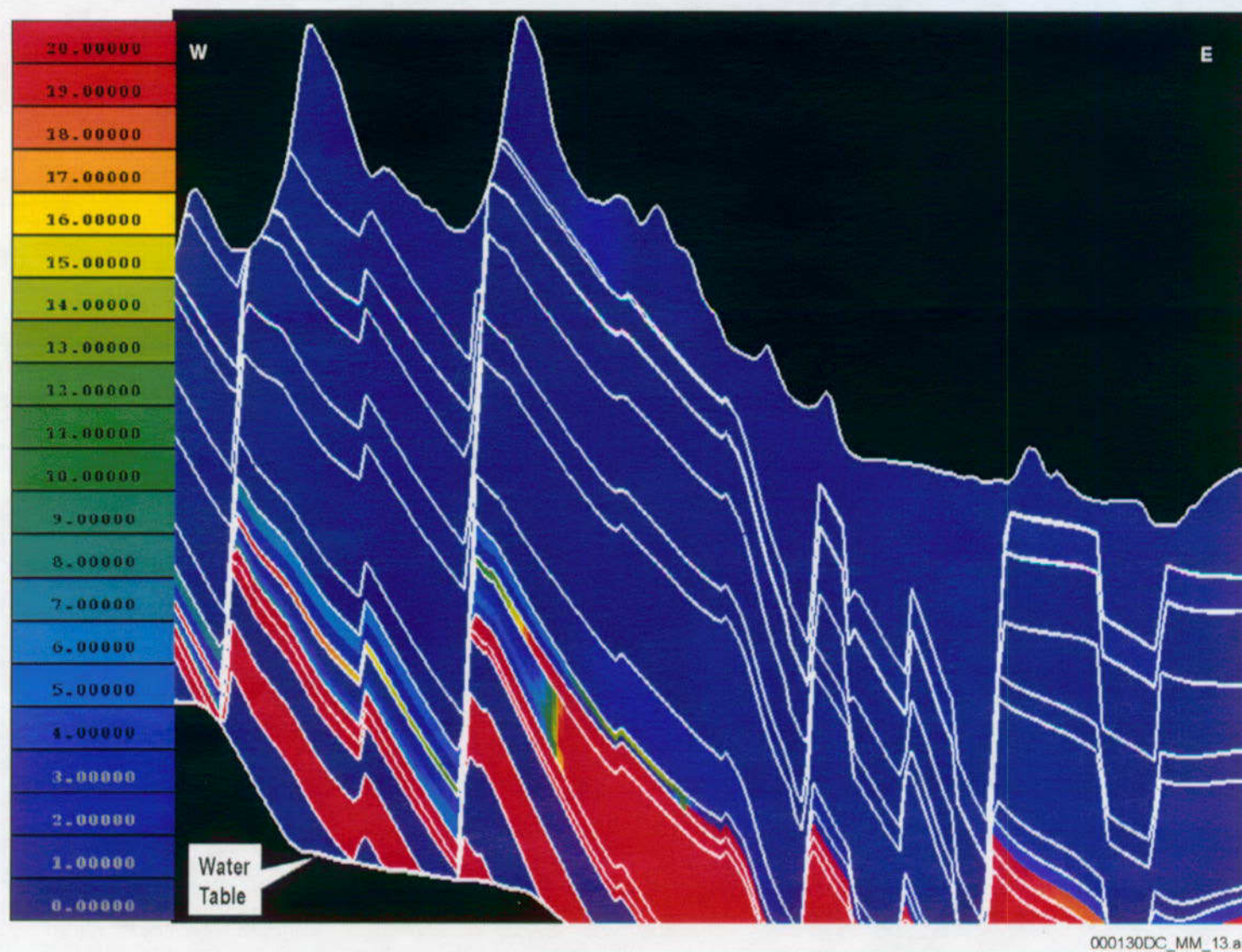
Figure 13. Zeolite Distribution in East-West Cross Section Through Potential Repository Block and Above Water Table
