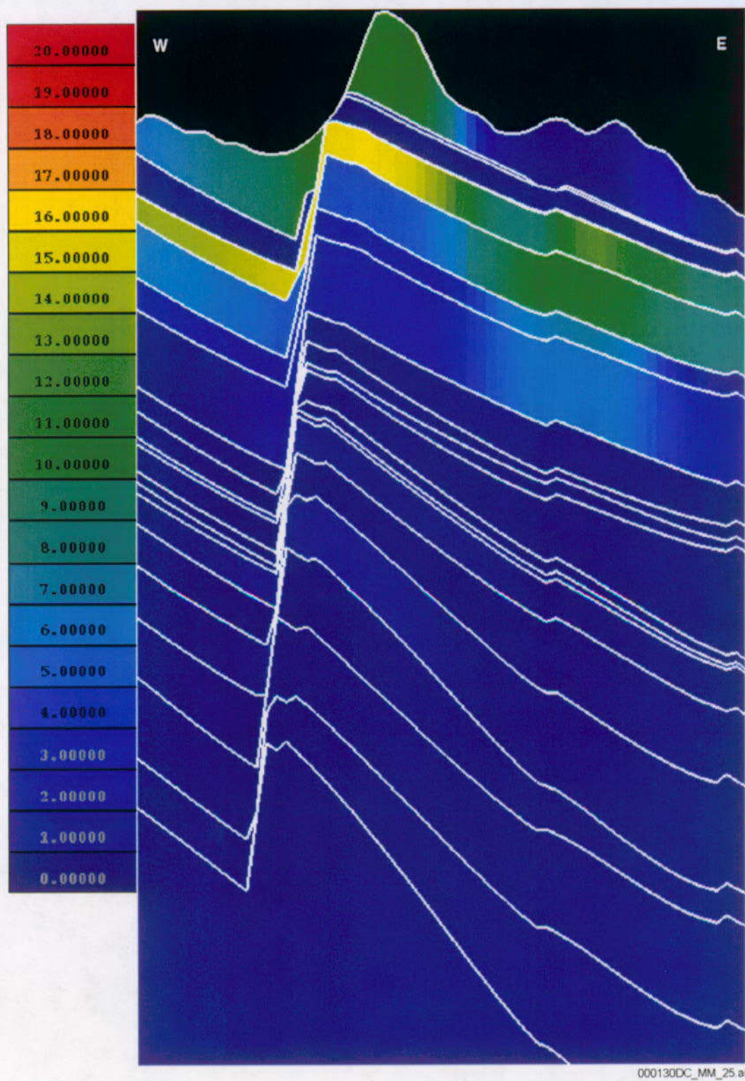
Figure 25. Tridymite Distribution in East-West Cross Section Through Potential Repository
