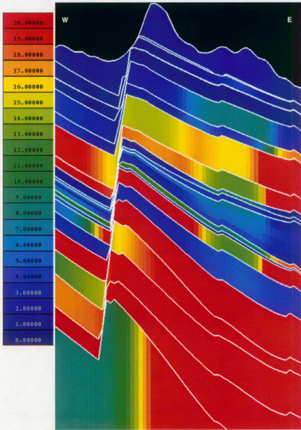
Figure 29. Quartz Distribution in East-West Cross Section Through Potential Repository
