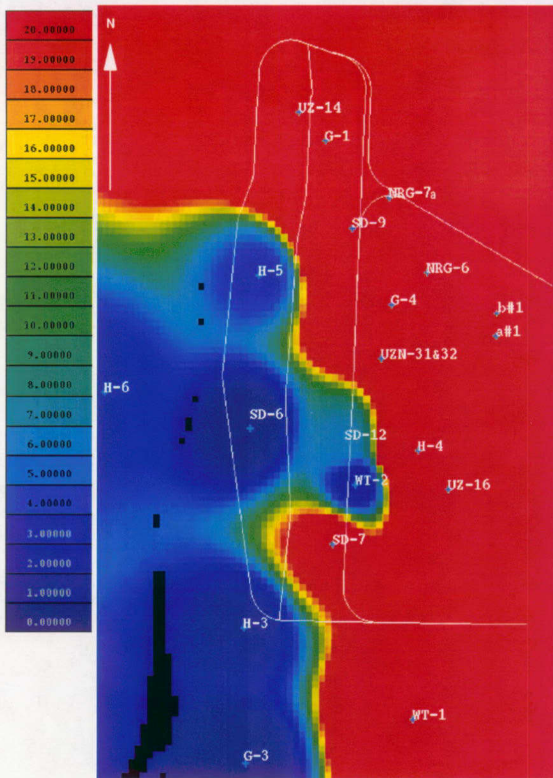
Figure 16. Zeolite Distribution in Map View of Middle-Lower Layer (Layer 12) of Calico Hills Formation (Tac, Sequence 11)
