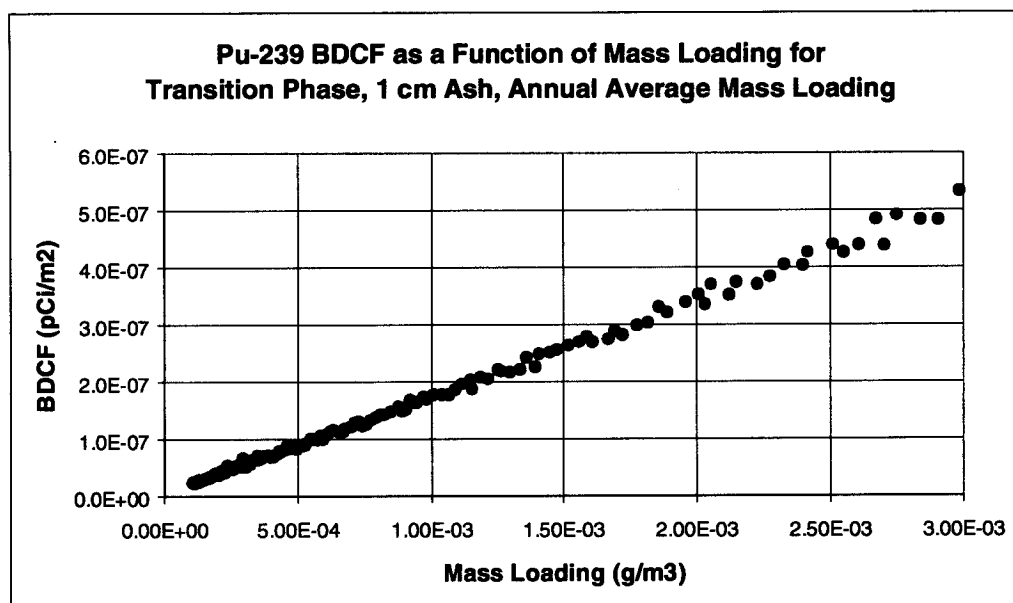
Figure 12. Dependence of BDCF for 239 Pu on Mass Loading for Transition Phase, 1-cm Ash Layer, and Annual Average Mass Loading
