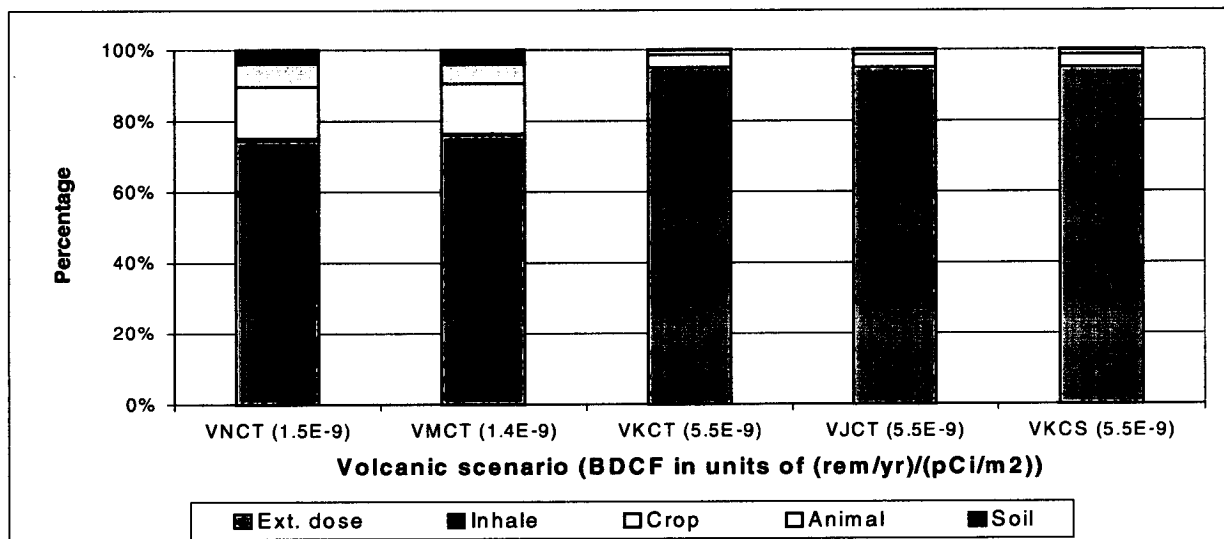
Figure 9. Percentage Pathway Contributions for Volcanic Eruption BDCFs for ^{226}\text{Ra}
