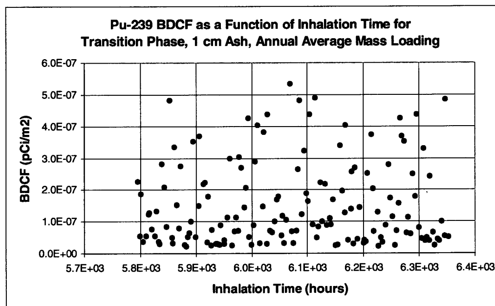
Figure 13. Dependence of BDCF for 239 Pu on Inhalation Time for Transition Phase, 1-cm Ash Layer, and Annual Average Mass Loading
