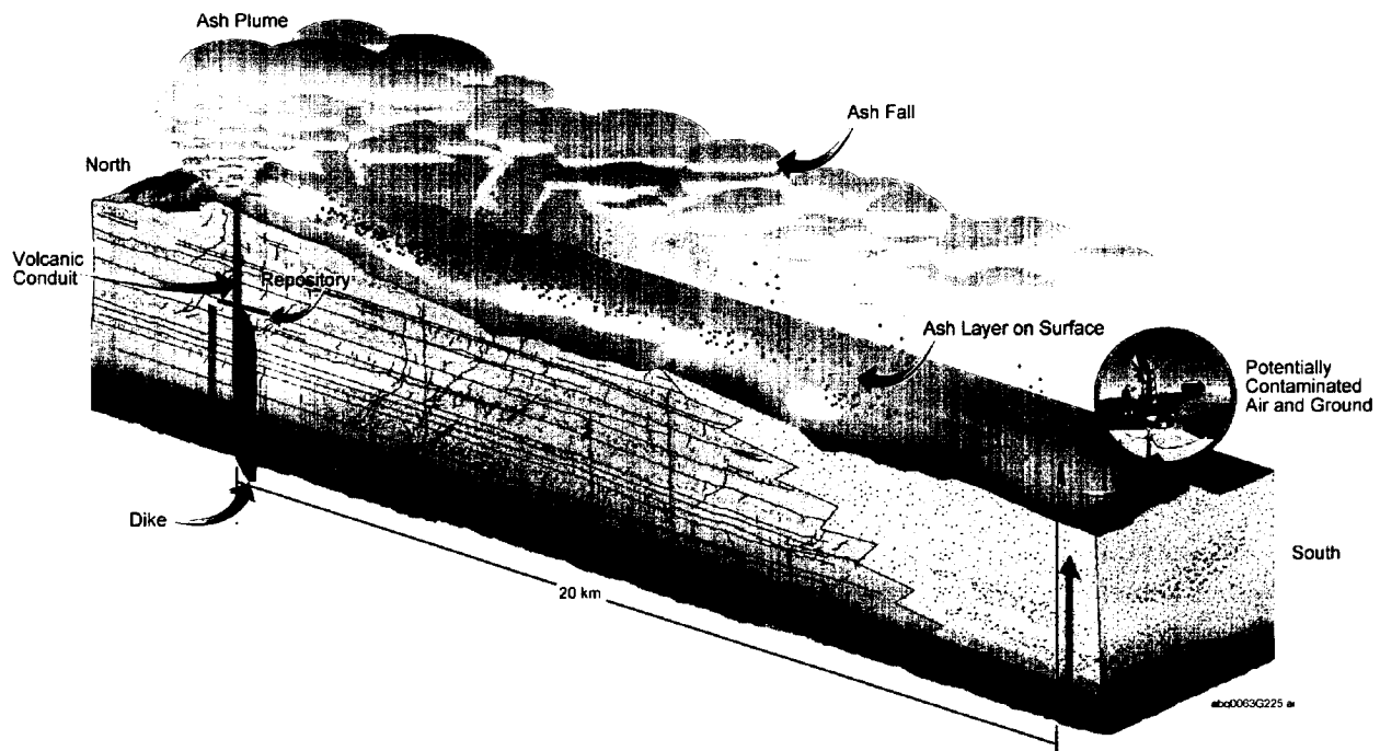
Figure 2. Representation of the Volcanic Eruption Intersecting the Repository
