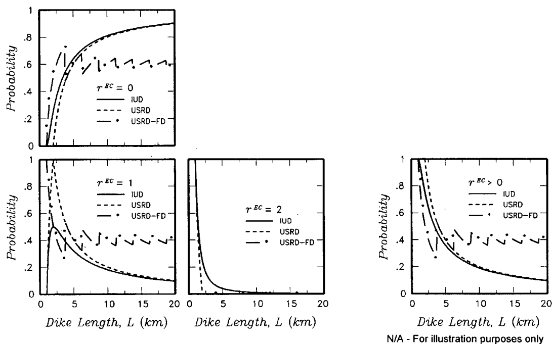
Figure 19. Probability for the Number of Eruptive Centers within the Potential Repository Footprint, r^{EC} , Computed Using the USRD-FD Spatial Distribution of Eruptive Centers and for the Length of Intersection, L^I = 1 Kilometer, and an Average Spacing of 2.5 Kilometers between Eruptive Centers Compared to the Results for the IUD and USRD Models Shown in Figure 15a
